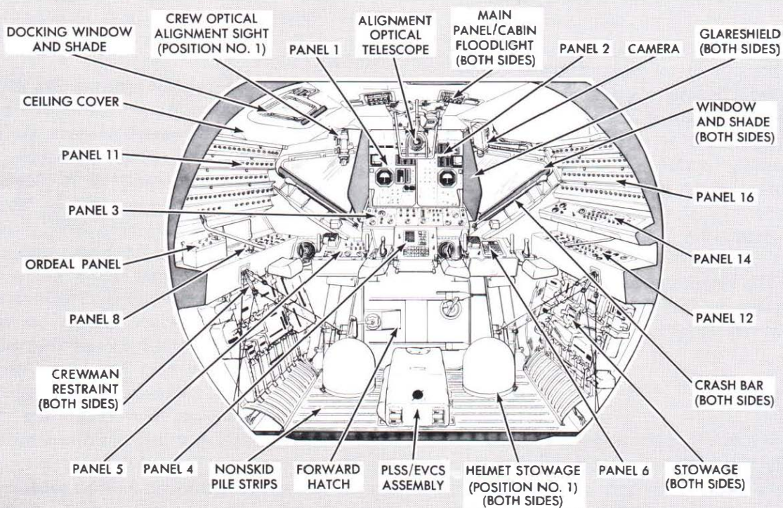
Crew Compartment Interior
