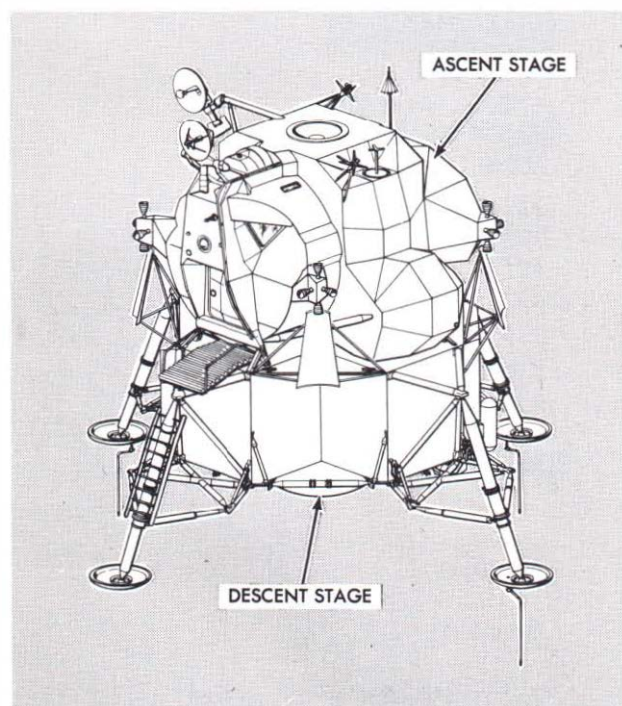
LM Configuration
