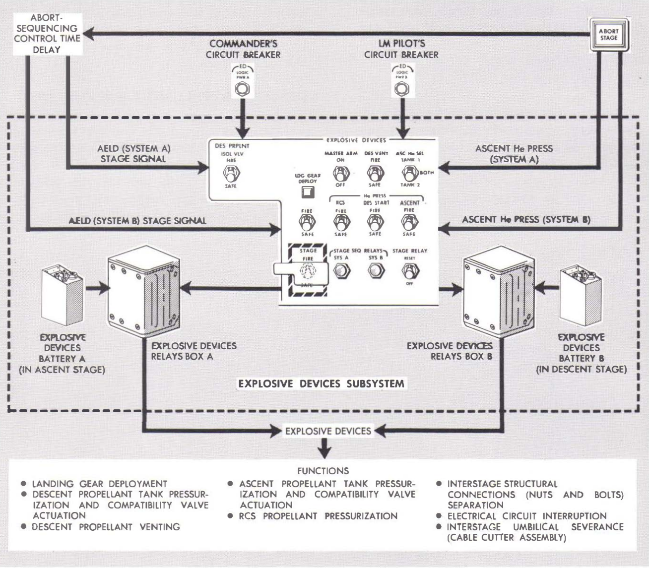
Diagram of Explosive Devices
