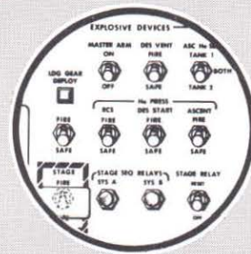
EXPLOSIVE DEVICES CONTROL PANEL
