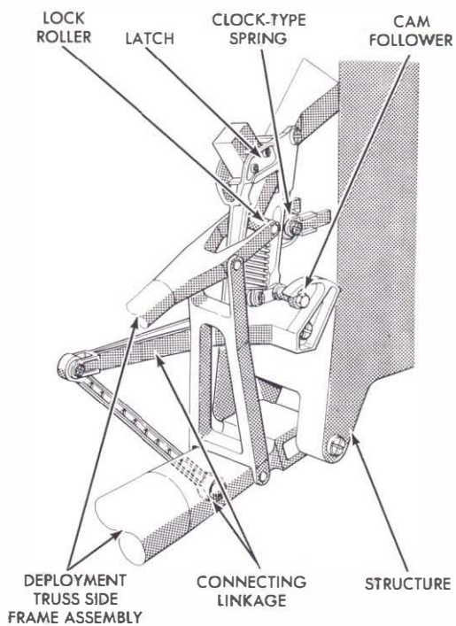
R-13 Deployment and Downlock Mechanism
