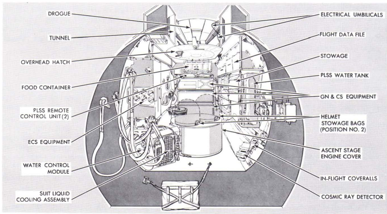
Midsection Interior
