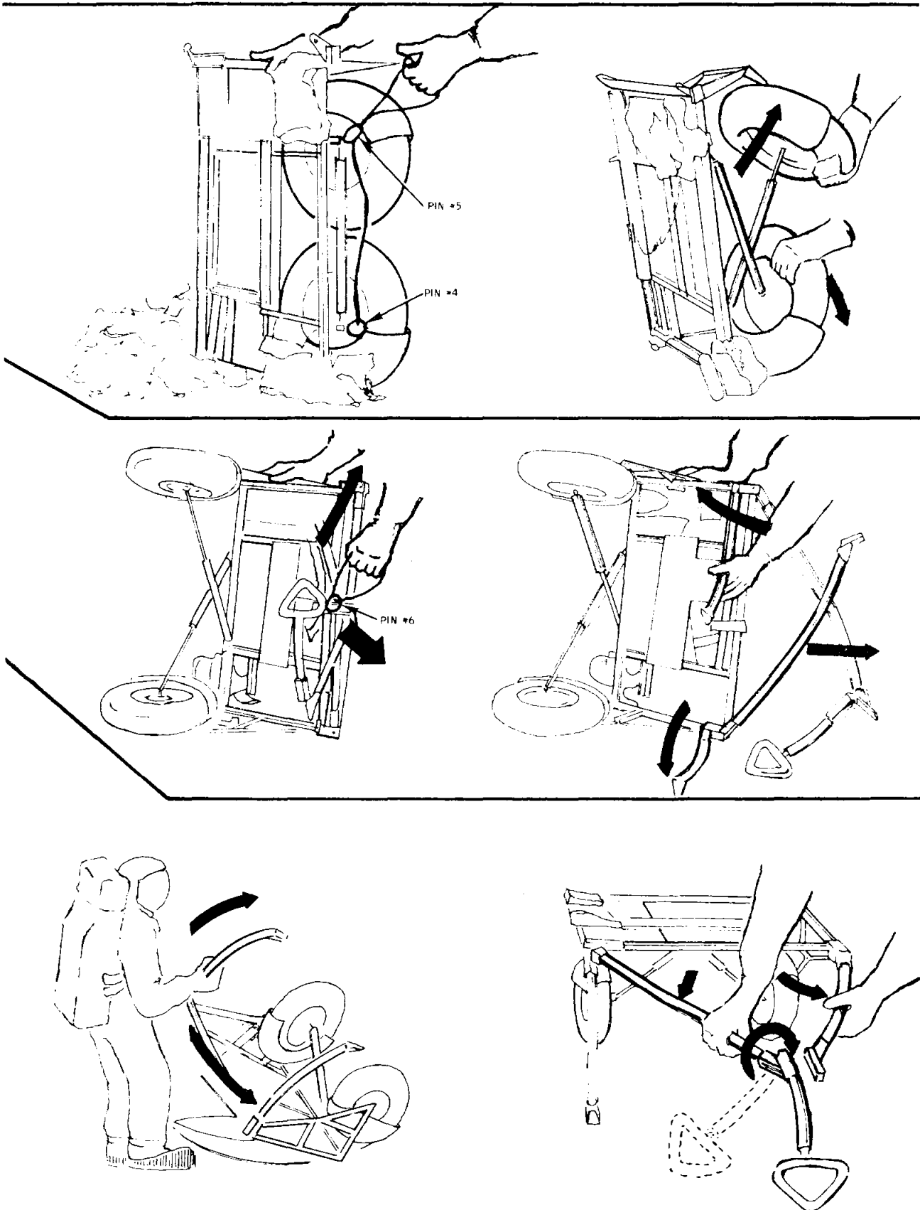
FIGURE 3.1-5 MET DEPLOYMENT
