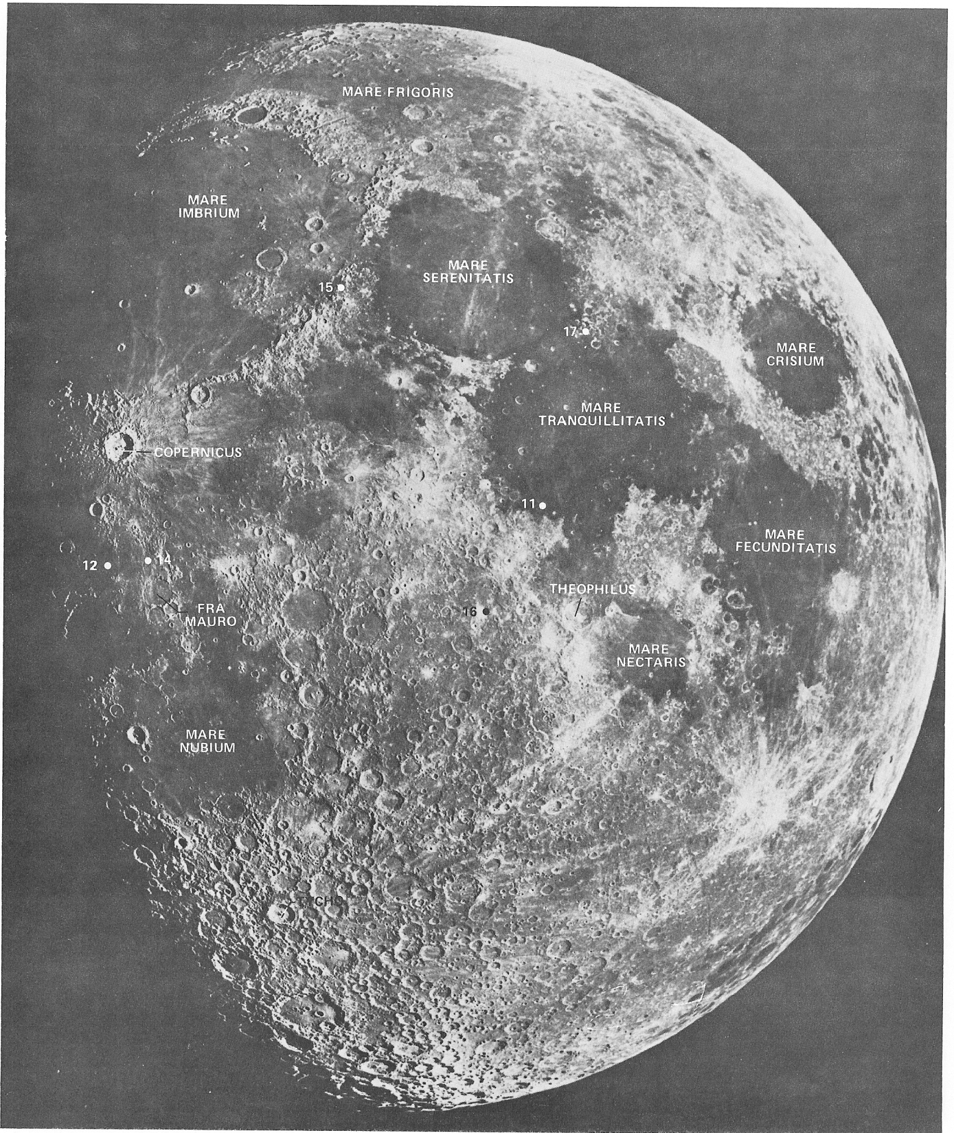
FIGURE 1.—Telescopic photograph of 9-day Moon showing Apollo 11–17 landing sites. Photograph number 113C, August 12, 1940 by J. H. Moore and J. P. Chappell. Lick Observatory 36-inch telescope. North is at top.
