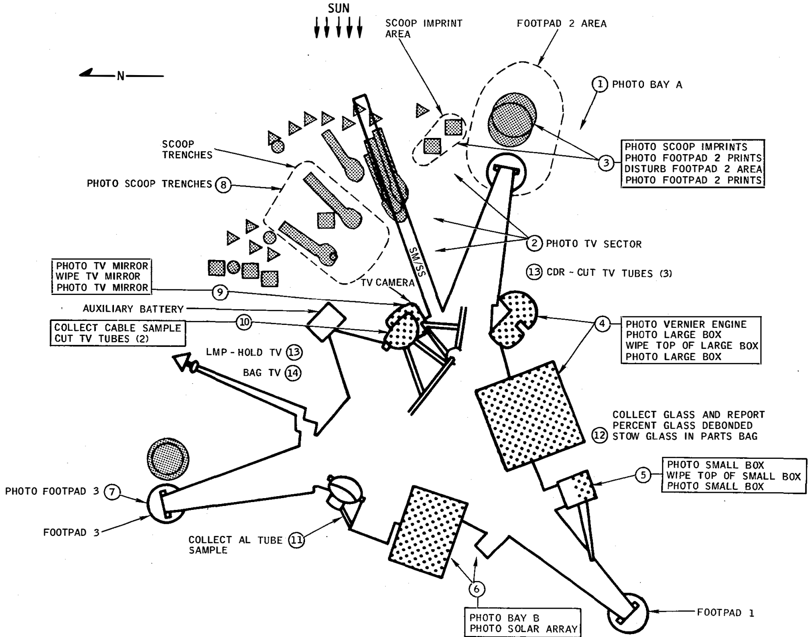
FIGURE 3-10 SURVEYOR INVESTIGATION ACTIVITIES
