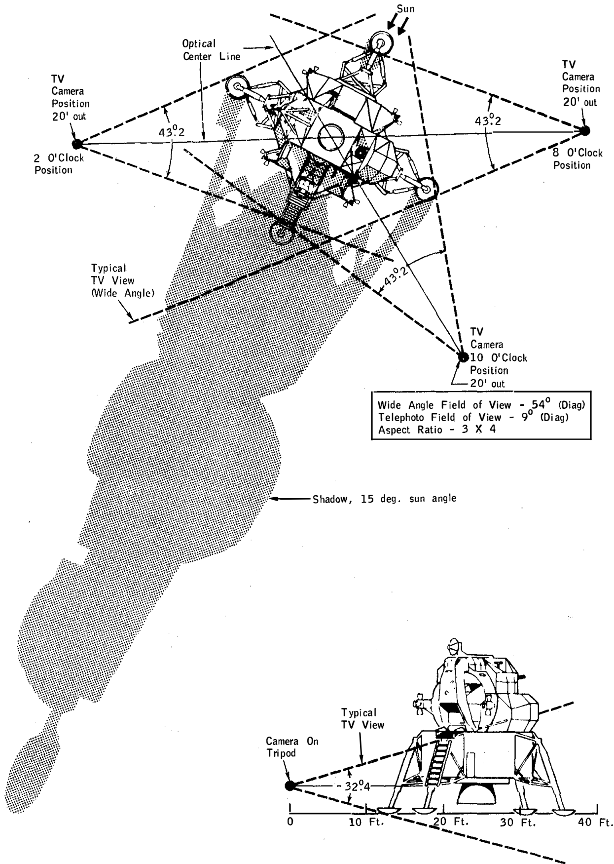
FIGURE 3-1 - COLOR TV FIELD OF VIEW FROM TRIPOD
