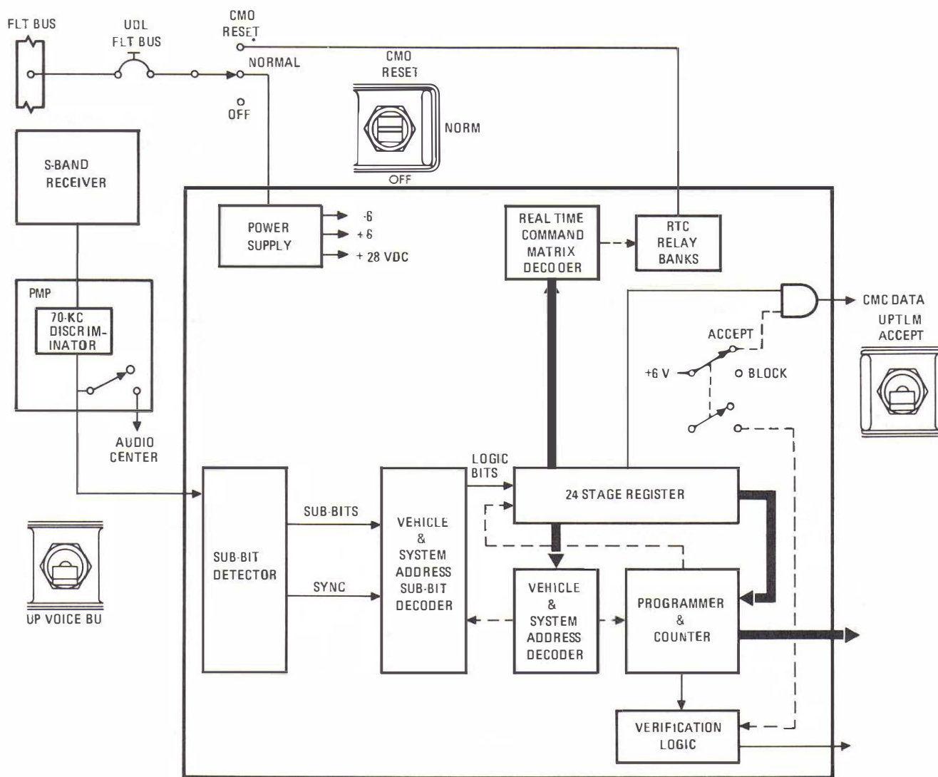
Block diagram of up-data link
