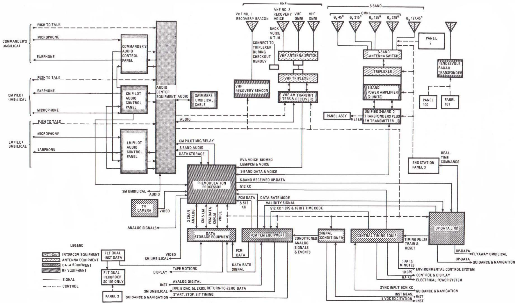
Telecommunications subsystem
