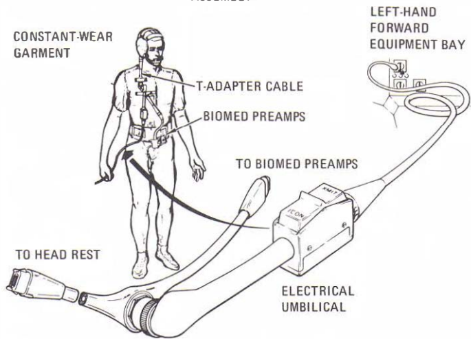
Communications cable
