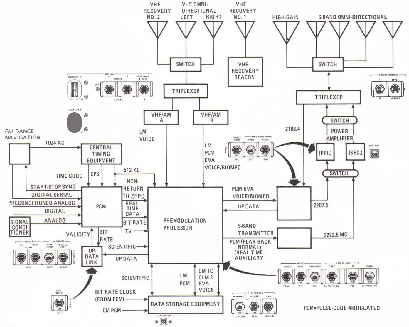
Data system relationship to other systems
