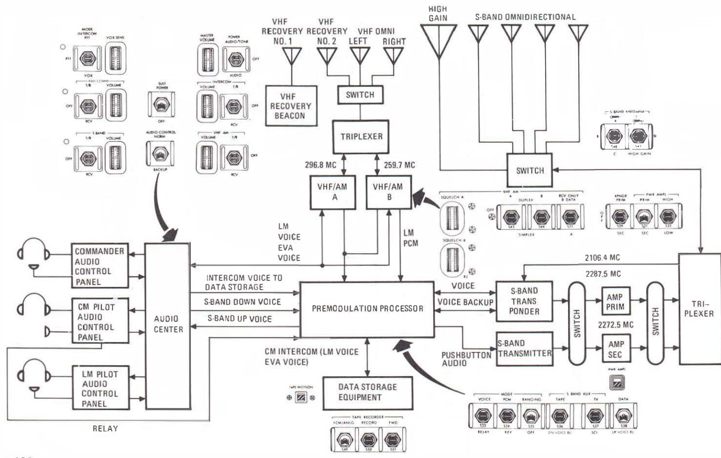
Audio system relationship to other systems
