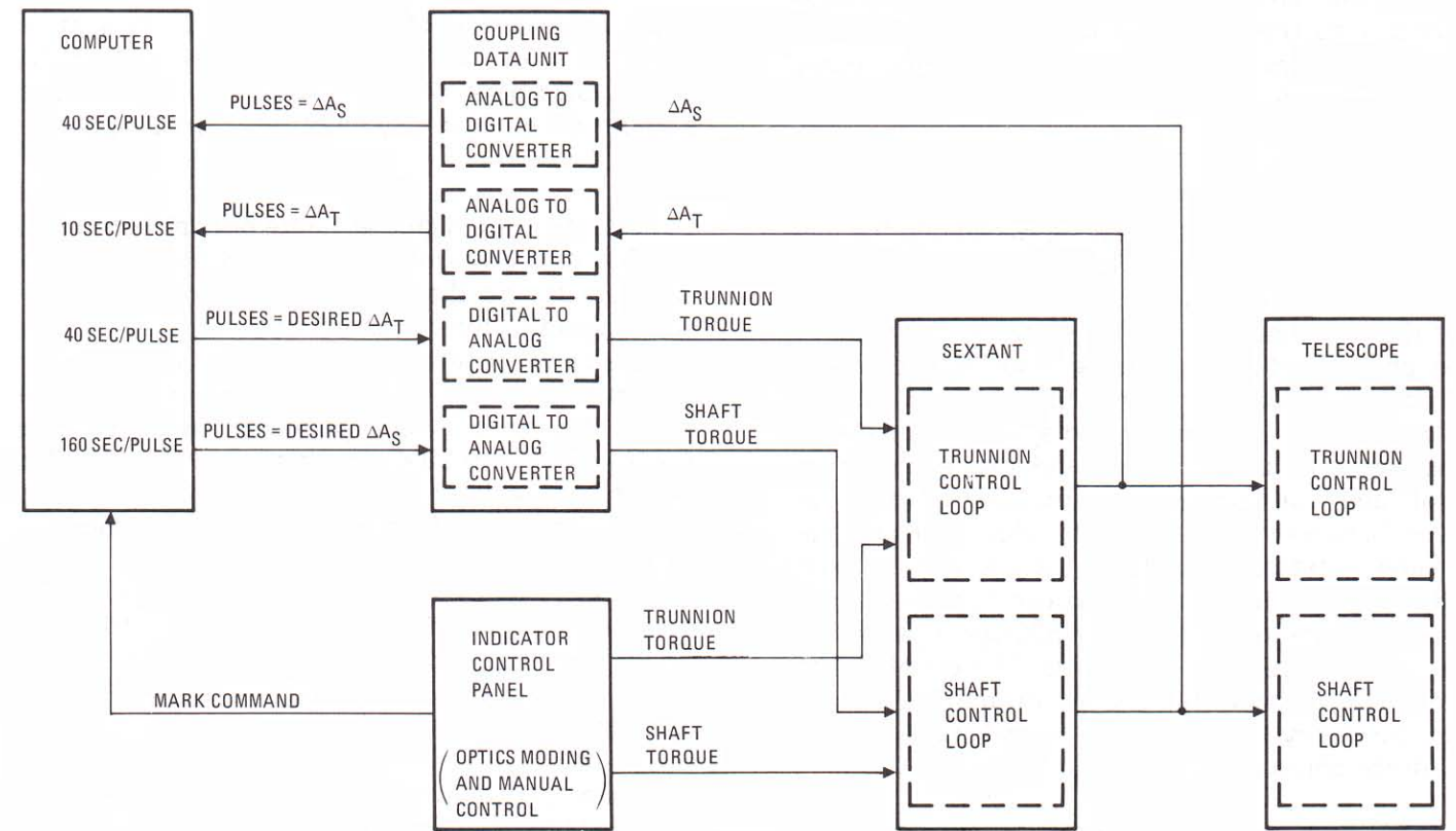
Schematic of optical subsystem
