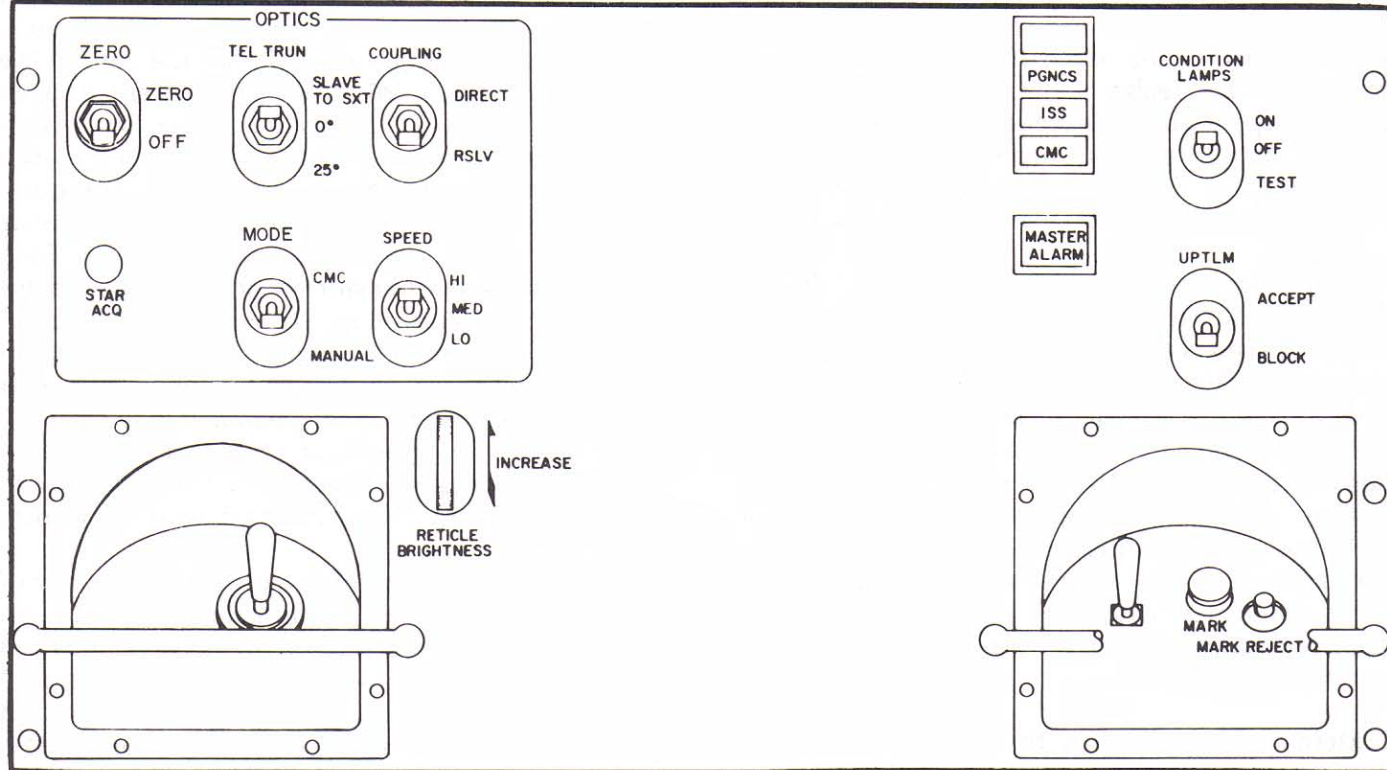
Optics control panel
