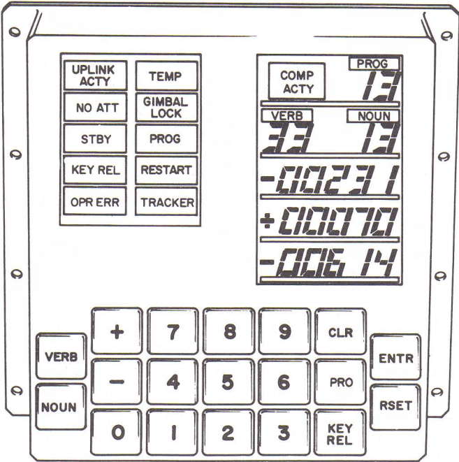
P-267 Computer display and keyboard
