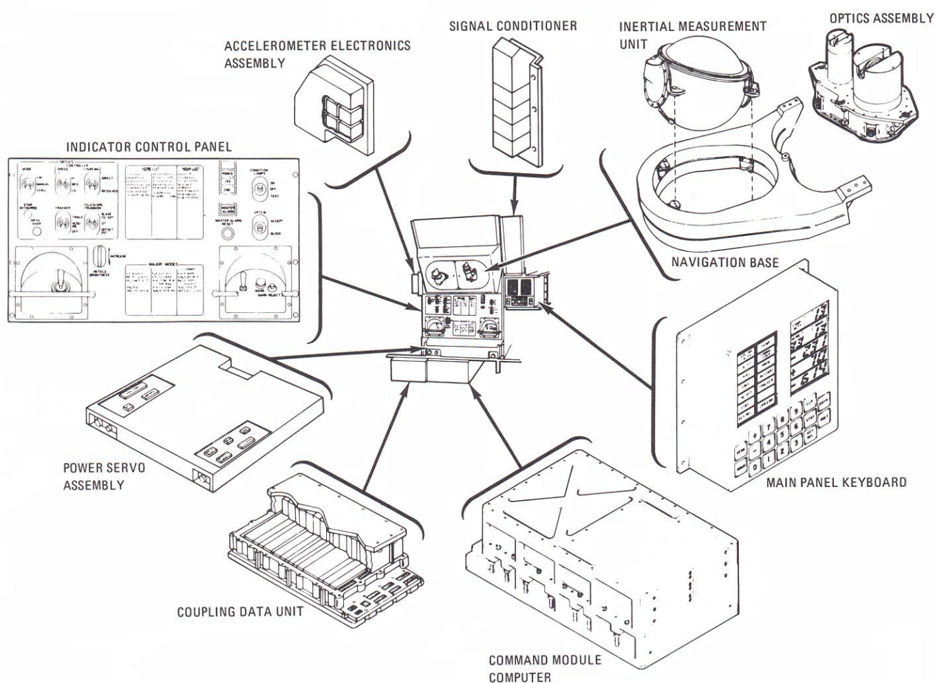
Major guidance and navigation subsystem equipment
