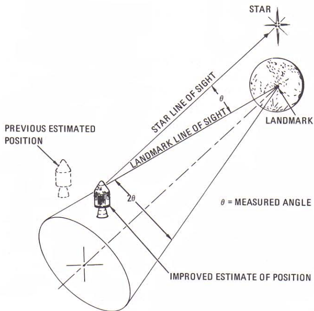
Determination of midcourse position
