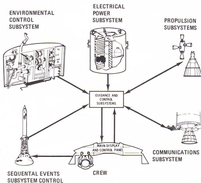
Guidance and control relationship to other subsystems
