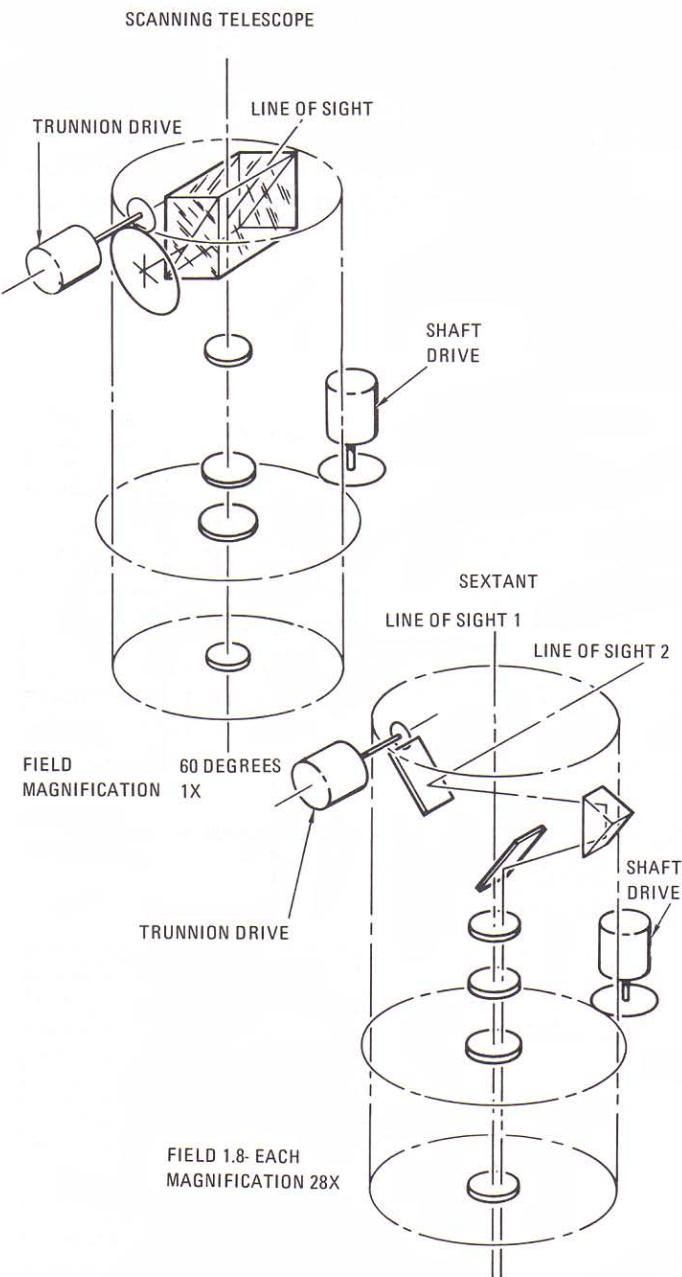
Schematic of sextant and telescope
