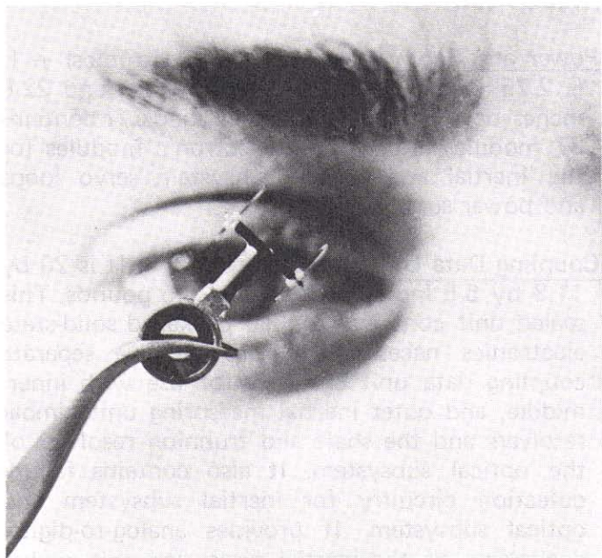
This tiny pendulum is heart of an accelerometer, a key component in guidance and navigation subsystem.
