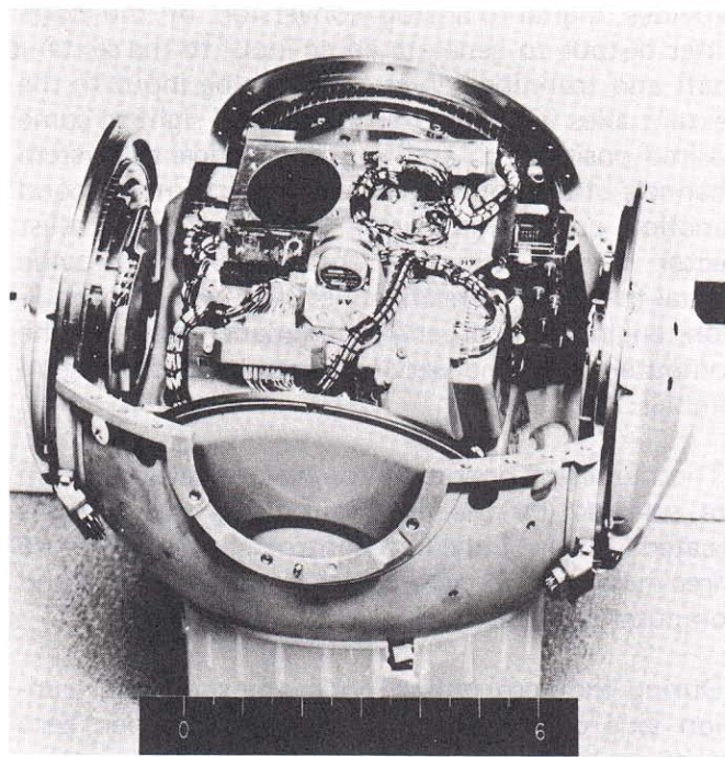
Cutaway of inertial measurement unit
