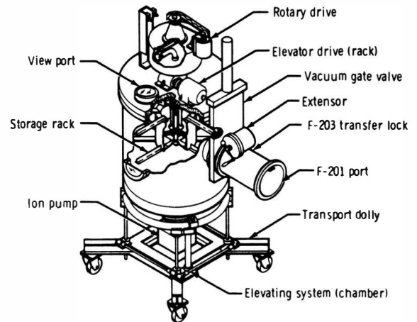
Figure 8. - The F-207 sample carousel.
