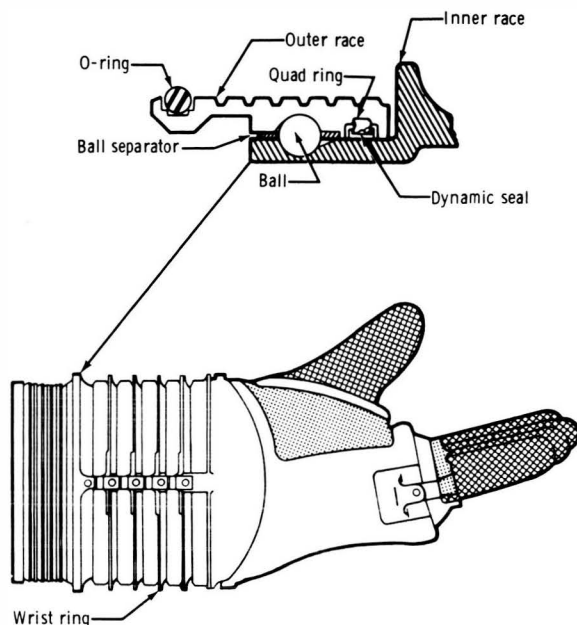
Figure 15. - Side view of glove and wrist assembly.
