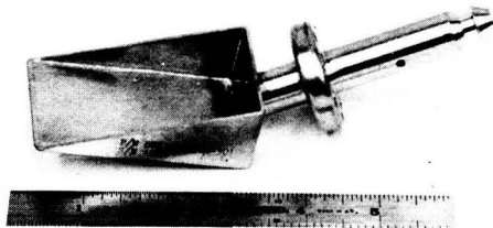
Figure 21. - Five-centimeter (2 inch) scoop (SEZ 36104724-301).
