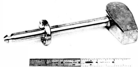
Figure 22. - Hammer (SEZ 36104728-301).
