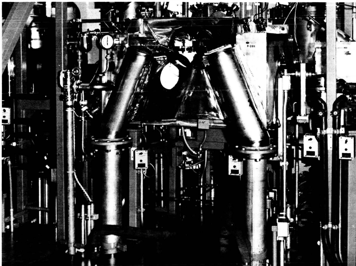
Figure 5. - The glove operator area of chamber F-201.
