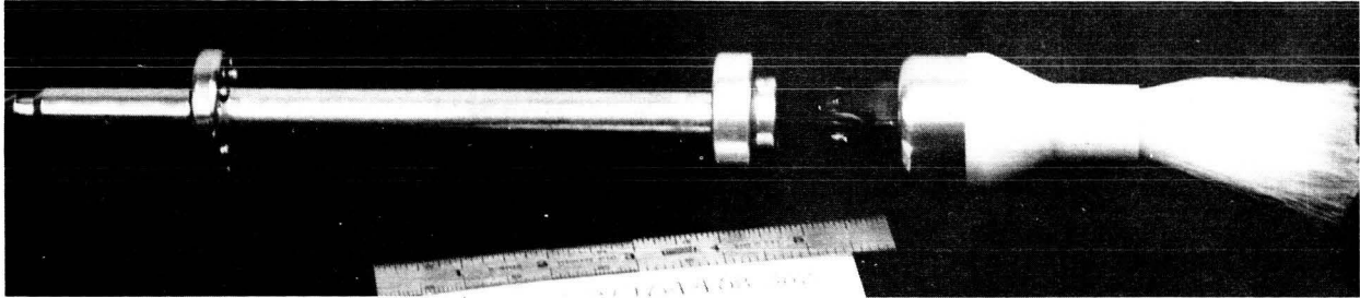
Figure 25.- Floor brush (SEZ 36104408-302).
