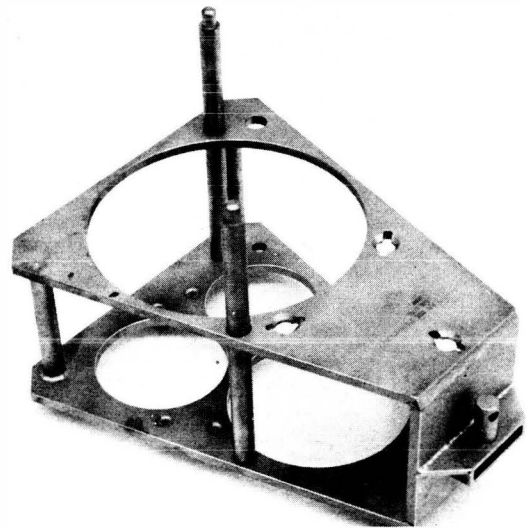
Figure 20. - Canholder assembly (SDZ 36106027-301).
