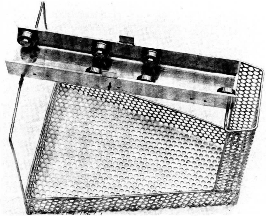
Figure 11. - Dolly and basket.
