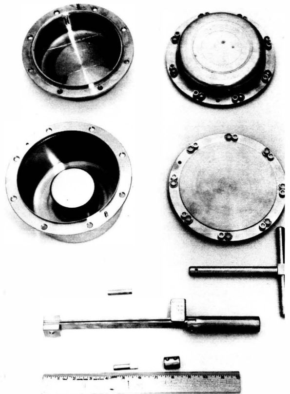
Figure 27.- Radiation counting sample containers and tools.
