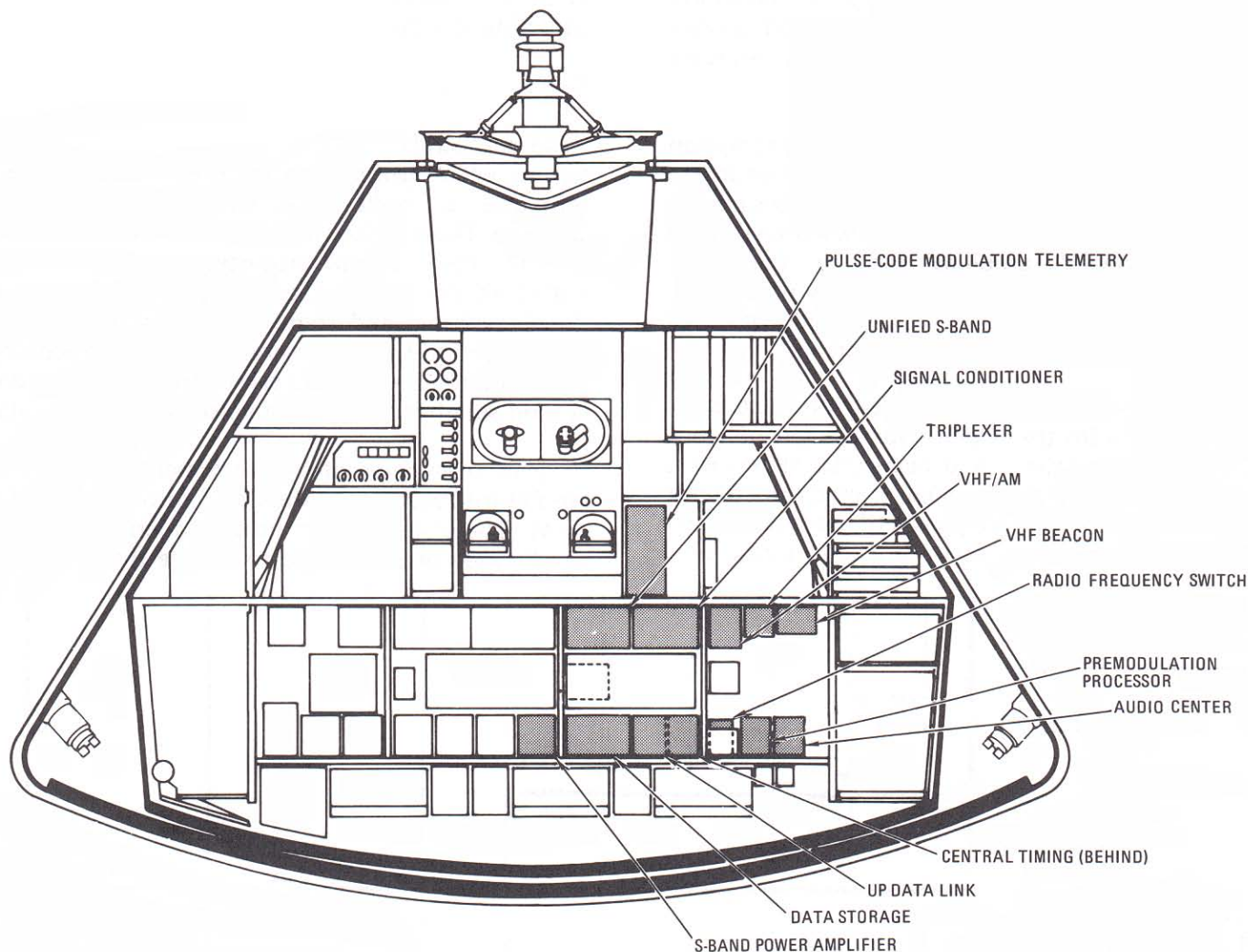
Location of main telecommunications equipment
