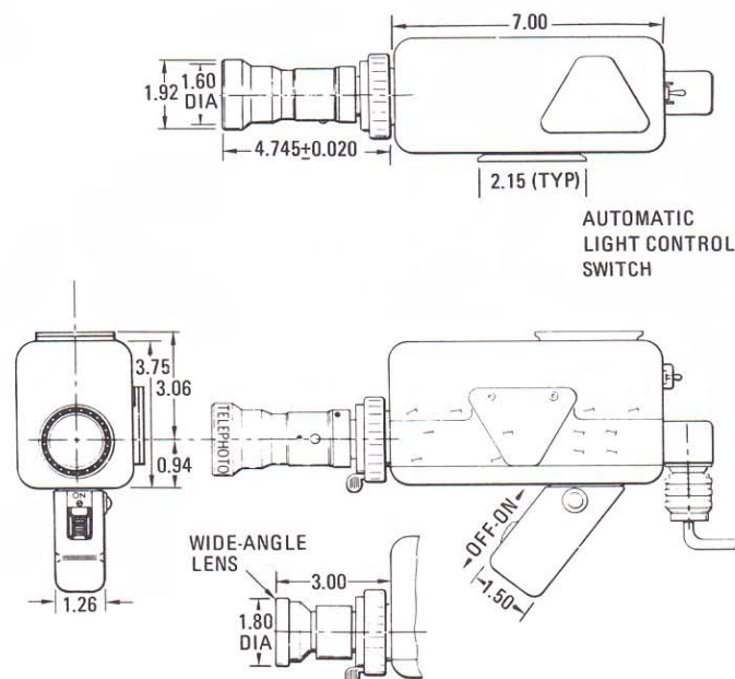
Apollo television camera
