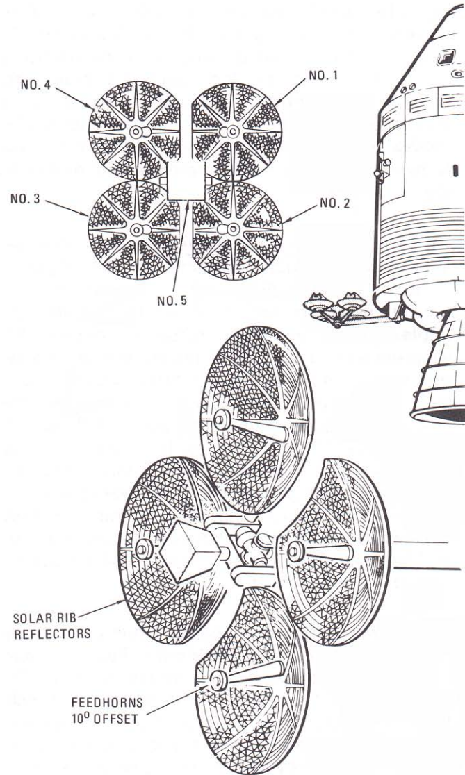
High-gain antenna construction
