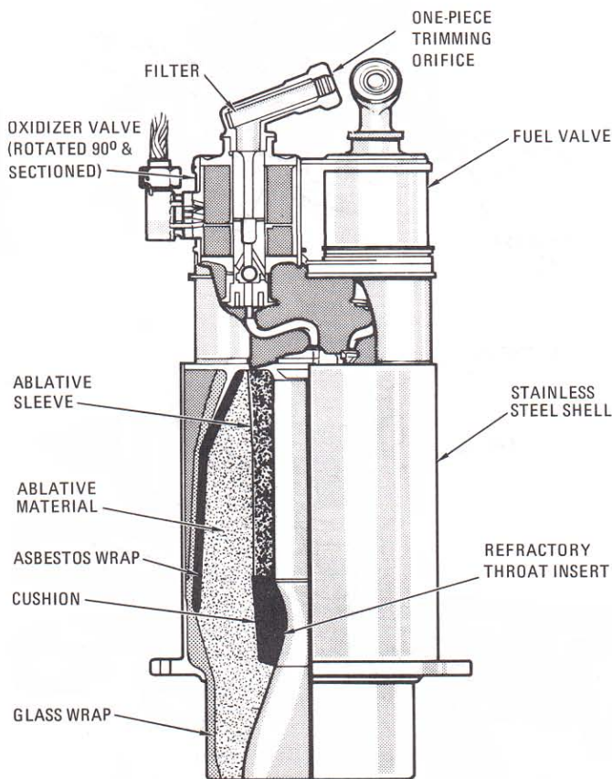
CM reaction control engine
