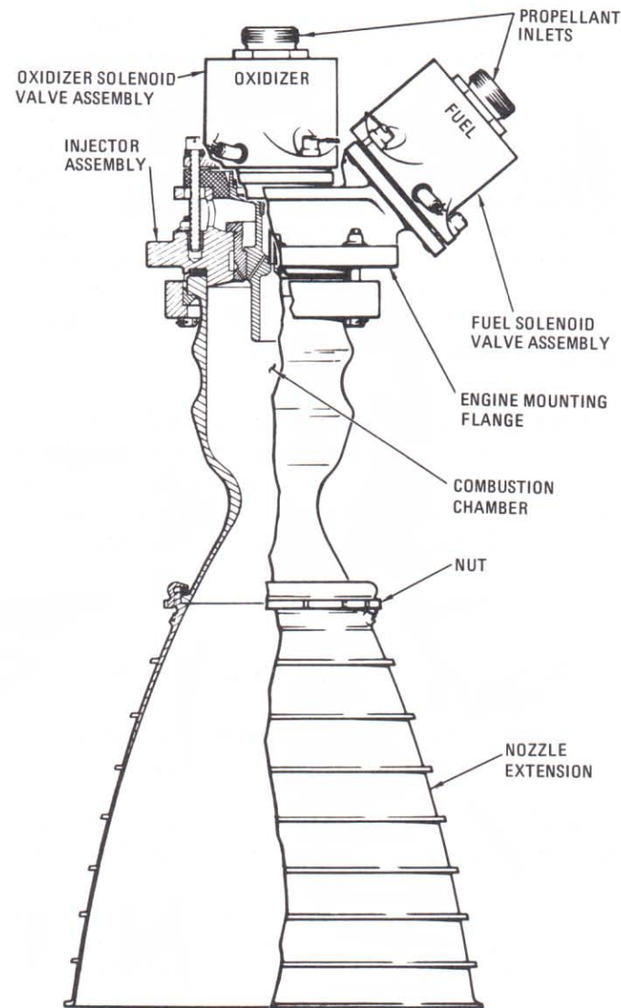
P-205 SM reaction control engine
