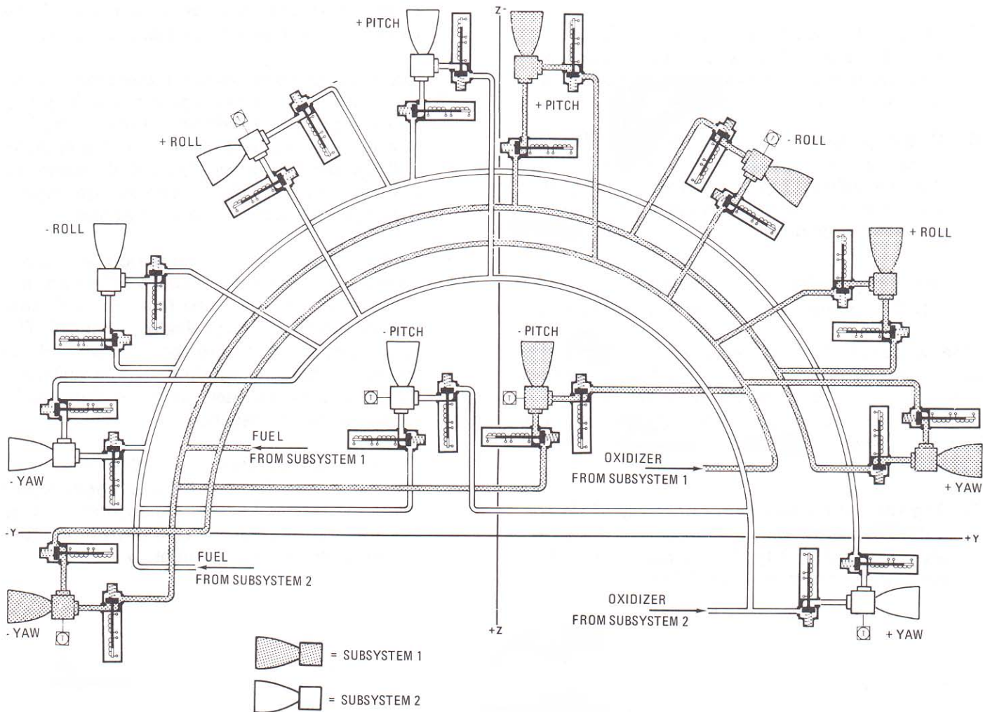
Schematic of reaction control engines
