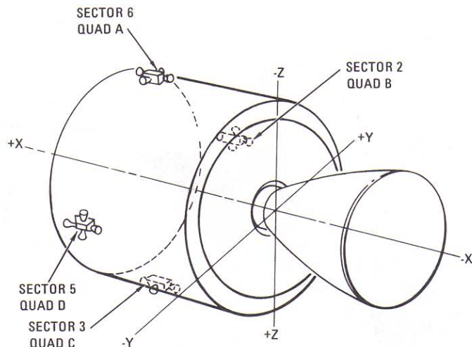
Location of SM quads
