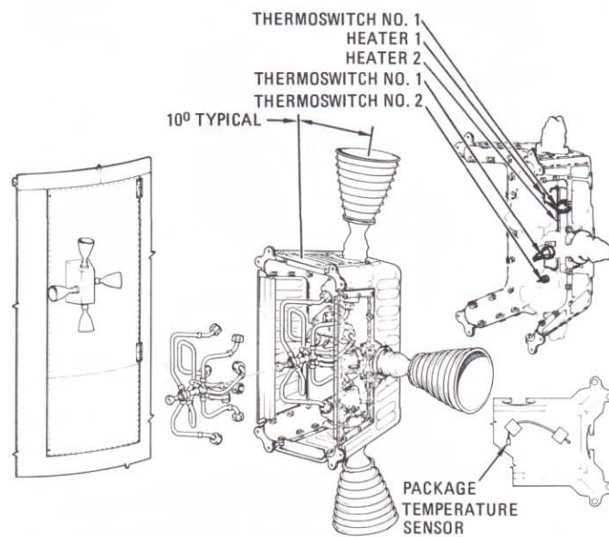
P-204 SM reaction control engine housing
