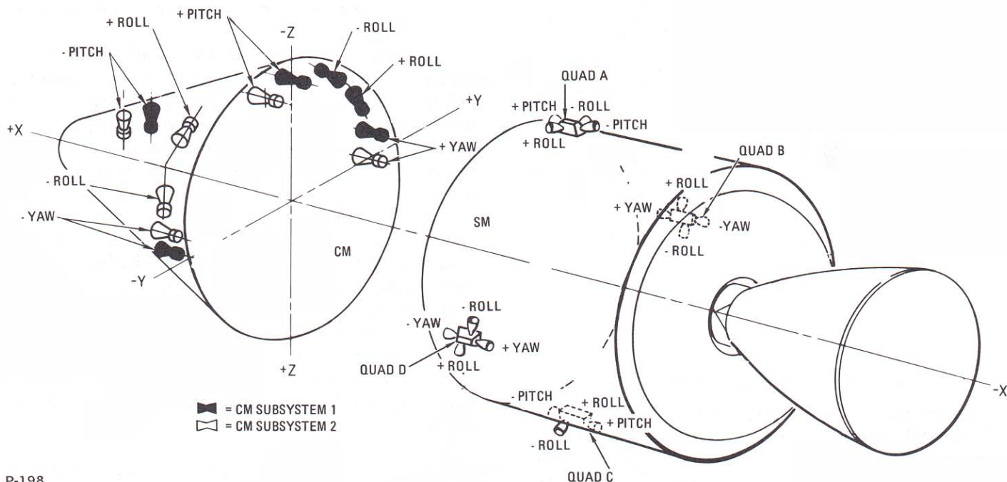
Location of reaction control subsystem engines
