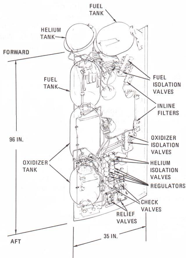
Typical SM quad
