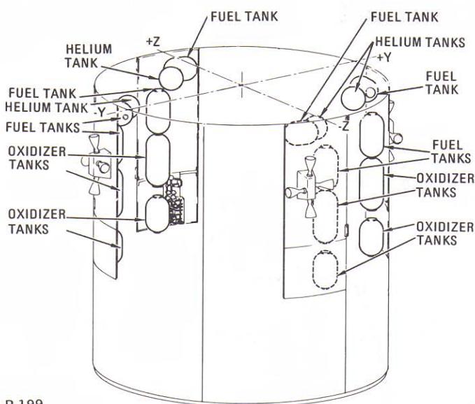
SM reaction control subsystem quads
