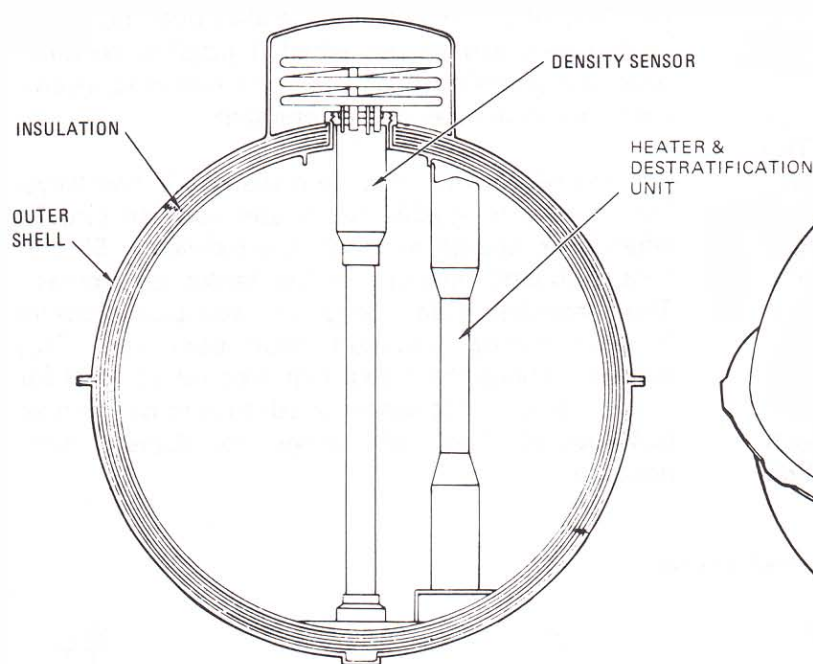
Cryogenic tank (hydrogen)
