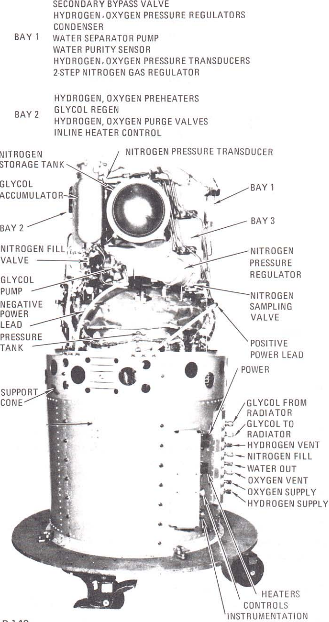
Fuel cell module accessories
