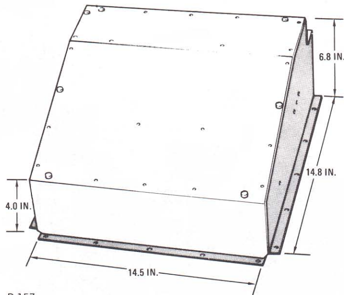
Size of static inverter
