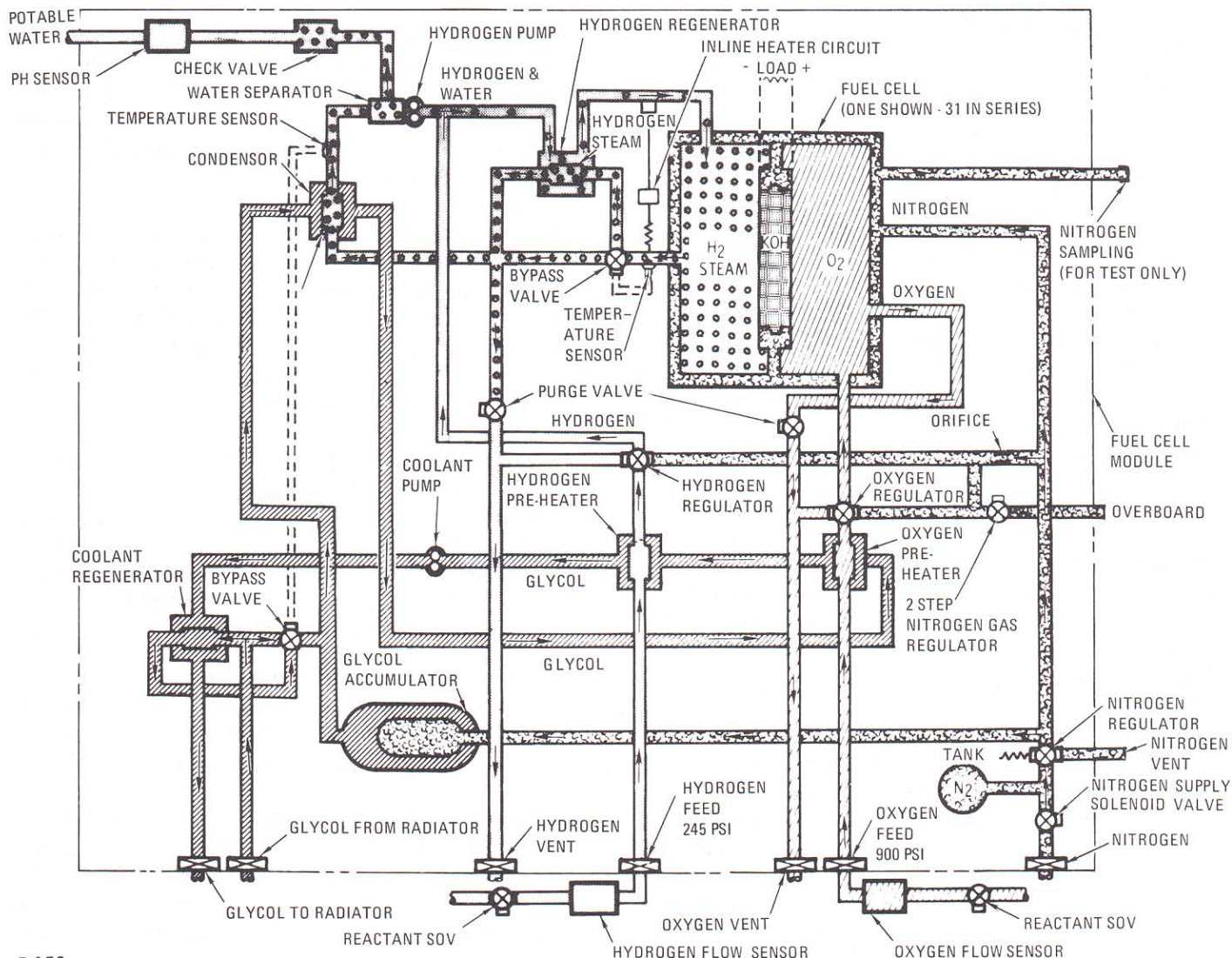
Schematic of fuel cell module
