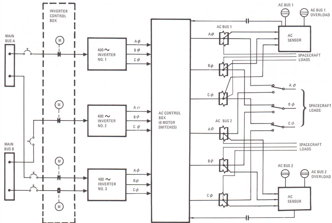
AC power distribution
