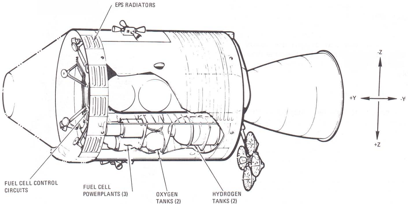
Location of major electrical power subsystem equipment
