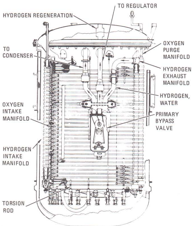
Fuel cell module
