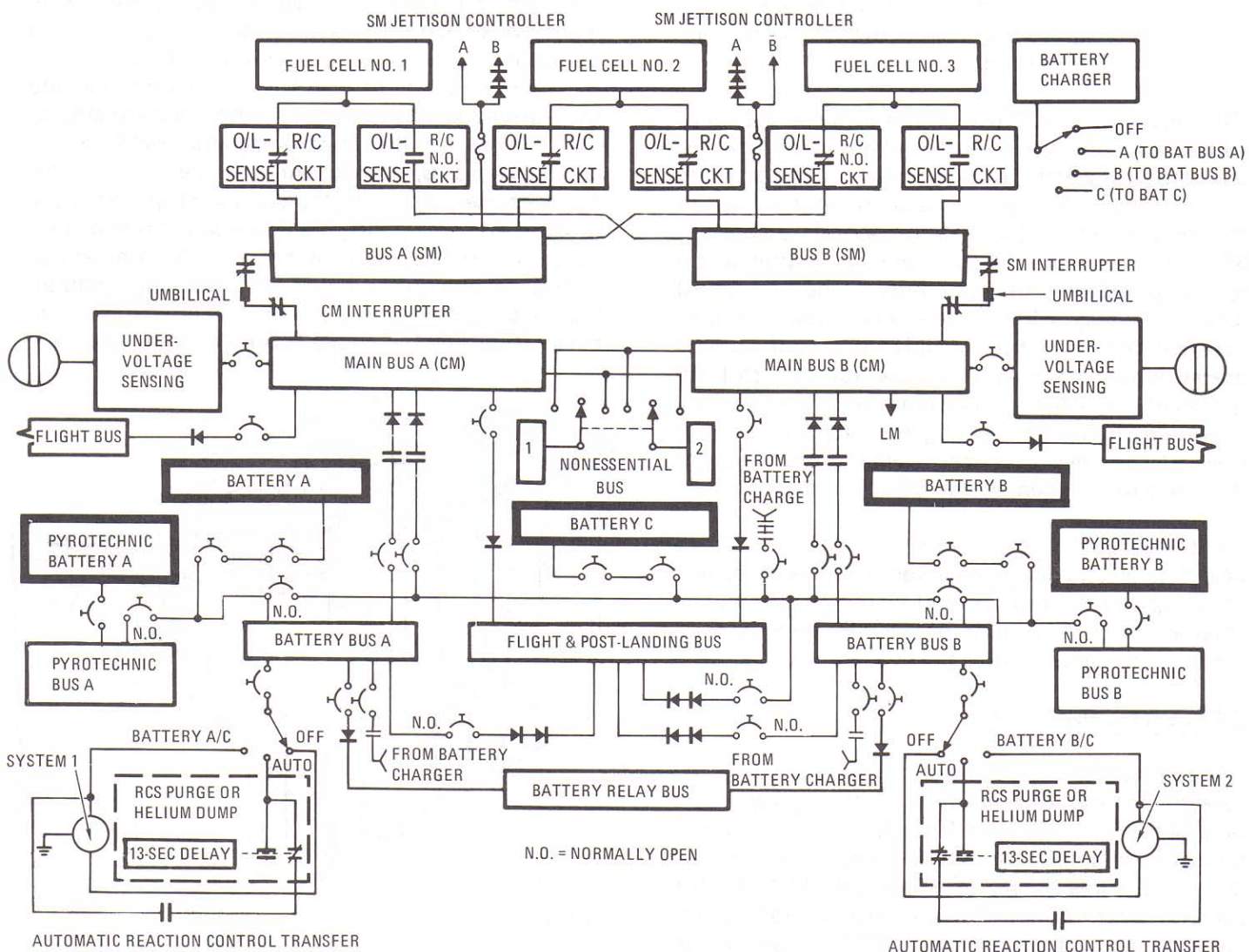
DC power distribution
