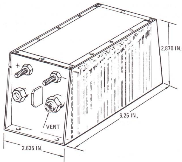
Pyrotechnic battery
