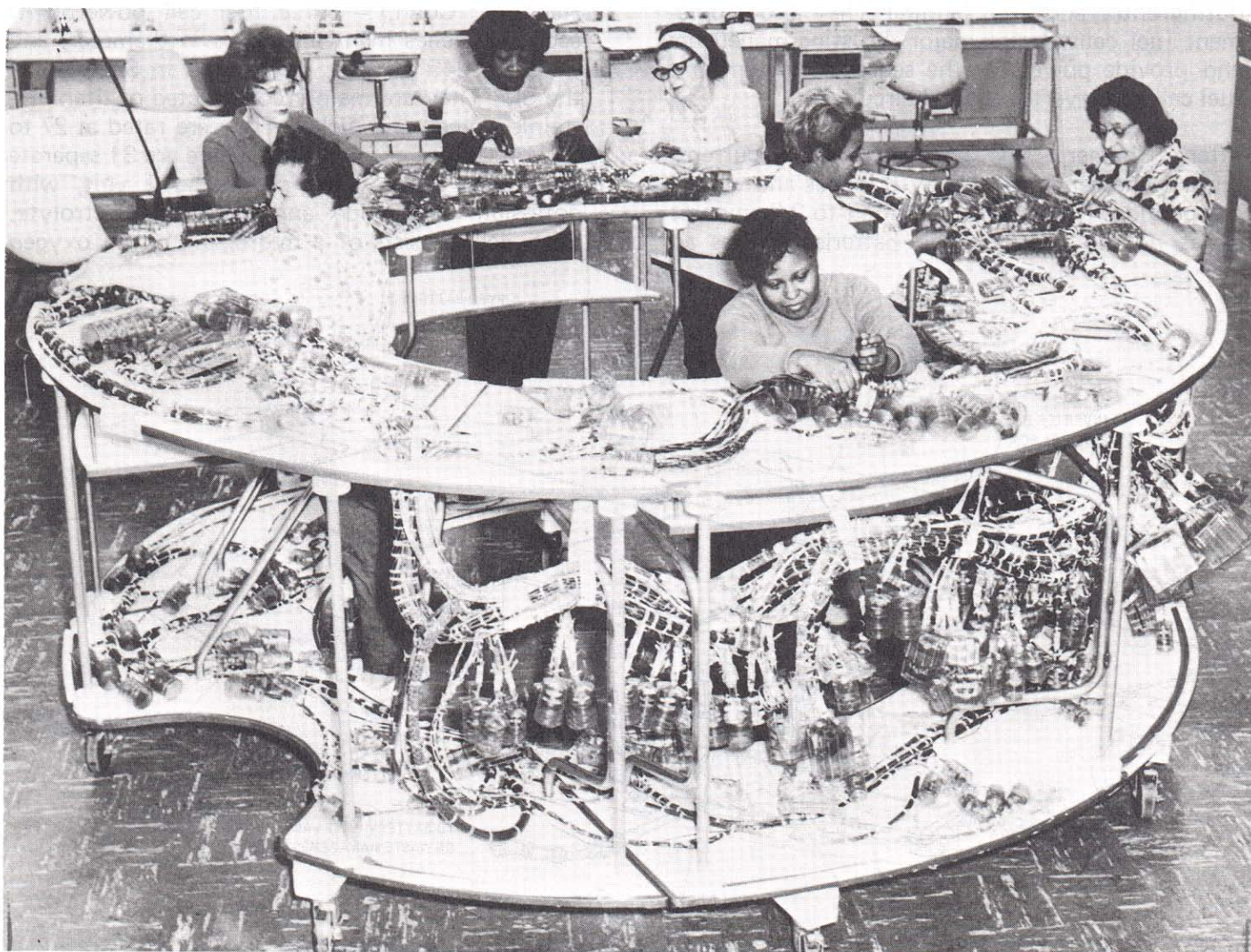
Command module wire harness is first assembled on this mockup stand
