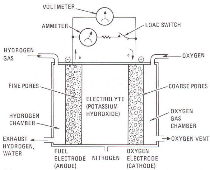
Electrochemical flow in fuel cell
