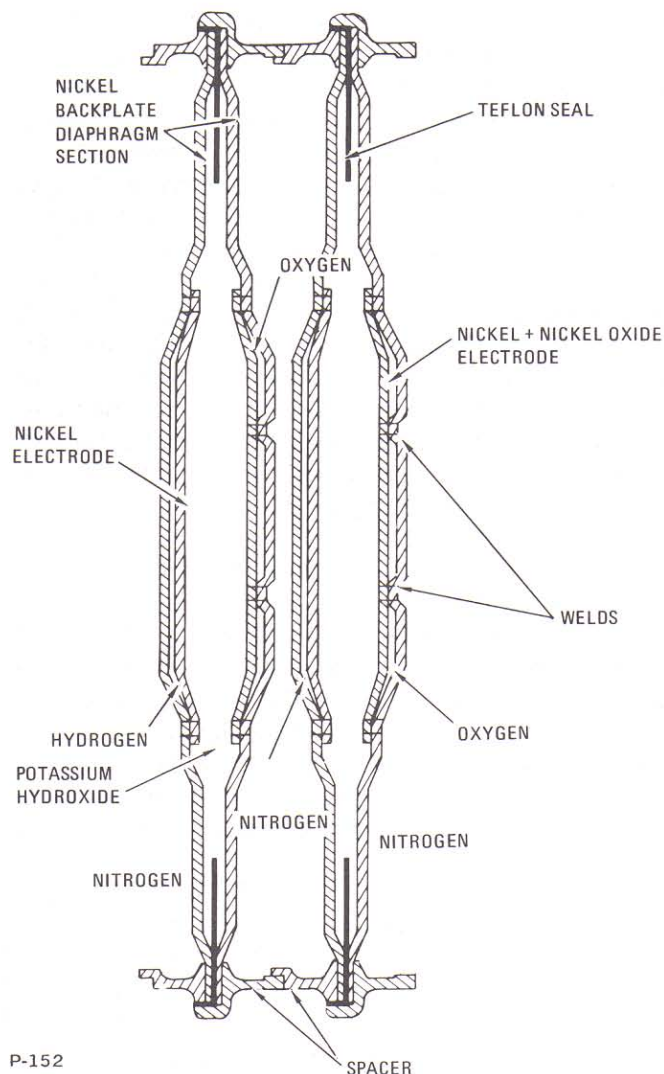
Cutaway view of cell
