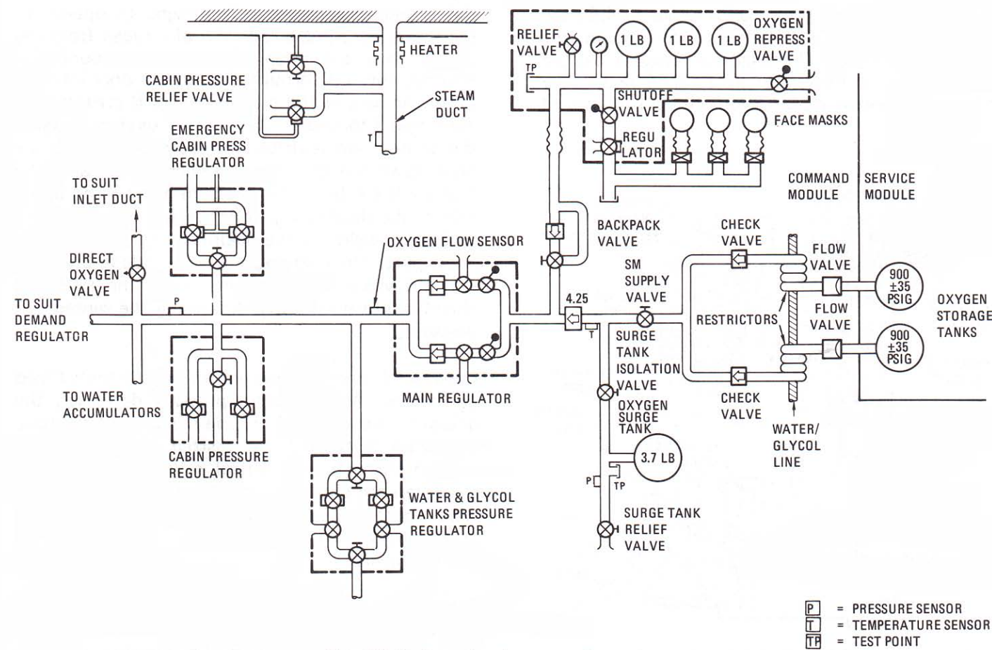
P-168 Simplified schematic of oxygen subsystem
