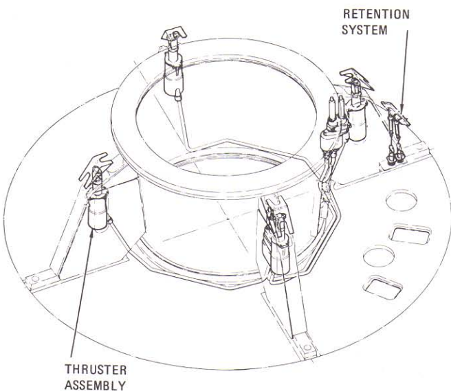
Forward heat shield retention and thruster system
