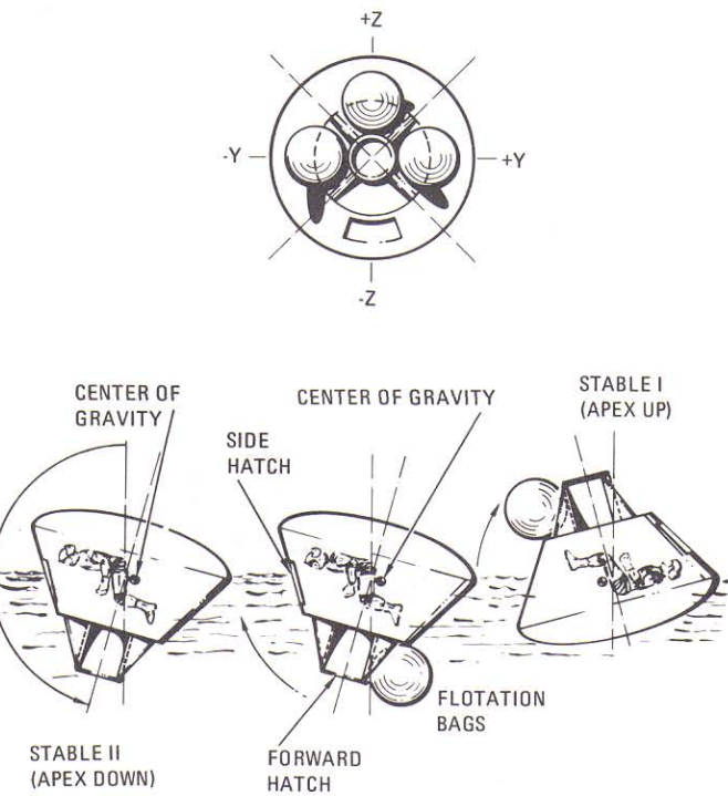
CM uprighting system
