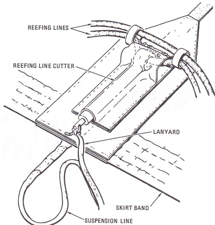
Reefing line cutter installation
