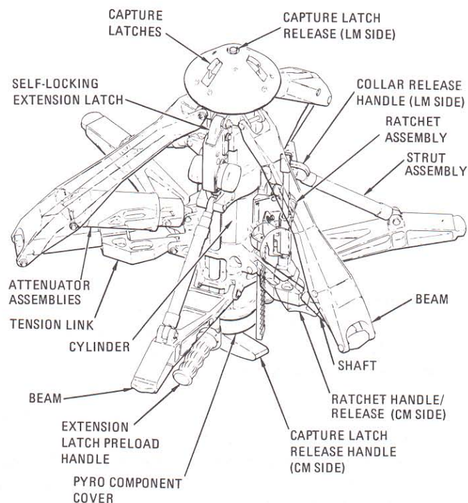
Probe assembly
