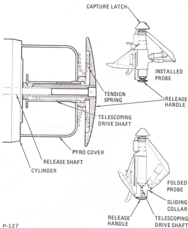
Capture latch release
