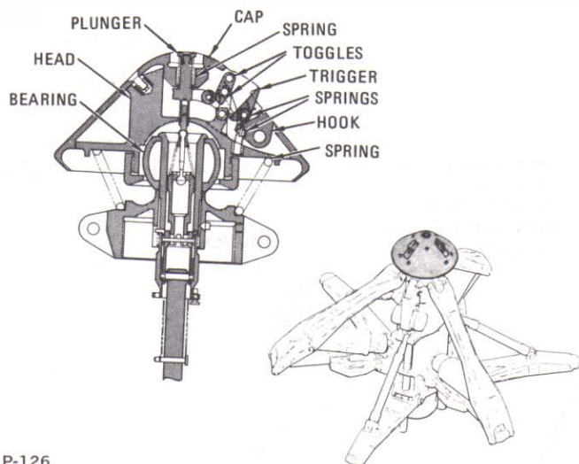
Capture latch assembly
