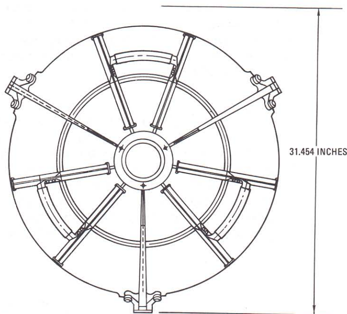
Drogue assembly
