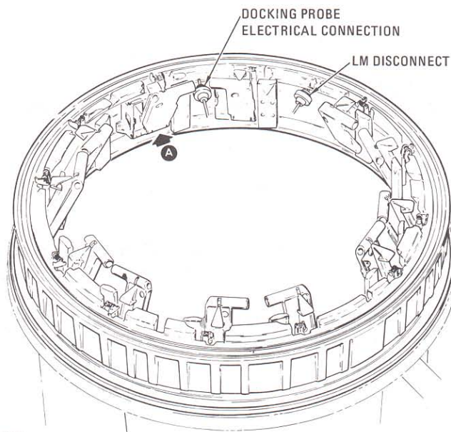
Docking latches
