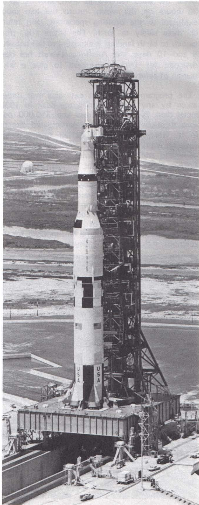
Saturn V/Apollo shortly before launch
