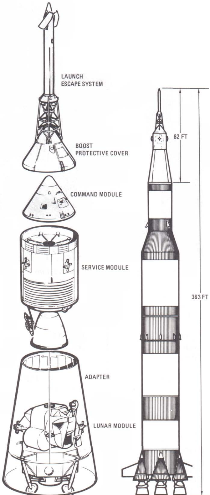
Apollo spacecraft
