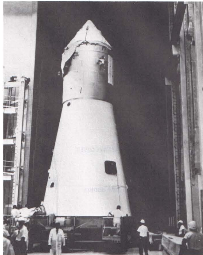
Spacecraft just before mating with Saturn V
