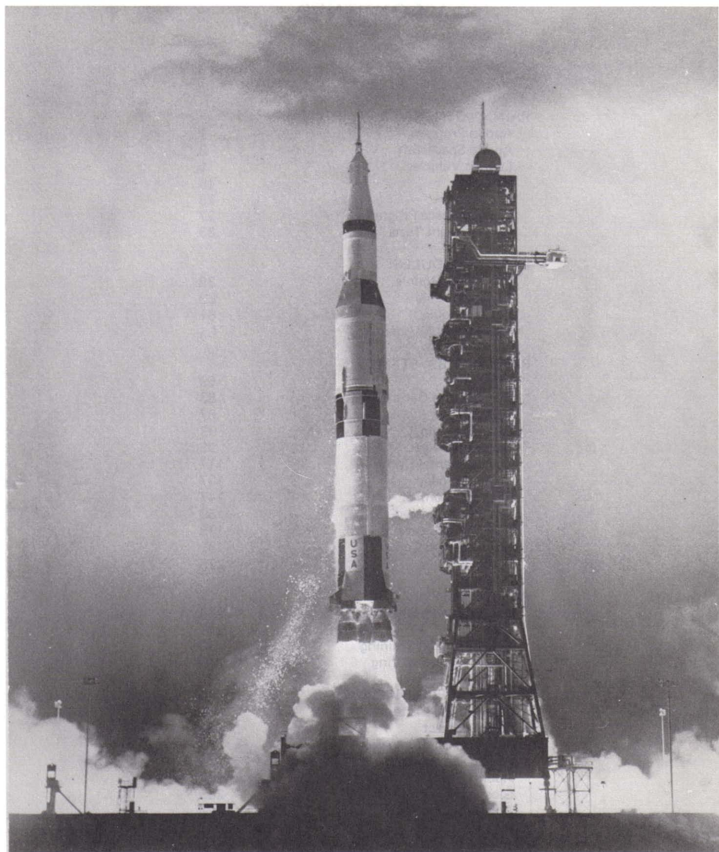
Saturn V lifts Apollo spacecraft off pad in unmanned flight test
