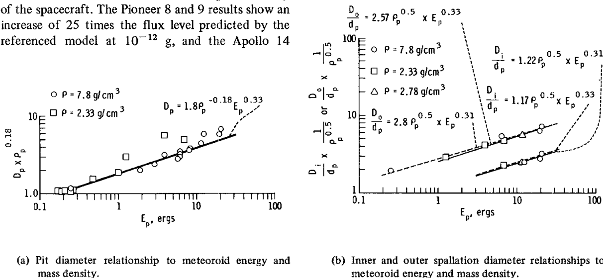
FIGURE 21-3.—Data from window calibration tests.
