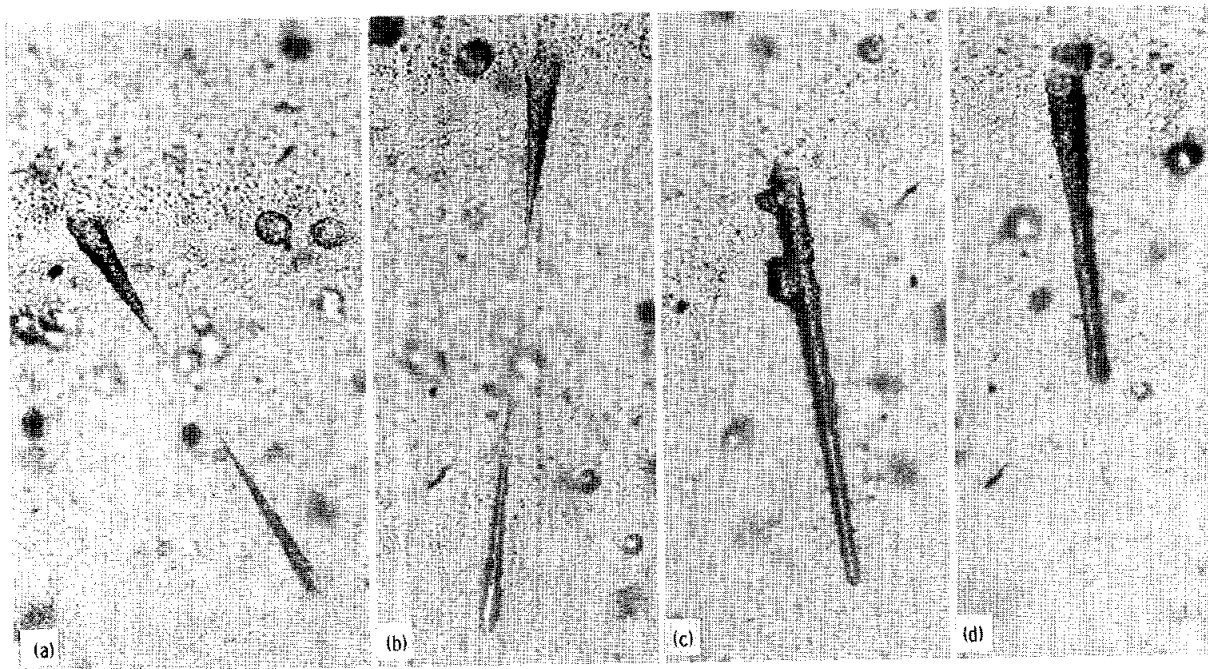
FIGURE 26-9. —Four tracks of highly ionizing cosmic ray particles as they pass through the CN detector. Tracks A, B, and D are from mouse A-3305, and track C is from mouse A-3326. These particles, possibly of the iron group, deposit substantial amounts of energy ( >0.1 \text{ MeV}/\mu\text{m} ) in the vicinity of their trajectories. Particles C and D are more ionizing than particles A and B. The top surface of each monitor is at the top of each photograph. Because the tracks extended through the CN layer at a small angle (i.e., more or less vertically) and thus were difficult to photograph in their entirety, the microscope stage on which they were located was tilted before photography. Magnification, \times 200 ; scale, 1 \text{ cm} = 32.5 \mu\text{m} . (From E. V. Benton and M. R. Cruty, University of San Francisco.)
