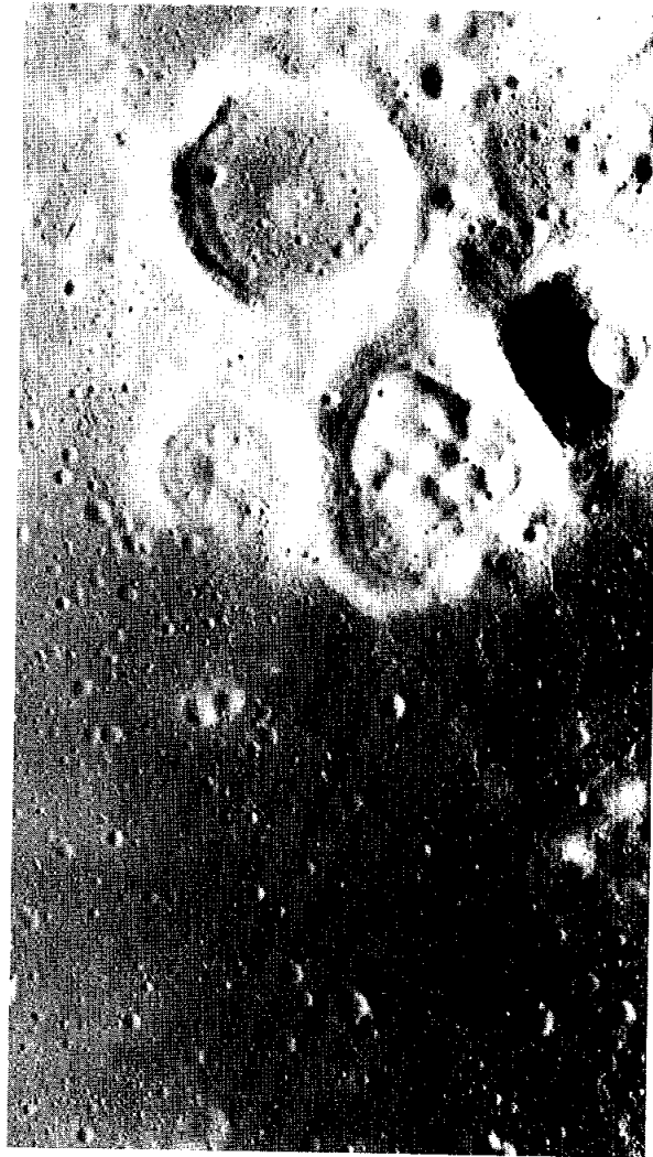
FIGURE 28-5.—Cluster of small craters (4 to 8 km in diameter) in the floor of Aitken Crater. Note the interior domical structures, the breaches in the walls, and the ridges and scarps in the dark floor material (lower right) (Apollo 17 panoramic camera frame AS17-1915).
