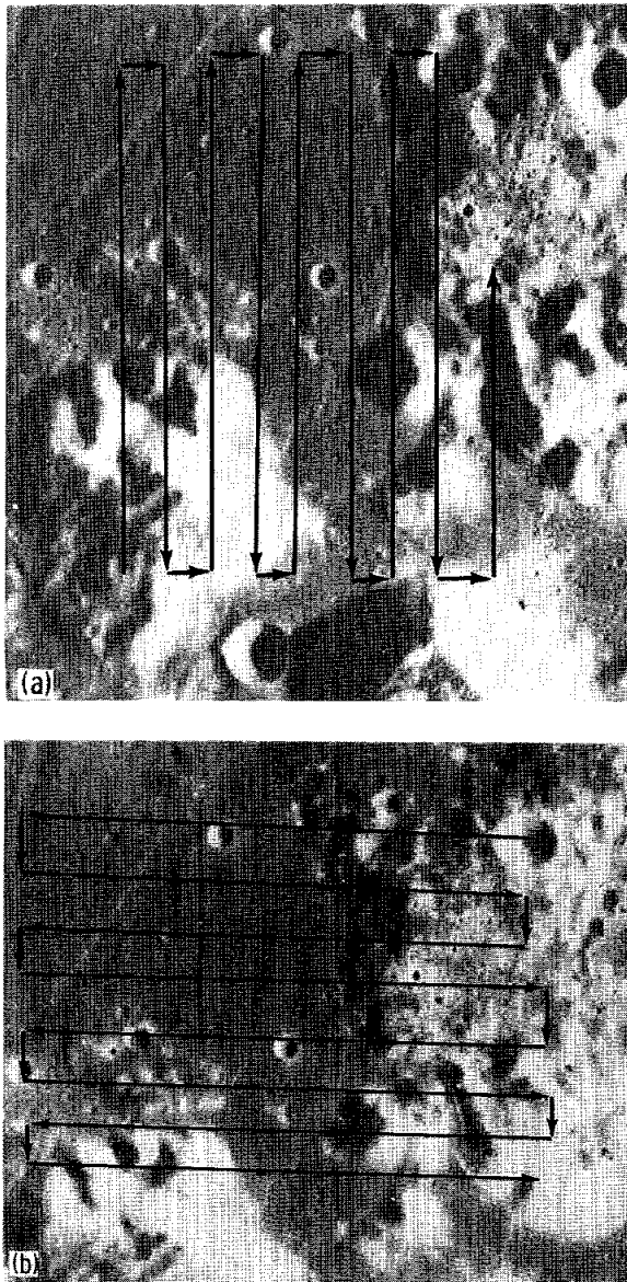
FIGURE 33-21.—Profile traverses used for standard error of measurements and analysis of slope effects. (a) Sun elevation angle of 16.5^\circ (Apollo 17 metric camera frame AS17-0446). (b) Sun elevation angle of 30.5^\circ (Apollo metric camera frame AS17-1500). (c) Sun elevation angle of 50.5^\circ (Apollo 17 metric camera frame AS17-2087).
