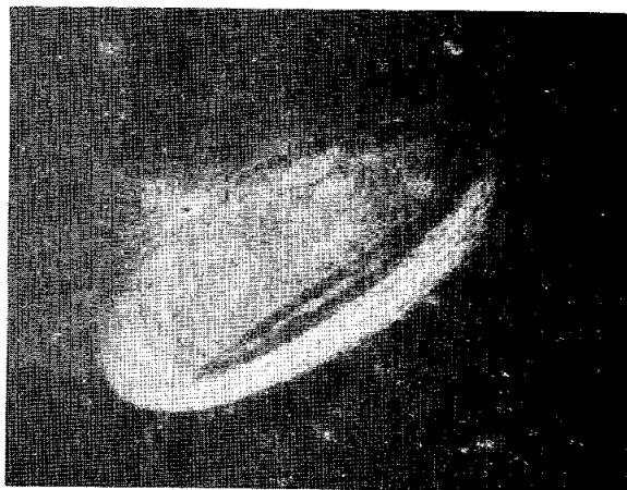
FIGURE 28-27.—Part of Apollo 15 panoramic camera frame AS15-127 showing the elongate Messier Crater in Mare Fecunditatis.
