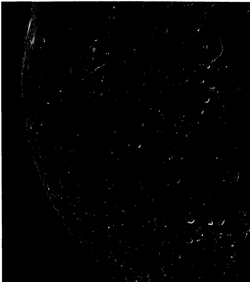
FIGURE 4-58.--A TEC view of Mare Australe. The center of this view is near latitude 35^{\circ} S, longitude 90^{\circ} E. In the upper middle, the large crater with dark material on its floor near both the left and right walls is Humboldt, centered at latitude 27^{\circ} S, longitude 81^{\circ} E (AS17-152-23288).
