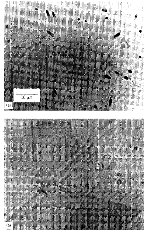
FIGURE 19-12.—Etched tracks in phosphate glass (GE-1457). (a) A typical view in the Apollo 16 detector, which was exposed during a solar flare known to have ejected particles into the interplanetary medium. (b) An atypical view in the Apollo 17 detector. The view is unusual in that it contains a track. Each detector was etched in 48 percent hydrofluoric acid to remove 0.5 \times 10^{-4} cm of glass.
