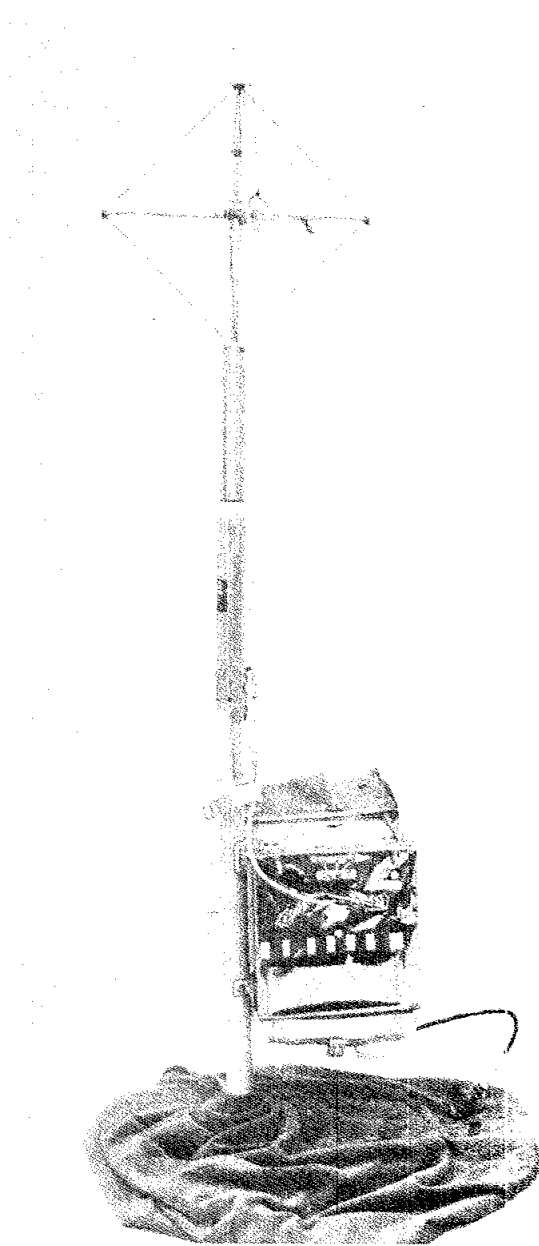
FIGURE 15-8.—The SEP experiment receiver and antennas. The receiver electronics, including tape recorder and battery, are contained in the box ( 23\text{ cm}^3 ), which usually is completely enclosed in a thermal blanket. The thermal blanket has been opened to show optical surface reflectors. The three-loop antenna assembly, folded during the journey to the Moon, is shown unfolded as it was used on the Moon.
