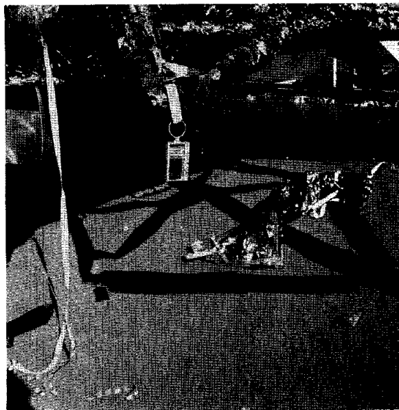
FIGURE 19-3.—The Sun half as deployed on the Moon. This photograph is one of a pair of stereoscopic pictures taken by the lunar module pilot (LMP) from a distance of 2.13 m (7 ft) immediately before termination of the experiment (AS17-140-21381 and 21382). Another pair of stereoscopic photographs was taken of the shaded portion (AS17-140-21383 and 21384).
