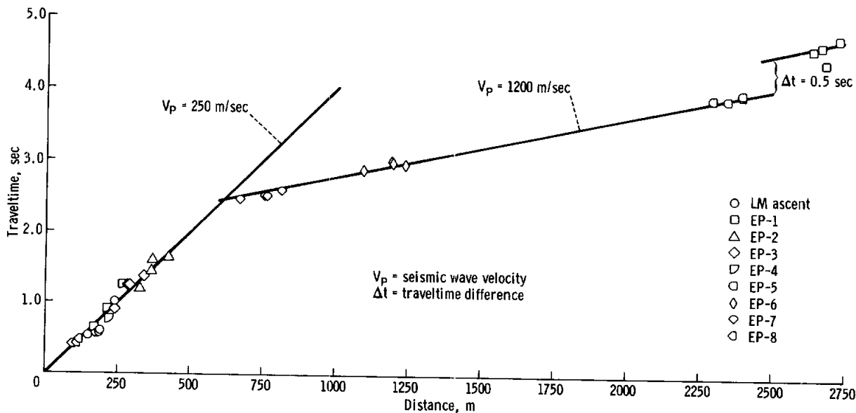
FIGURE 10-13.—Seismic arrivals from the detonation of the explosive charges plotted on a travelttime/distance graph.
