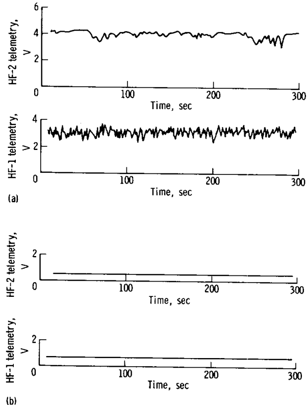
FIGURE 22-31.—Telemetry recordings of the receive-only noise levels observed on the lunar near side and far side. (a) Near side. (b) Far side.
