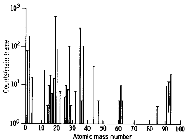
FIGURE 17-4.—Reduced spectrum taken 100 hr before sunrise of the third lunar night after deployment (16:30:00 G.m.t., Mar. 5, 1973). The solar zenith angle is 140^\circ . Corrections have been applied for background counting rates.
