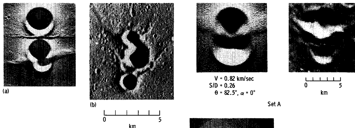
FIGURE 32-25.—Comparison of three simultaneously produced laboratory craters with lunar crater triplet. (a) Experimental craters. (b) Lunar craters (figs. 32-19 (inset) and 32-20) (part of Apollo 15 metric camera frame AS15-1699).
