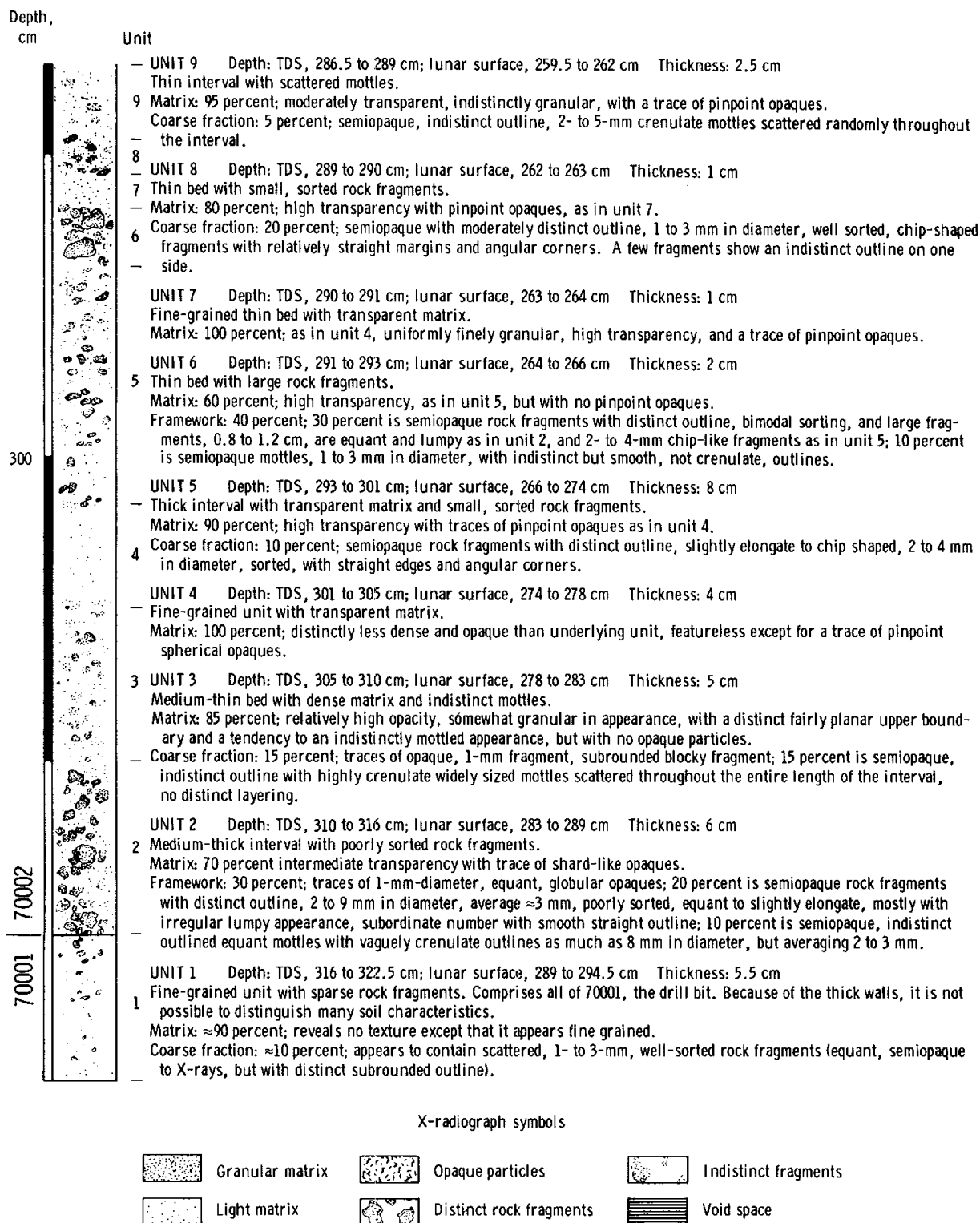
FIGURE 7-27.—Interpretation of X-radiographs of Apollo 17 deep drill string. The top of the drill string is represented by the abbreviation TDS. Depth values are direct from X-radiographs and therefore are somewhat expanded.
