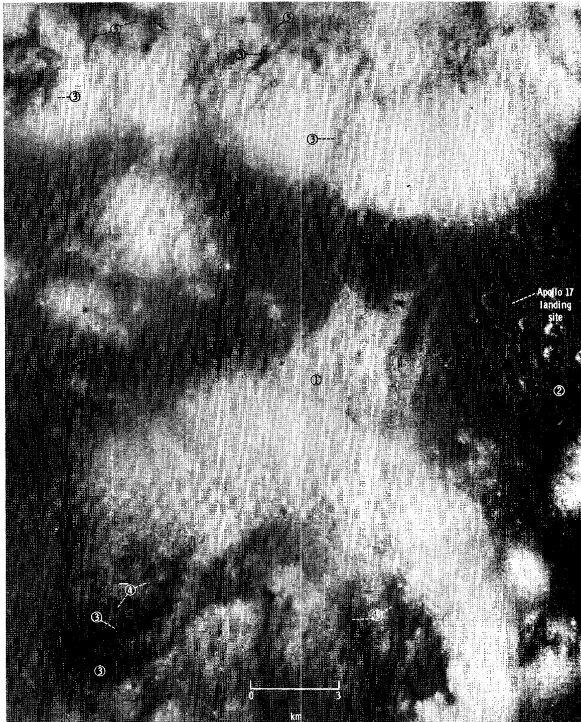
FIGURE 29-18.—Apollo 17 landing site area. (1) Bright mantle overlying dark mantle; (2) cluster of craters of middle-Copernican age; (3) dark patches and streaks on steep highland slopes; (4) dark mantle covering bouldery outcrop ledges; and (5) moderately dark mantle material concentrated in lows (Apollo 15 panoramic camera frame AS15-9557).
