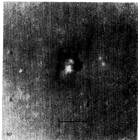
FIGURE 29-22.—Dark-halo craters in Taurus-Littrow region. (a) Dark-halo crater with shape typical of small impact craters (Apollo 15 panoramic camera frame AS15-9559). (b) Dark-halo crater on hill (sloping steeply to upper left). Crater has bright walls and is half filled with dark material (Apollo 15 panoramic camera frame AS15-9559). (c) Dark-halo crater with subdued rim, steep walls, and deep interior (Apollo 15 panoramic camera frame AS15-9559). (d) Very subdued crater with distinct ray-like halo (Apollo 15 panoramic camera frame AS15-9559). (e) Crater with subdued, mantled rim and fresh-looking rocky floor (Apollo 15 panoramic camera frame AS15-9557). (f) Dark patch across crater rim (Apollo 15 panoramic camera frame AS15-9559). (g) Dark patch on crater rim; dots outline rim crest (Apollo 15 panoramic camera frame AS15-9559).
