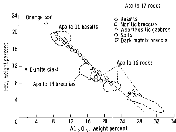
FIGURE 7-21.—The FeO and \text{Al}_2\text{O}_3 variation in Apollo 17 rocks and soils compared with data from previous missions.
