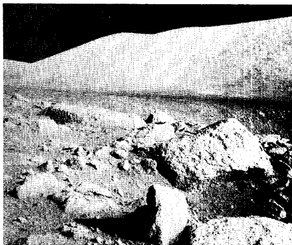
FIGURE 6-42.—North-looking photograph of part of station 5 area showing tabular basalt boulders on southwest rim and inner wall of Camelot Crater. Prominent banding is visible in large block in right near field (AS17-145-22178).
