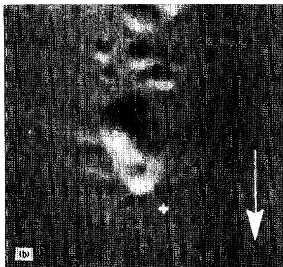
FIGURE 32-17.—Groups of secondary craters near Copernicus Crater. Locations of parts are shown in figure 32-16. Arrows point toward Copernicus Crater. (a) Crater chain showing V-shaped ridges (Lunar Orbiter IV frame H-121). (b) Crater pair with subdued ridges (Lunar Orbiter IV frame H-114). (c) Crater pair with subdued ridges (Lunar Orbiter IV frame H-121). (d) Six crater pairs with prominent ridges (Lunar Orbiter IV frame H-121).
