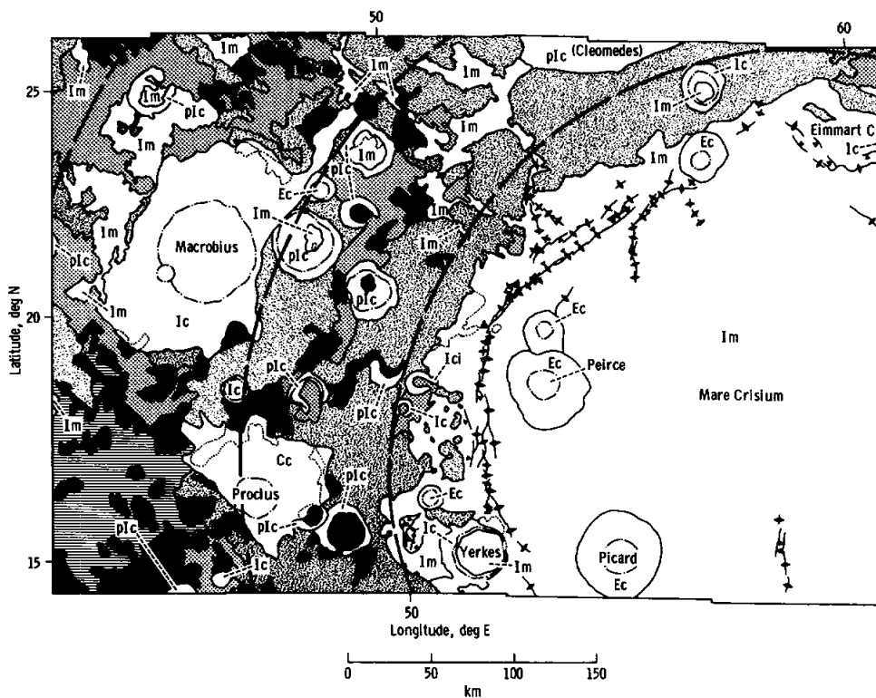
FIGURE 29-27.—Geologic map of northern Crisium region, based on photomosaic of figure 29-26. Detailed description of map units is listed separately.
