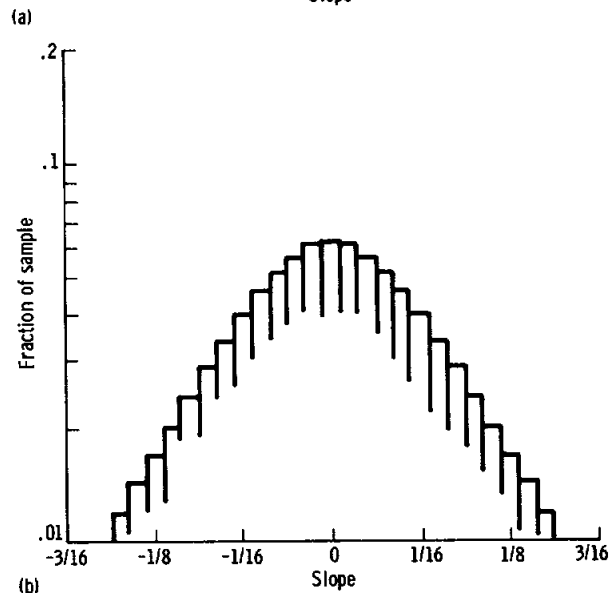
FIGURE 33-16.—Histograms illustrating effect of reading error on hypothetical exponential slope-frequency distribution. Note difference in peakedness of the two distributions. (a) Starting hypothetical distributions. (b) Apparent distribution produced by reading error.
