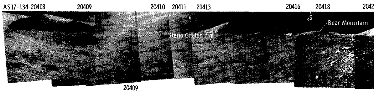
FIGURE 6-101.—Panoramic view taken east of station 1.
