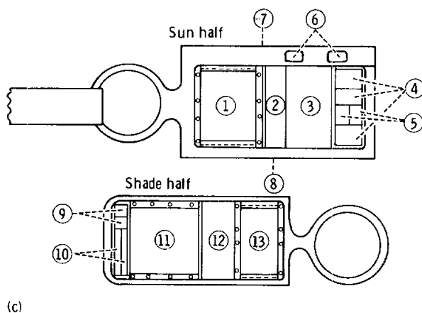
FIGURE 19-1.—The LSCRE. (a) View of interior. (b) View of exterior. (c) Schematic diagram. For information on numbered detectors, see table 19-I.
