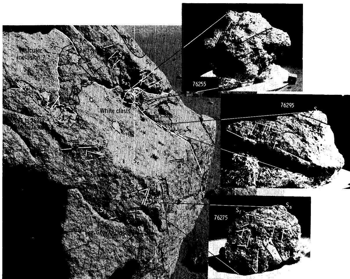
FIGURE 6-23.—Locations of samples removed from boulder 1 at station 6. Known orientations are shown in insets. Heavy solid lines indicate traces of shear planes, S_a through S_g . Dashed lines outline inclusions and samples. A and B denote fracture surfaces bounding boulder (AS17-140-21443) (inset photographs, S-73-19375, 19387, and 19385, respectively).
