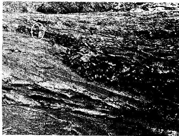
FIGURE 31-19.—Alae lava lake, Hawaii. Compressional ridge at buckled toe of thrust fault in subsiding crust of lava lake; man circled for scale (ref. 31-19).
