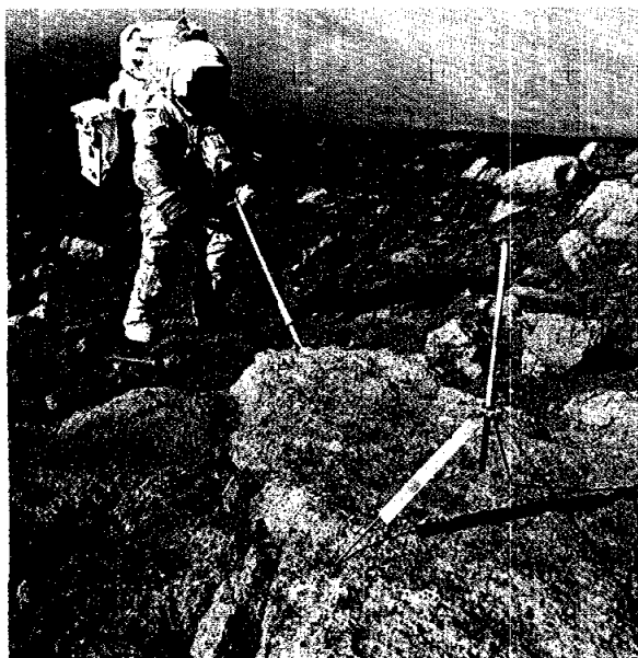
FIGURE 4-31.—The LMP uses the scoop to collect a sample at station 5. The high density of boulders along the rim of Camelot Crater is shown in this photograph (AS17-145-22157).
