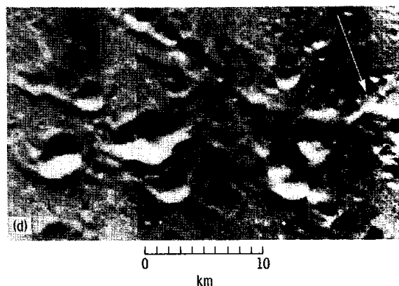
FIGURE 32-17.—Groups of secondary craters near Copernicus Crater. Locations of parts are shown in figure 32-16. Arrows point toward Copernicus Crater. (a) Crater chain showing V-shaped ridges (Lunar Orbiter IV frame H-121). (b) Crater pair with subdued ridges (Lunar Orbiter IV frame H-114). (c) Crater pair with subdued ridges (Lunar Orbiter IV frame H-121). (d) Six crater pairs with prominent ridges (Lunar Orbiter IV frame H-121).
