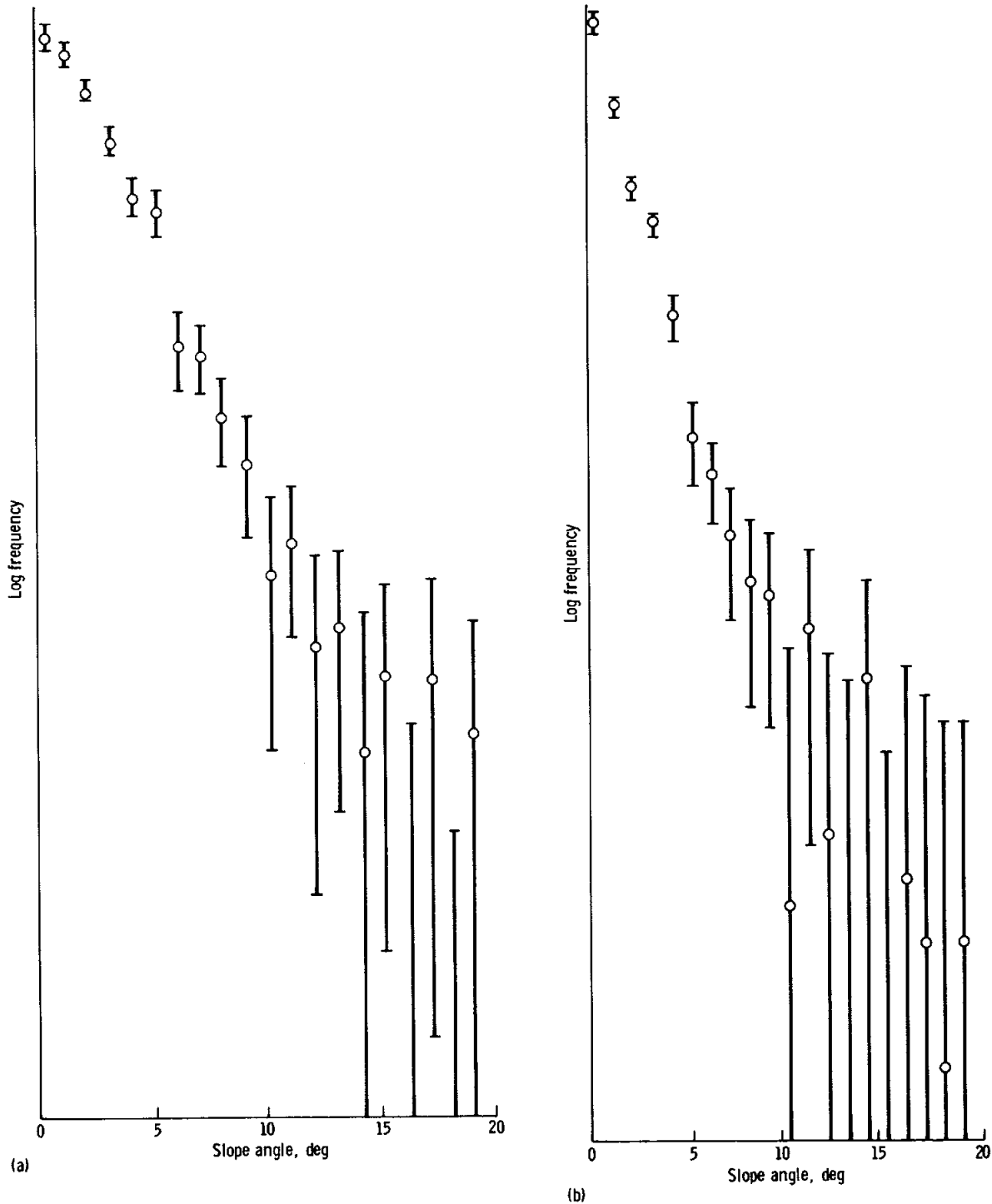
FIGURE 33-13.—Incremental slope-frequency distributions inferred from 13- and 116-cm bistatic-radar data for a region in central Mare Serenitatis. (a) 13-cm data (lat. 20.1^{\circ} N, long. 27.2^{\circ} E). (b) 116-cm data (lat. 20.2^{\circ} N, long. 26.9^{\circ} E).
