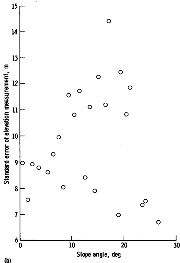
FIGURE 33-22.—Standard errors for elevation measurements and absolute slope angle. (a) Stereomodel 1 with Sun elevation angle of 16.5^\circ (from Apollo 17 metric camera frames AS17-0446 and 0447). (b) Stereomodel 2 with Sun elevation angle of 30.5^\circ (from Apollo 17 metric camera frames AS17-1499 and 1500). (c) Stereomodel 3 with Sun elevation angle of 50.5^\circ (from Apollo 17 metric camera frames AS17-2086 and 2087).
