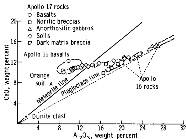
FIGURE 7-22.—The \text{CaO} and \text{Al}_2\text{O}_3 variation in Apollo 17 rocks and soils compared with Apollo 16 and 11 rocks.
