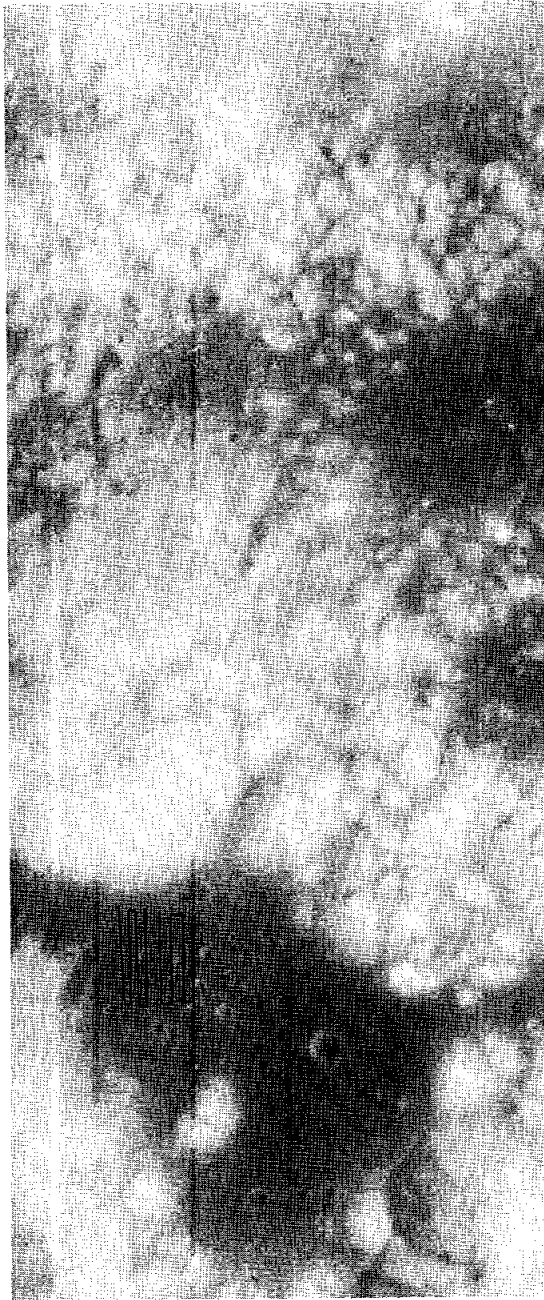
FIGURE 33-19.—Apollo 17 panoramic photograph showing traverse lines for slope-frequency distributions. Traverse to right is for the landing site; traverse to left is westward of landing site.
