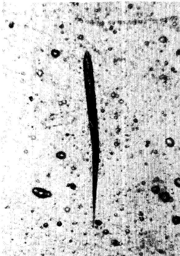
FIGURE 25-7.—Etch cone of a scattered HZE particle (approximately 750 μm long) in Daicel-71 CN.
