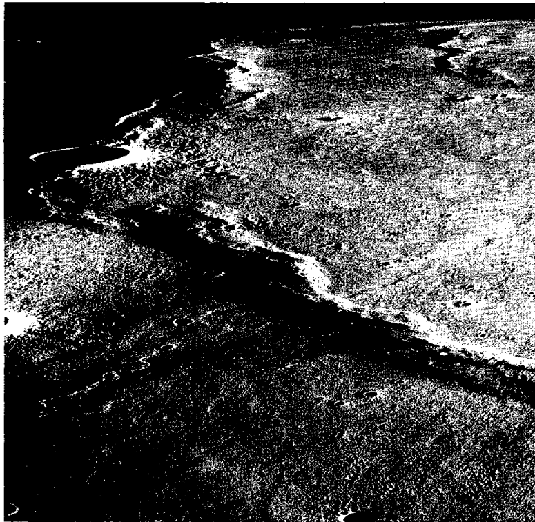
FIGURE 4-51.—Near-terminator photograph in Mare Imbrium. The very low angle of Sun illumination emphasizes topographic detail in this north-looking, high-oblique view of the crater C. Herschel and associated mare ridges. C. Herschel, approximately 15 km in diameter, is located at latitude 34.5^{\circ} N, longitude 31^{\circ} W (AS17-155-23712).
