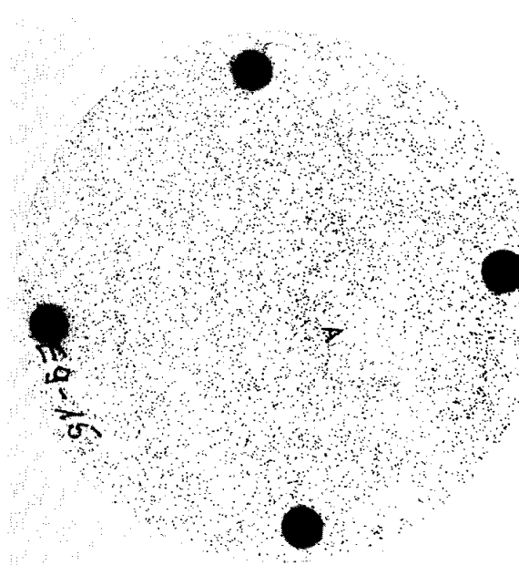
FIGURE 25-2.—A biologic layer of the biostack II flight unit consisting of Artemia salina eggs embedded in a foil of polyvinyl alcohol.
