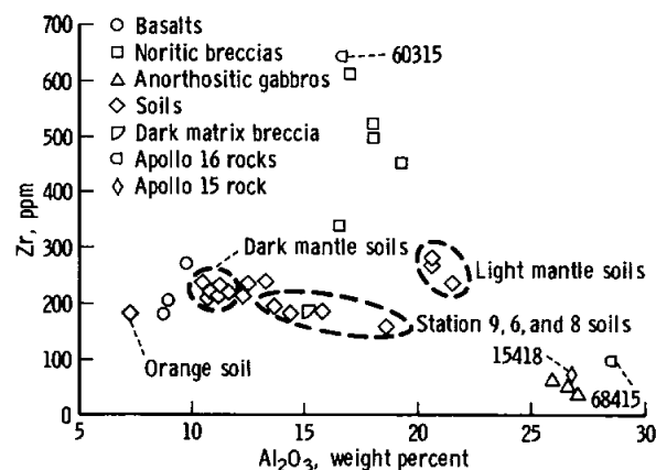
FIGURE 7-24.—The \text{Al}_2\text{O}_3 and Zr variation in Apollo 17 rocks and soils. Data for previous missions were taken from references 7-9 and 7-10.
