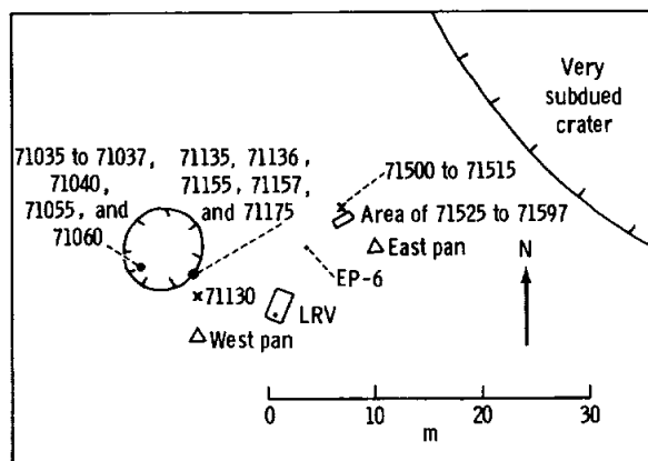
FIGURE 6-102.—Planimetric map of station 1.
