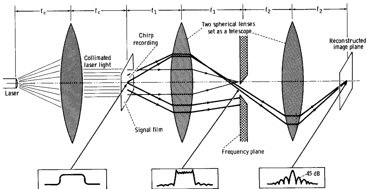
FIGURE 22-9.—Schematic illustration of optical setup. Focal distances are designated f_1 , f_2 , and f_c .
