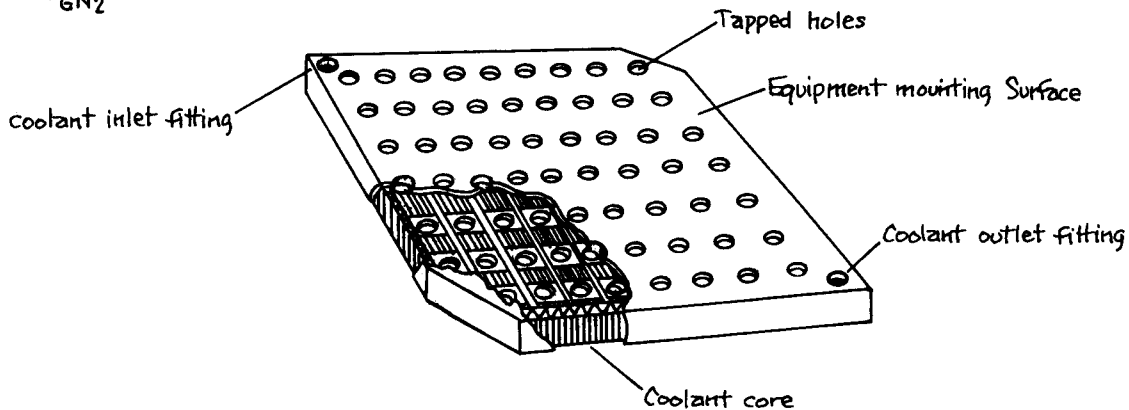
Typical Coldplate
