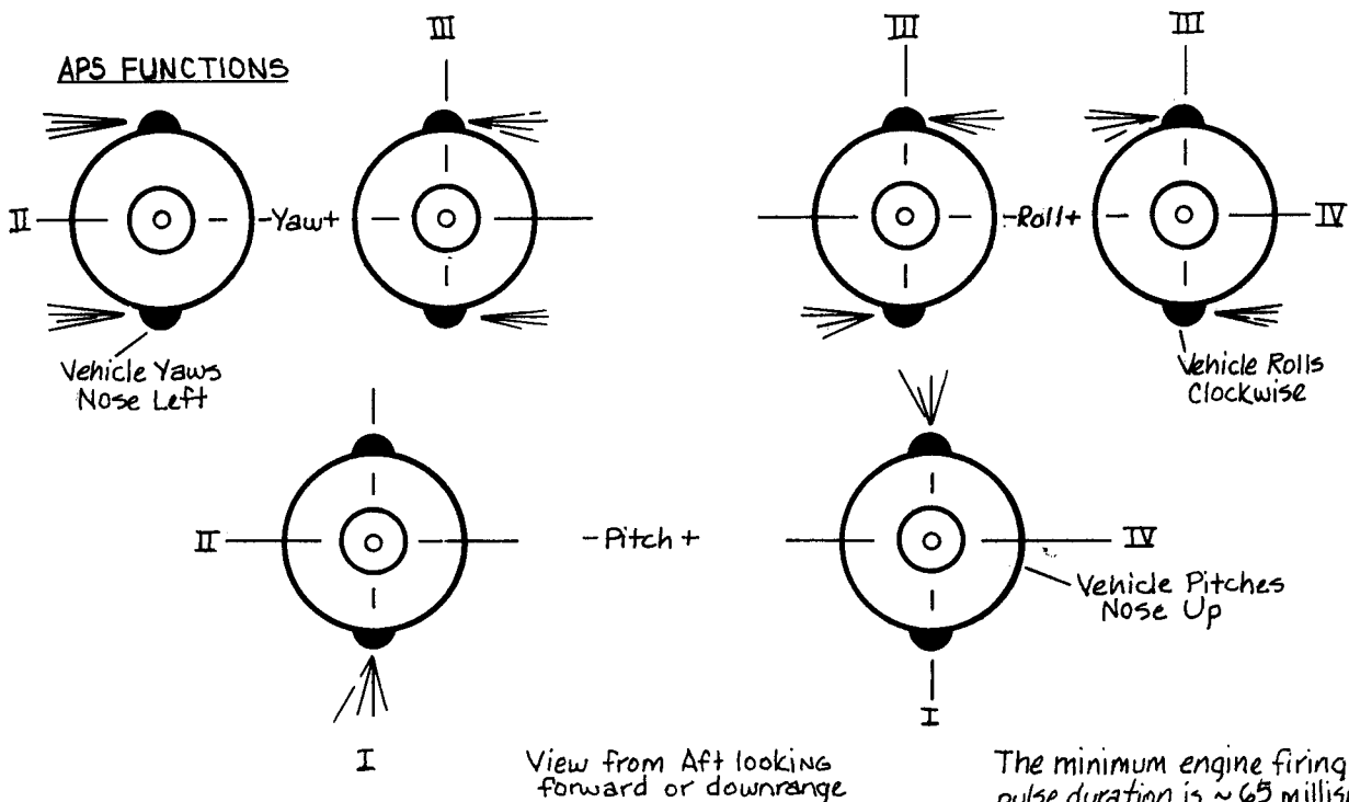
S-IVB Auxiliary Propulsion System
