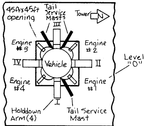
Engine/Holddown Arm/ Tail Service Mast Orientation
