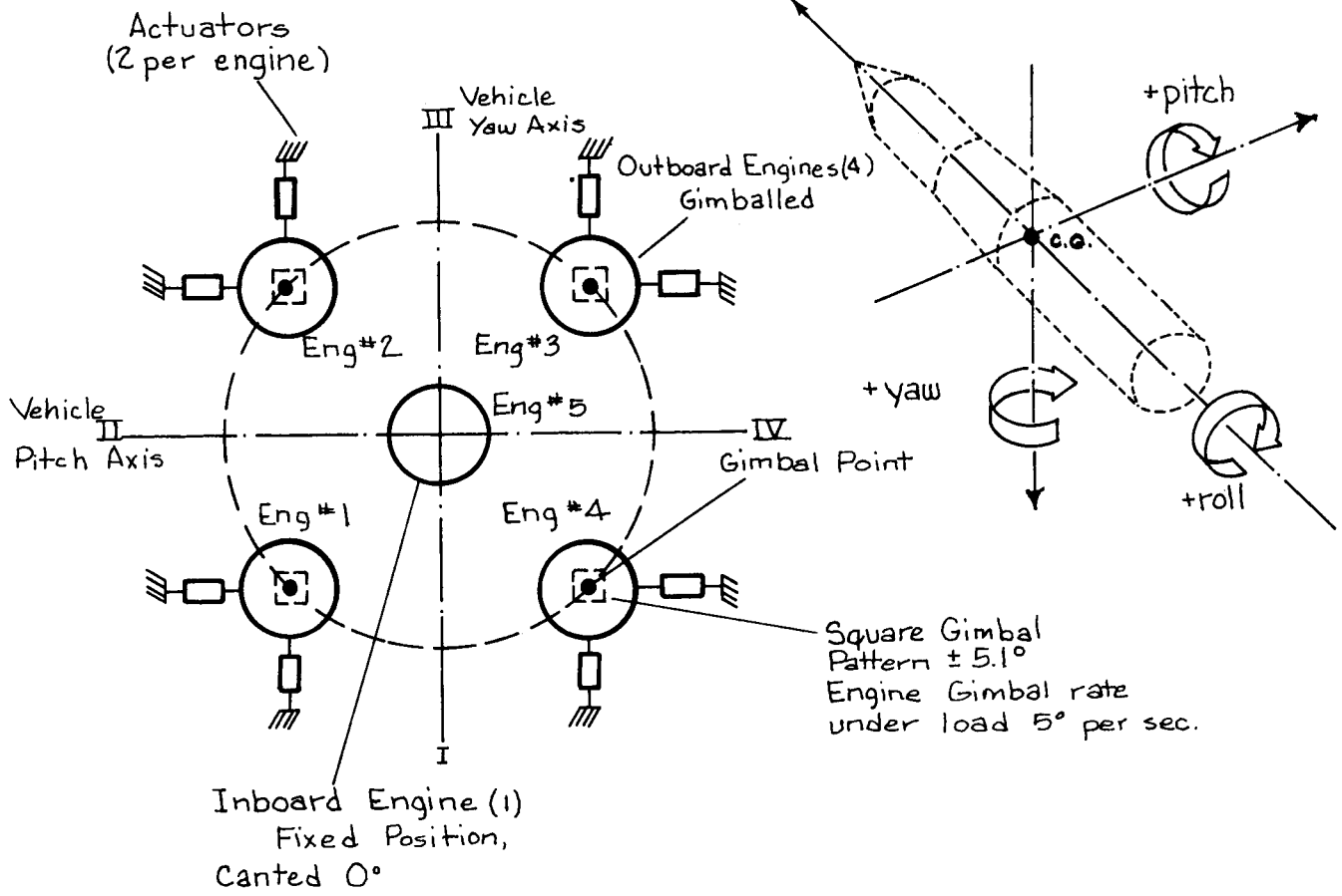
5-IC Thrust Vector Control System
