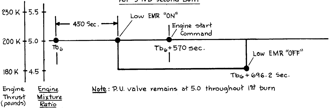
S-IVB Propellant Utilization (P.U.) Timeline For S-IVB Second Burn
