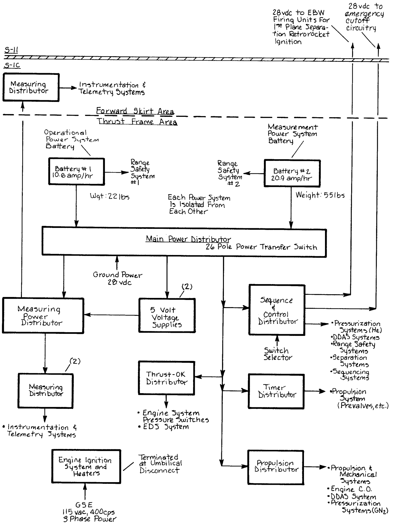
S-1C Electrical Power & Distribution System
