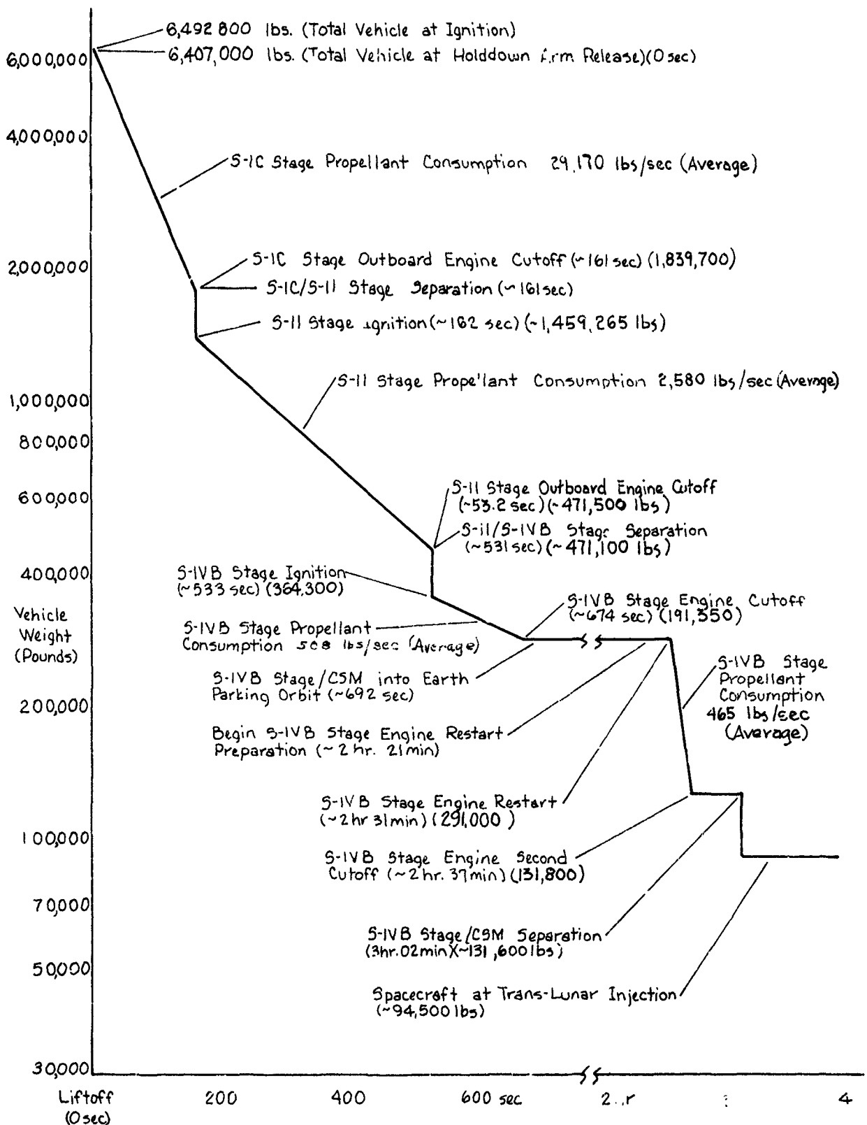
Space Vehicle Weight vs. Flight Time
