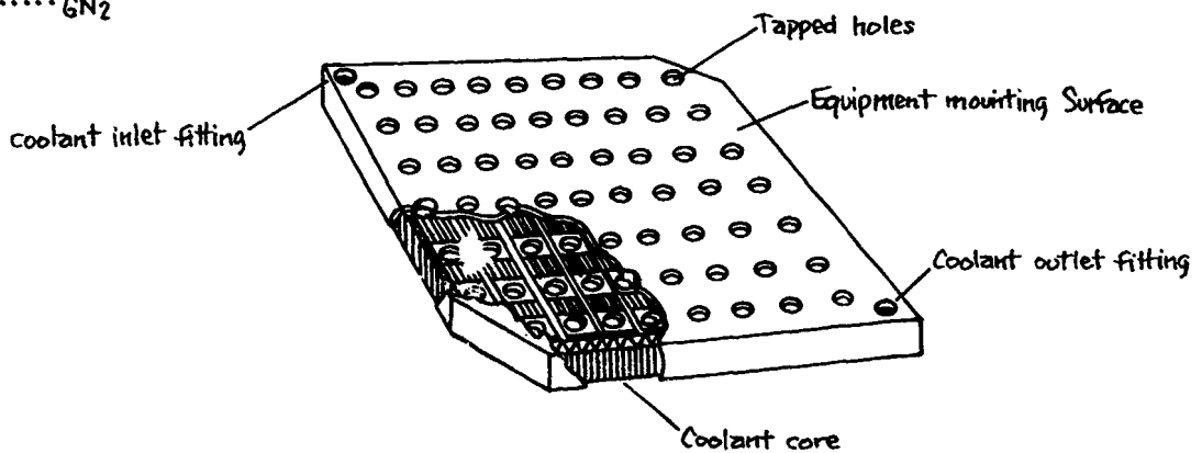
Typical Coldplate
