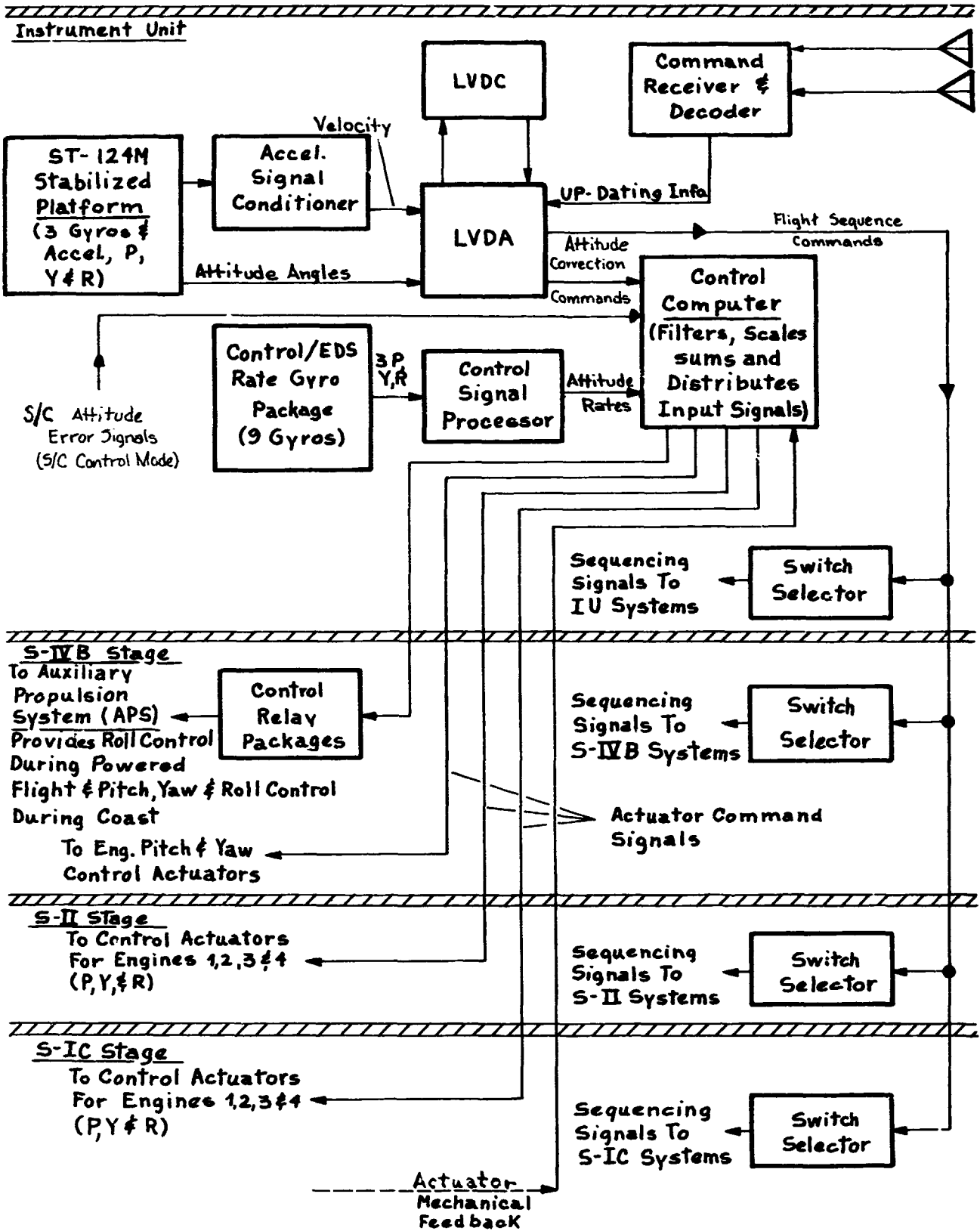
Guidance and Control System Block Diagram
