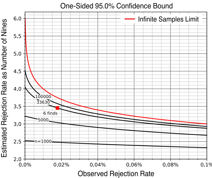
Figure 2 95% confidence upper bound on risk as a function of total inspections and proportion of rejections
