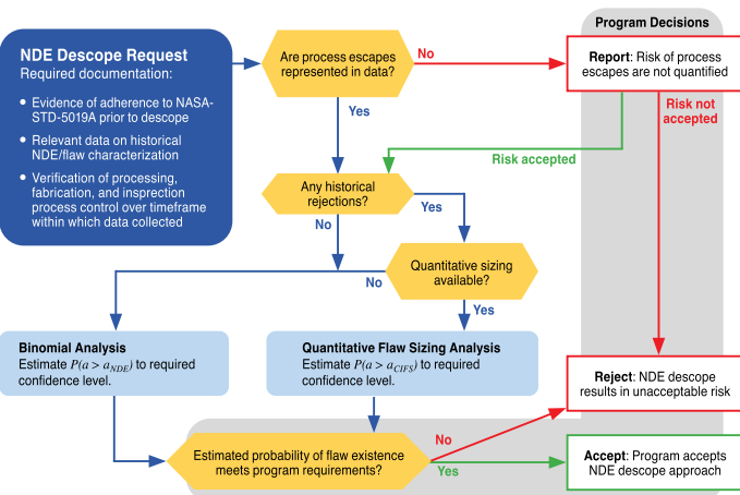
Figure 3 Flowchart of the proposed approach for assessing risk associated with NDE descscope
