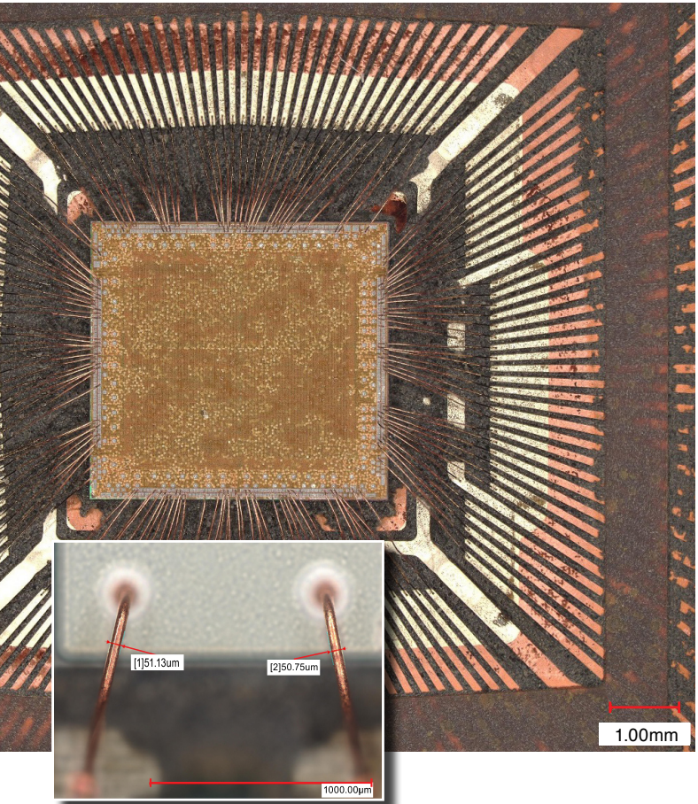
Example of copper wire bonds.
