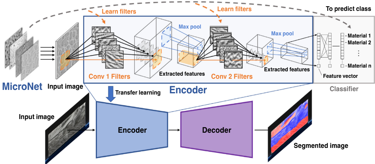
The team eliminated issues with manual identification of LTA by training a neural network to detect LTA from images of fracture surfaces, pretraining an encoder on a large NASA dataset of microscopy images called MicroNet.
