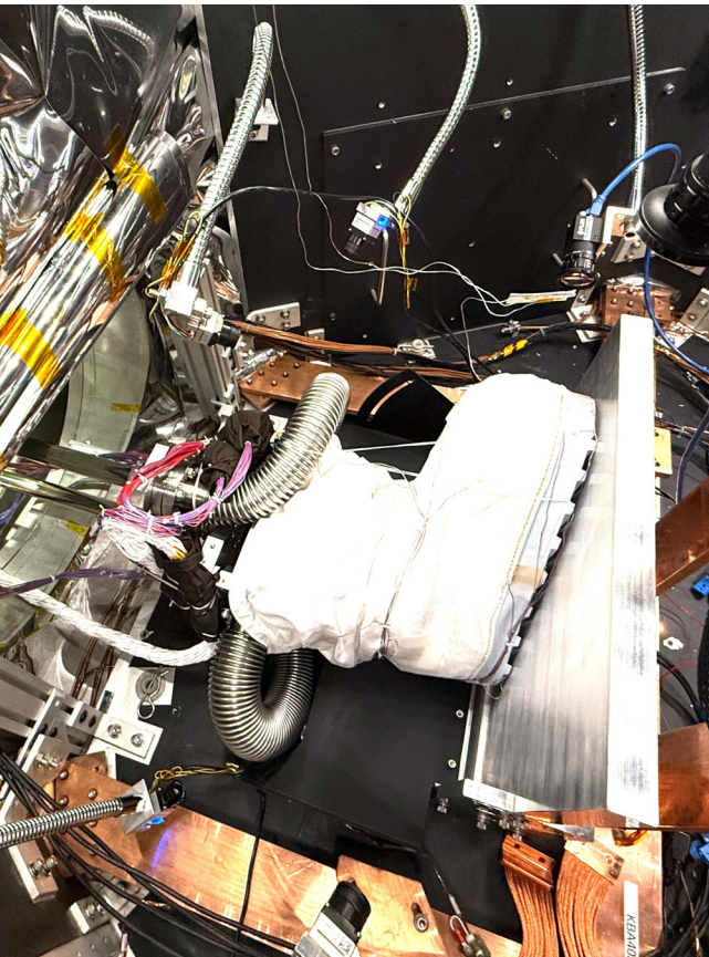
A boot that's part of a NASA lunar surface spacesuit prototype is readied for testing inside a thermal vacuum chamber called CITADEL at the agency's Jet Propulsion Laboratory. The thick aluminum plate at right stands in for the frigid surface of the lunar south pole, where Artemis III astronauts will confront conditions more extreme than any previously experienced by humans.
