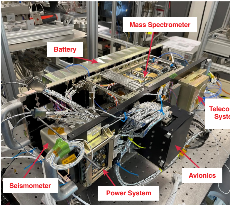
LEMS engineering unit during integration at Goddard. This LEMS prototype incorporates a compact mass spectrometer provided by Goddard and a broadband seismometer provided by the University of Arizona. The unit’s avionics manage its power and thermal states and initiate monthly communication sessions with ground stations on Earth to transmit collected data.
