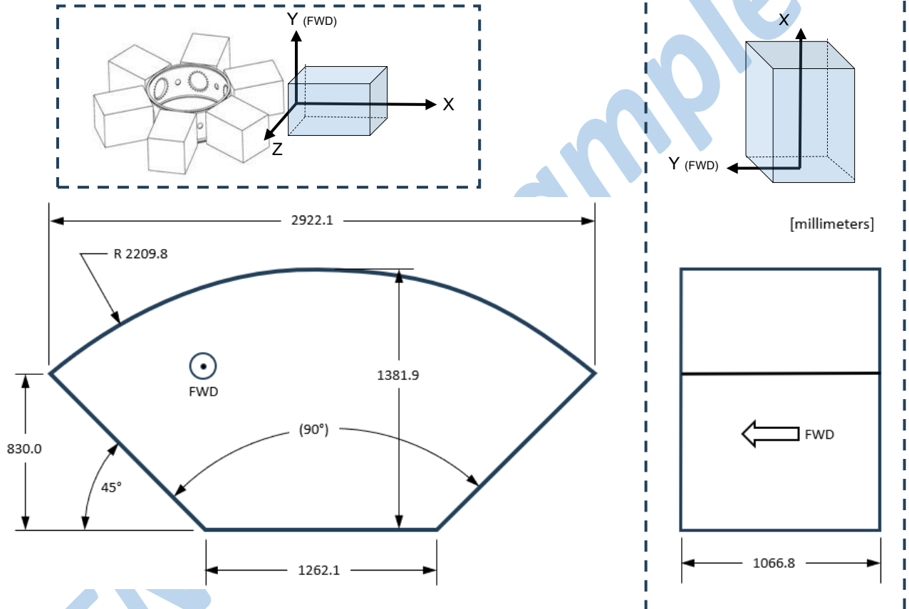
Figure 6.1 SPA and RPL Coordinate System
