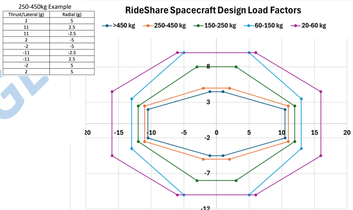
Figure 6.2 Side Mounted Design Load Factors
