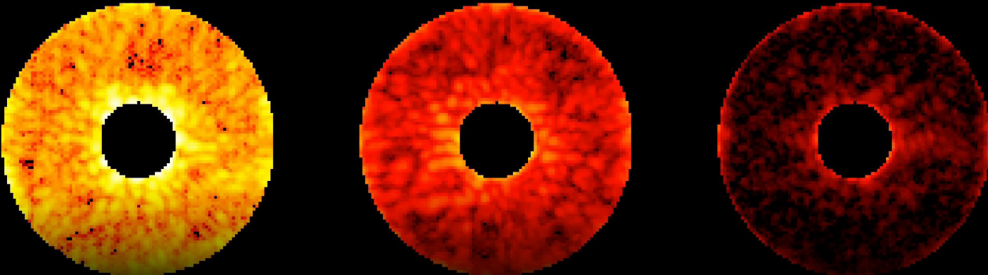
Image Caption: Three computer readouts display data from tests of the Roman Coronagraph Instrument, showing how starlight is progressively reduced using fixed masks and deformable mirrors. The arrangement demonstrates how adjustable optics can suppress stray light to reveal faint planets otherwise hidden by the glare of their parent stars. Credits: NASA/JPL-Caltech
