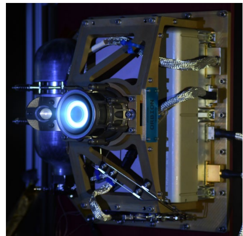
Figure 4.39: Aurora HET, PPU and XFC. Credit: Orbion Space.
