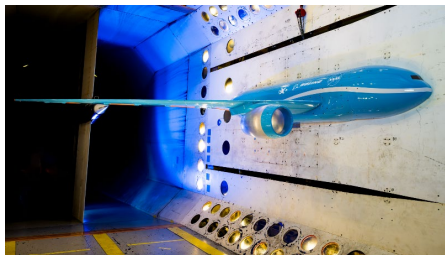
Shown here is the Integrated Adaptive Wing Technology Maturation wind-tunnel model installed in the Transonic Dynamics Tunnel at NASA LaRC in Hampton, Virginia.
