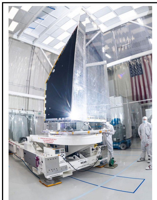
The photo above captures the integration and testing of the NEO Surveyor's instrument enclosure at the Space Dynamics Laboratory (SDL), ahead of its scheduled launch in June 2028.
