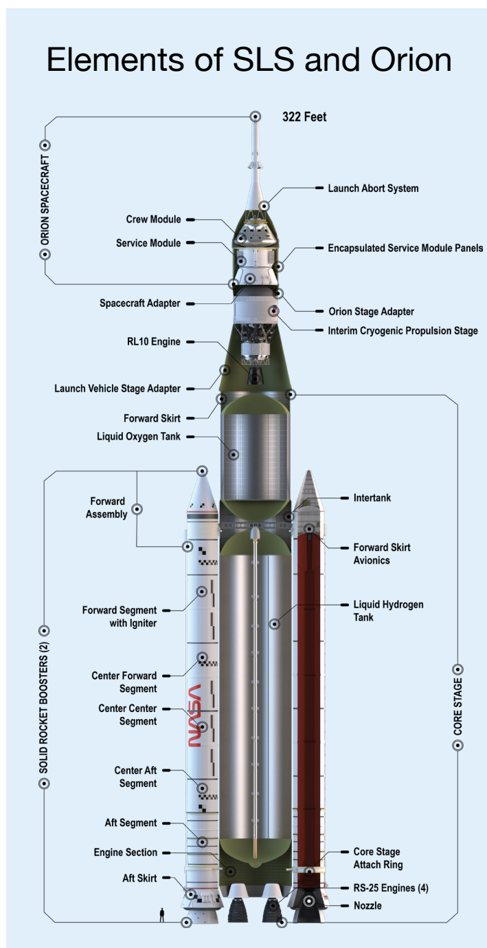
This cutaway illustration identifies the major elements of the SLS and Orion stack. From the ground up, the SLS portion consists of: twin solid rocket boosters with major components labeled, RS-25 liquid-fuel engines, central core stage with propellant tanks and flight computers, launch vehicle stage adapter, ICPS, and Orion stage adapter. Orion is atop SLS. A 6-ft. human figure is shown for comparison in the lower left.
