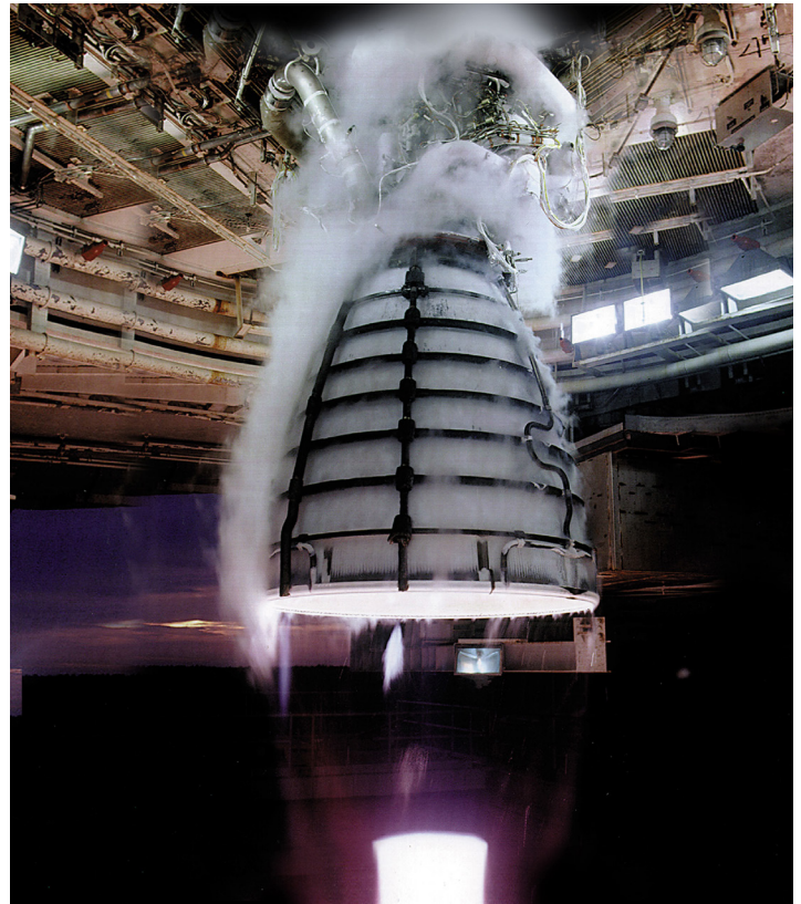
The RS-25s have been upgraded with new controllers that were hot fire tested prior to the Artemis I flight.
