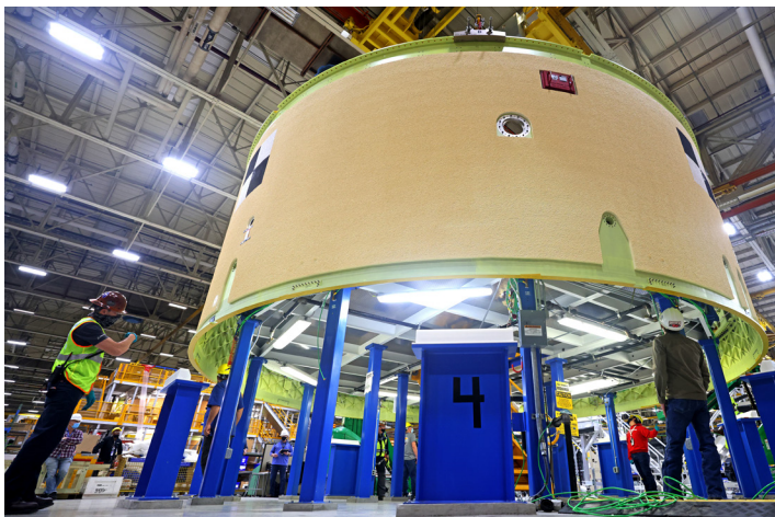
The Artemis II core stage forward skirt is seen here undergoing outfitting at NASA Michoud.
