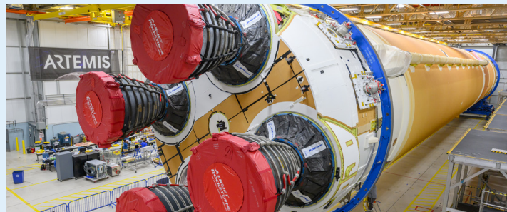
The Artemis II RS-25 engines were installed in the core stage during assembly at NASA's Michoud Assembly Facility in New Orleans.
