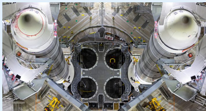
Artemis II five-segment solid rocket boosters were stacked on the mobile launcher at NASA Kennedy.
