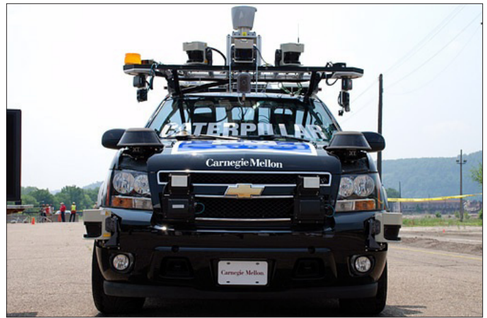
Boss, a self-driving Chevy Tahoe
