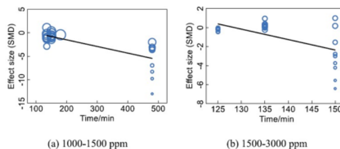
Fig. 6. Subgroup regression analysis of complex cognitive task performance under different exposure durations [8,21-23,29].
