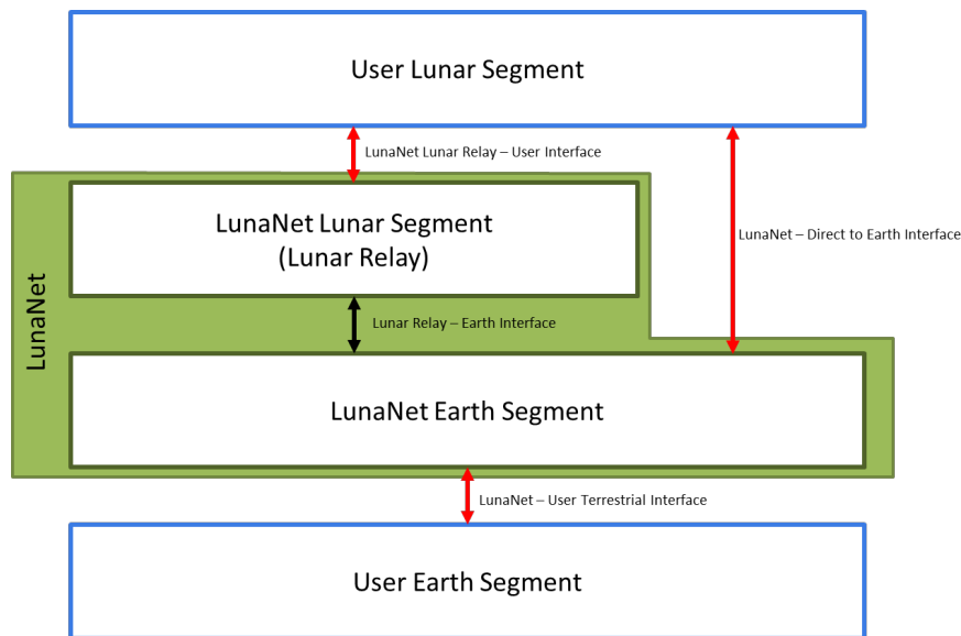
Figure 1 - LunaNet Segments
