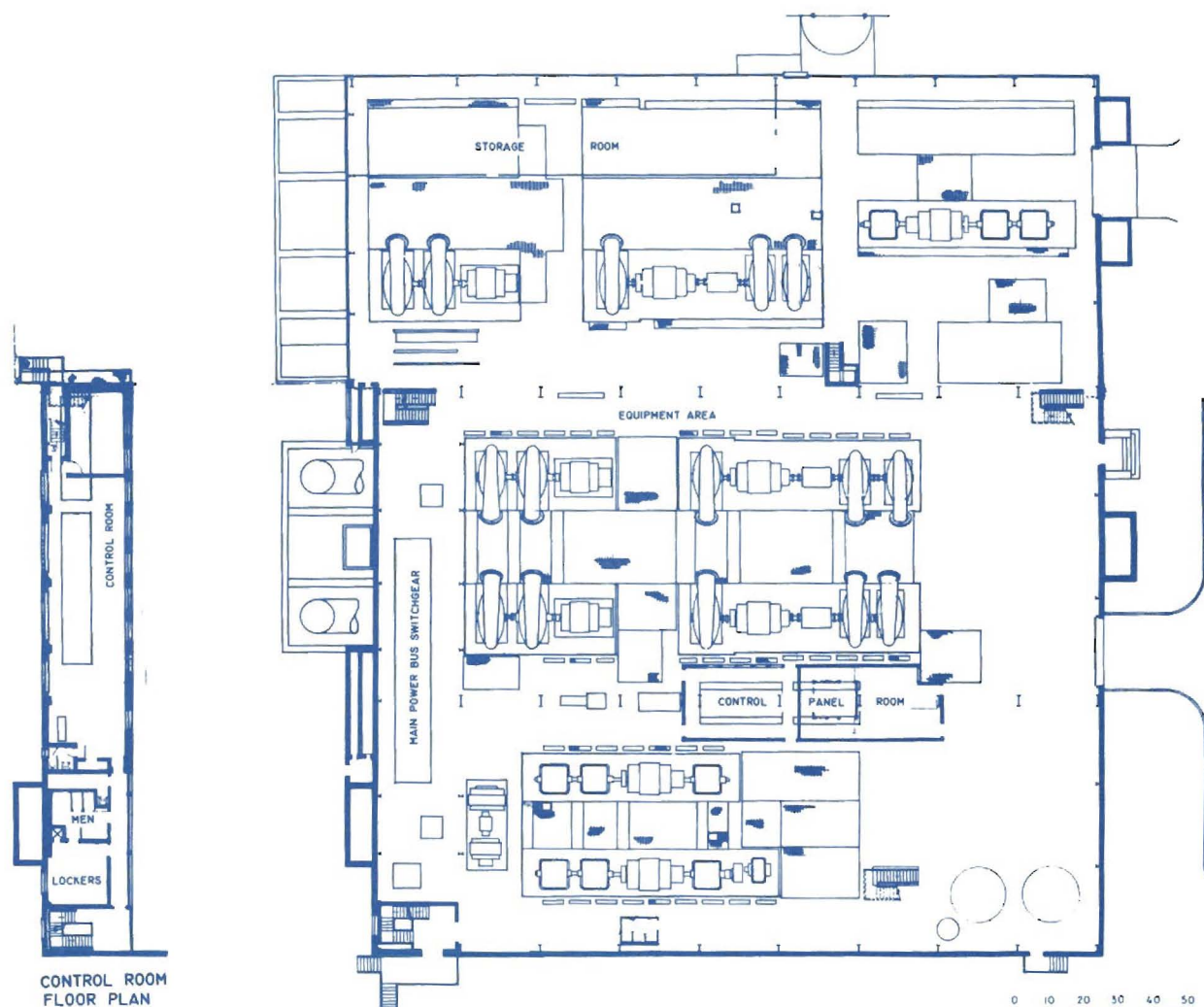
OPERATING FLOOR PLAN
