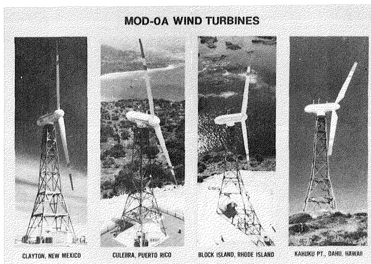
Figure 2. - Mod-0A 200 kW wind turbines.
