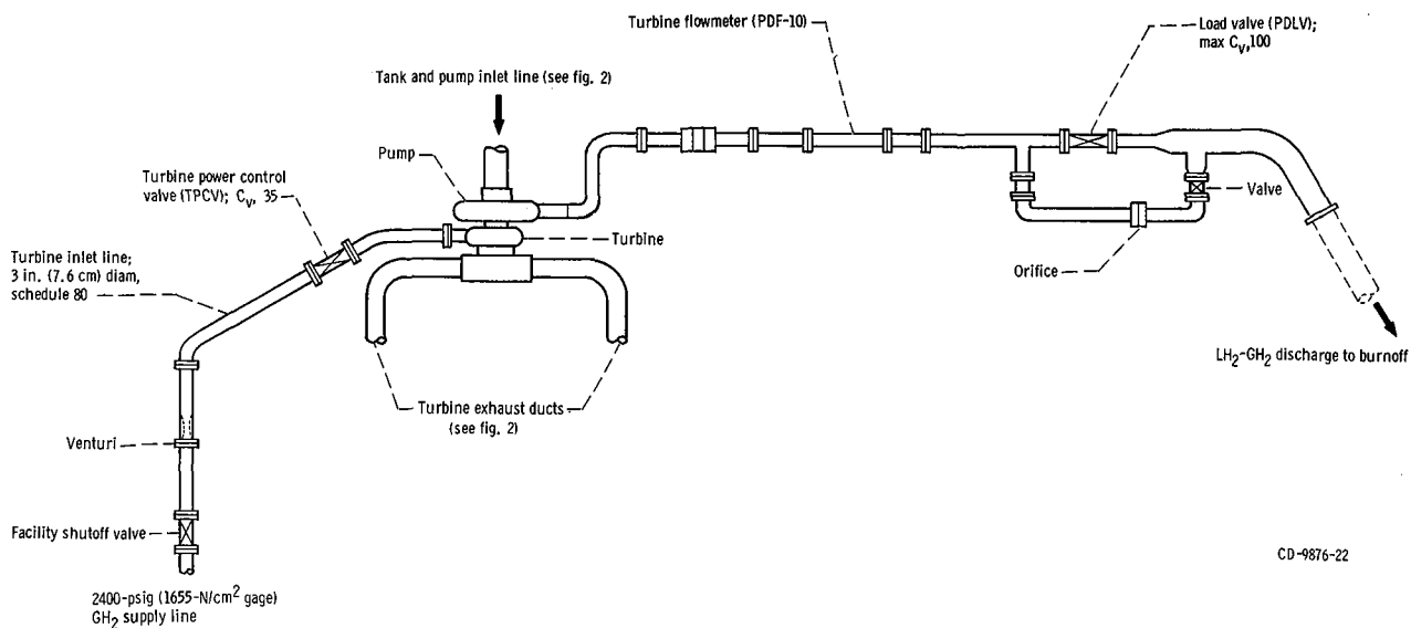
Figure 3. - Low-speed turbopump mapping test piping.
