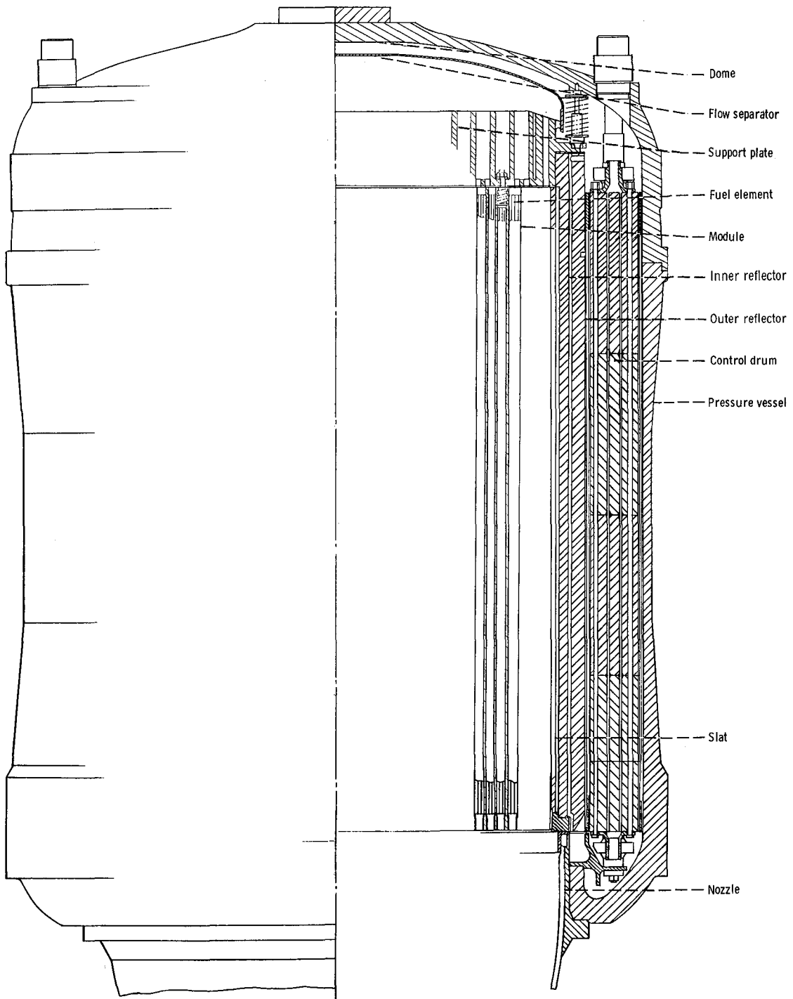
Figure 10. - Schematic diagram of reactor.
