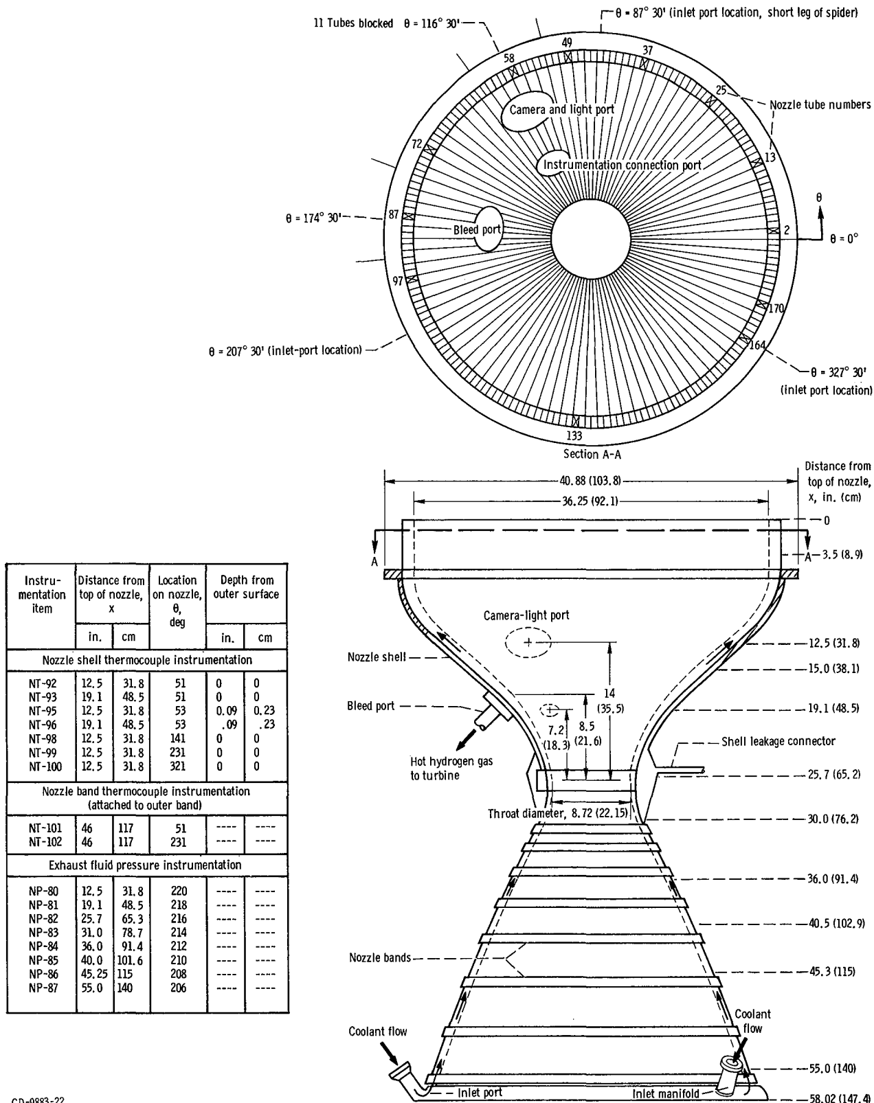
Figure 11. - Nozzle with instrumentation. (Dimensions in inches (cm); instrumentation items identified in table I.)
