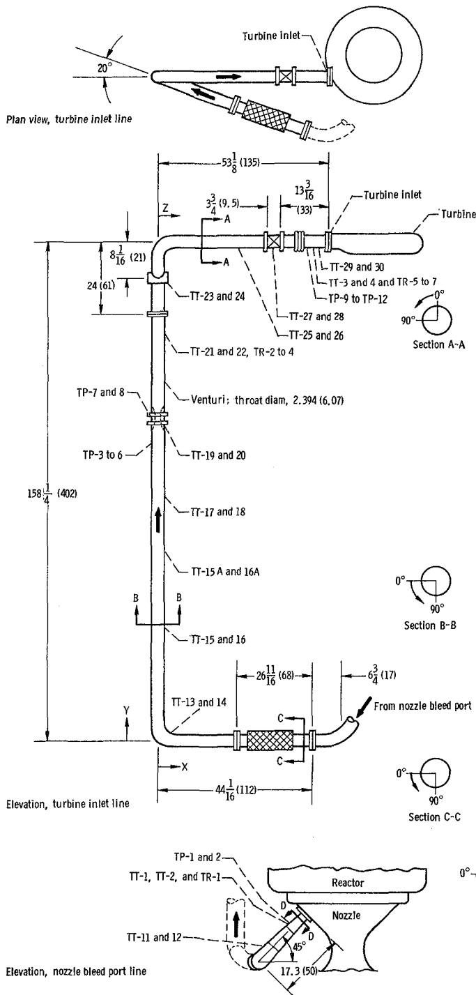
Figure 19. - Turbine inlet line instrumentation, system tests. (Dimensions are in inches (cm); instrumentation items are identified in table I.)
