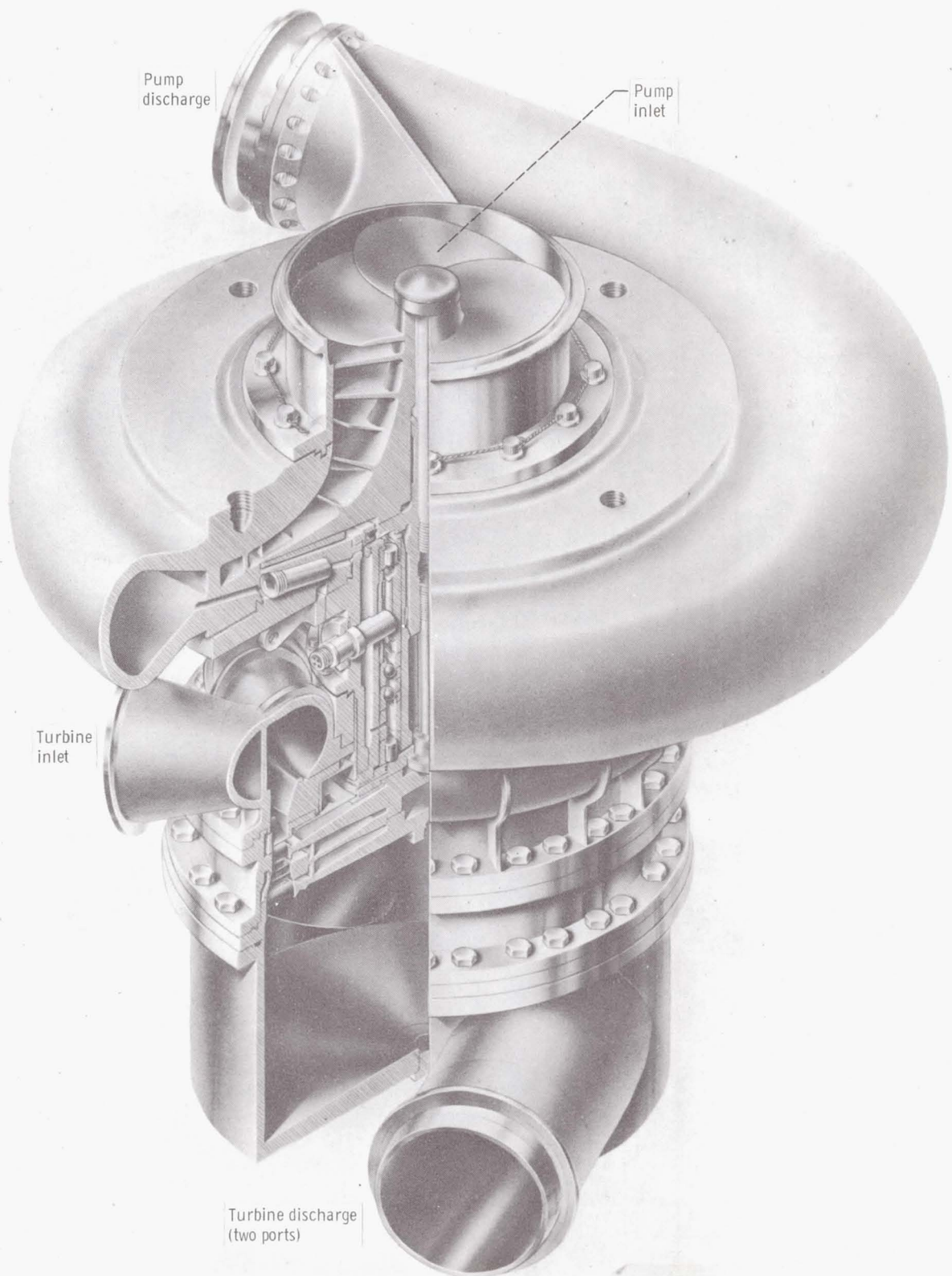
Figure 9. - Mark III, model 4 turbopump.
