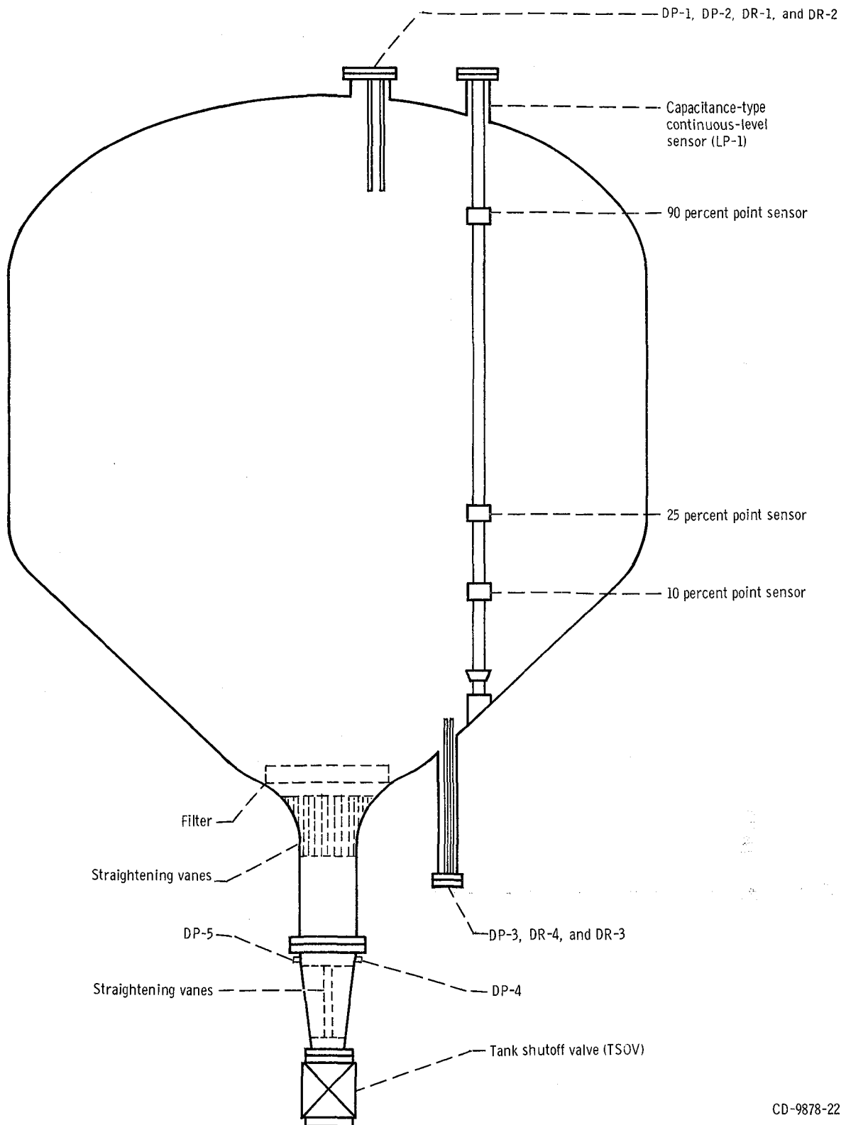
Figure 5. - Liquid-hydrogen run tank. (Instrumentation items identified in table I.)
