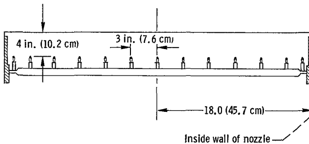
Detail of nozzle chamber thermocouple rake
