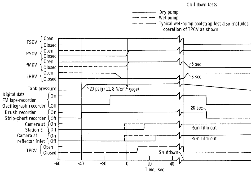
(a) Wet- and dry-pump chiltdown tests.
