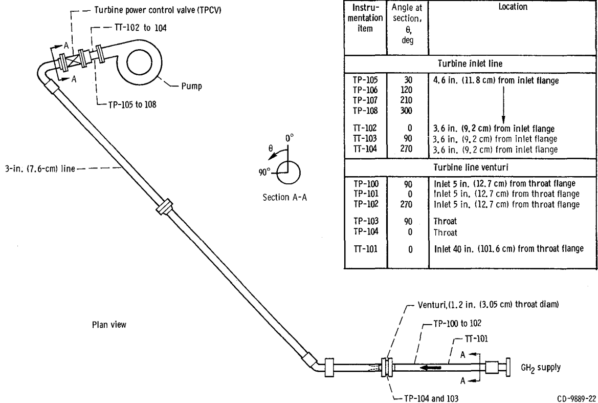
Figure 20. - Turbine inlet line instrumentation, pump tests. (Instrumentation items are identified in table I.)
