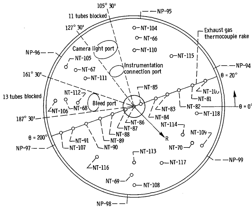
Location of thermocouples in nozzle chamber (section A-A, fig. 11)
