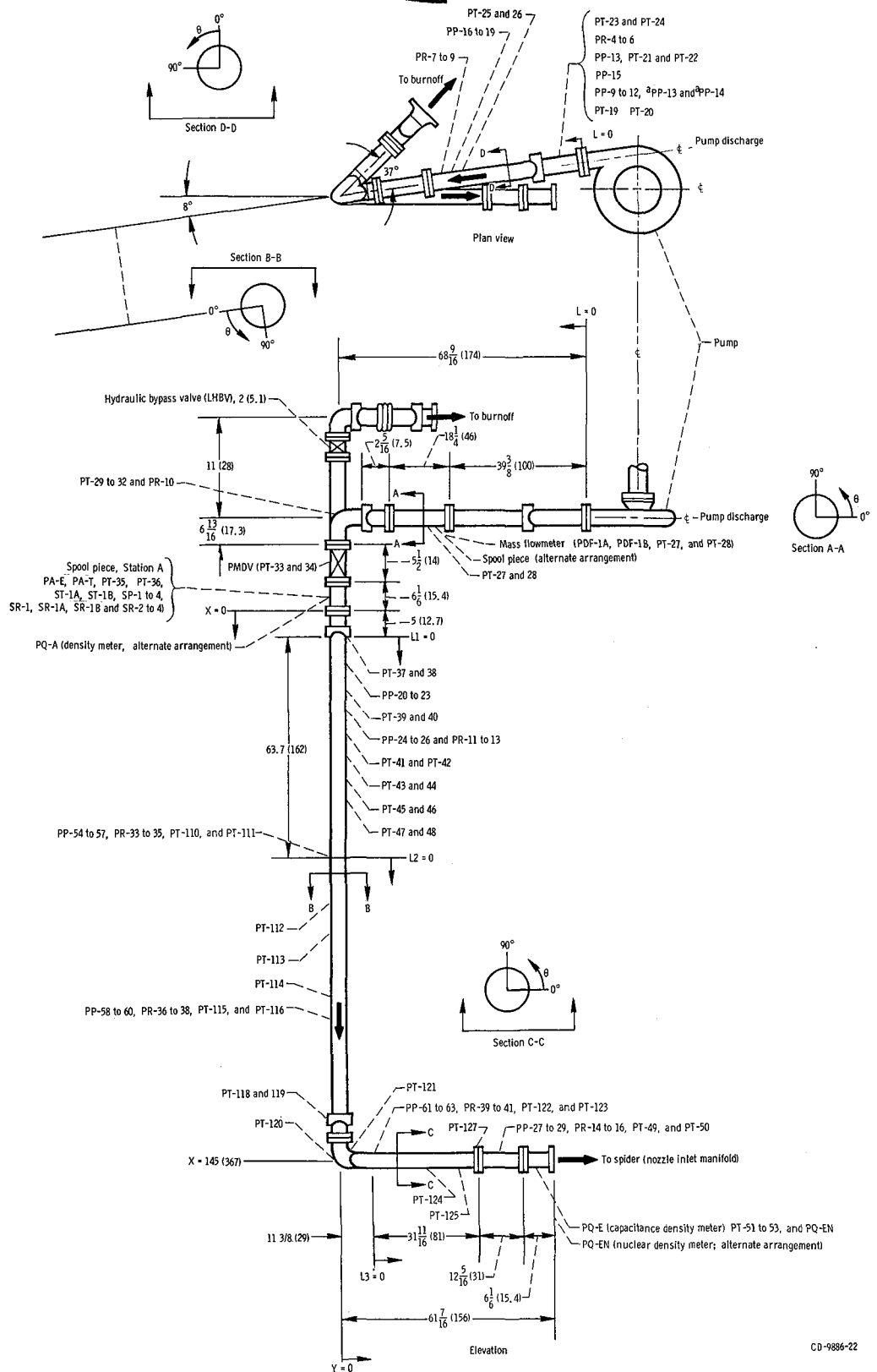
Figure 17. - Instrumentation on pump discharge piping as used on systems tests. On tests in which station E nuclear tance density meter when it was located at Station A. (Dimensions are in inches (cm); instrumentation items are
