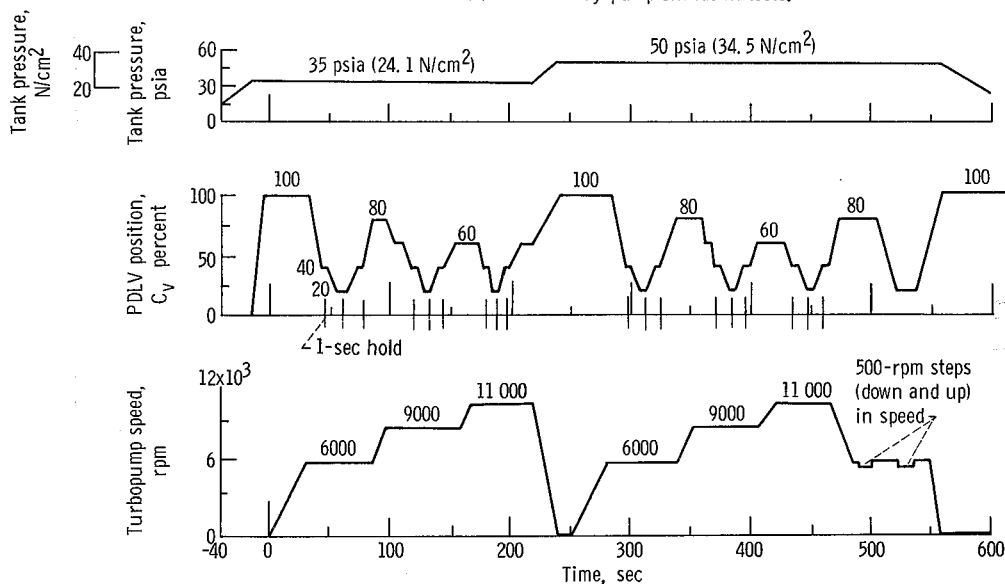
(b) Simplified diagram of pump test.
