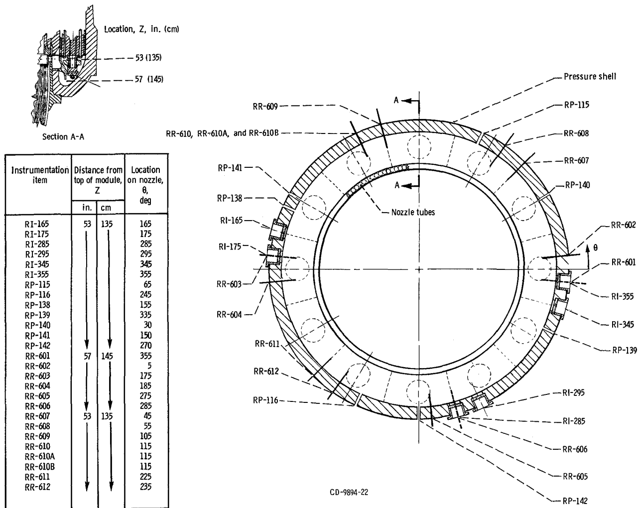
Figure 25. - Reflector inlet plenum instrumentation. (Instrumentation items are identified in table I.)
