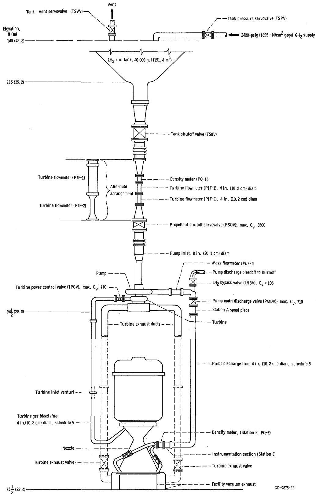
Figure 2 - Full-scale nuclear rocket cold-flow experiment in B-3 facility.
