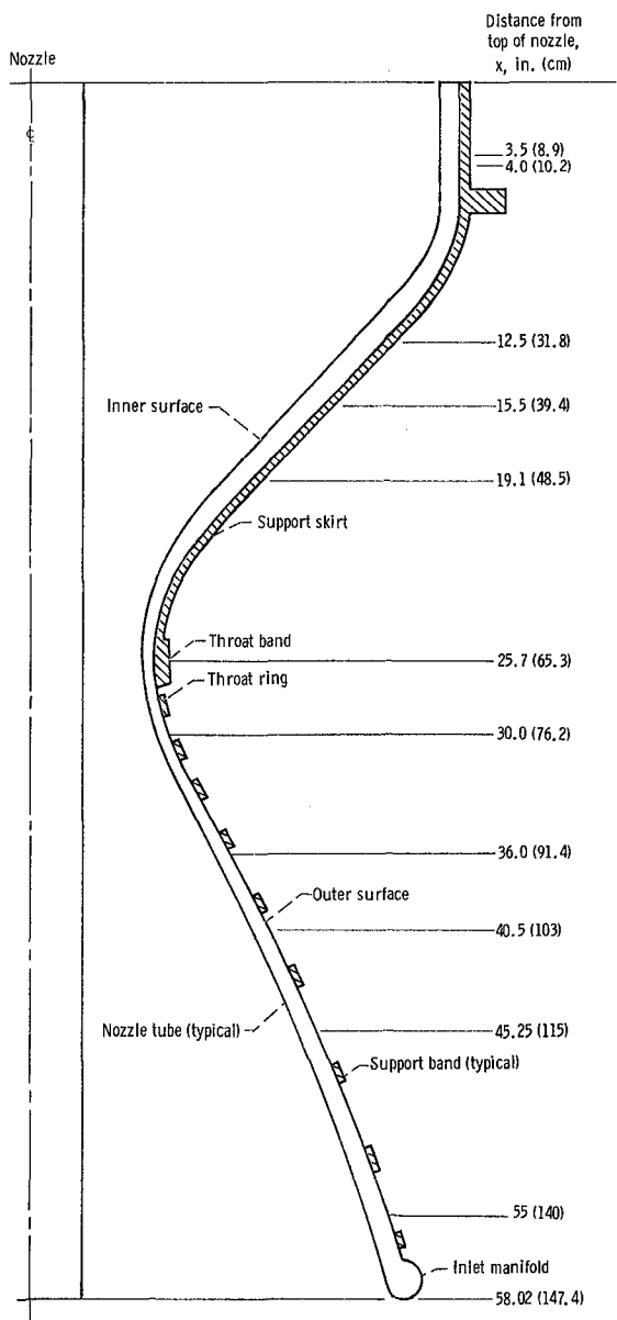
Figure 23. - Nozzle coolant tube instrumentation. (See fig. 11 for coolant tube location; instrumentation items are identified in table I.)
