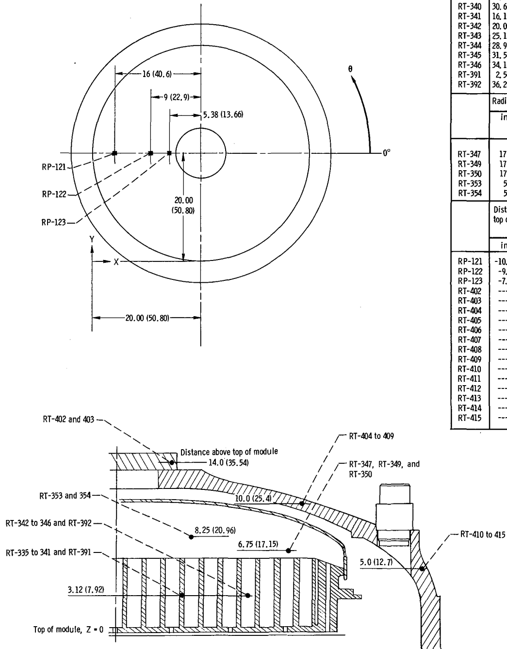
Figure 30. - Dome and core support plate instrumentation. (Dimensions are in inches (cm); instrumentation items are identified in table I.)
