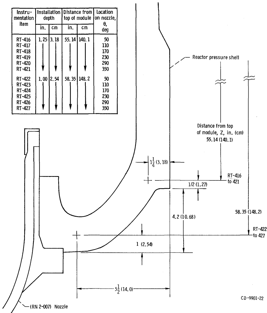
Figure 32. - Reactor pressure shell instrumentation at nozzle end. Copper-constantan thermocouples; thermocouple locations, angle and height, are shown in figure 31. (Dimensions are in inches (cm); instrumentation items are identified in table I.)
