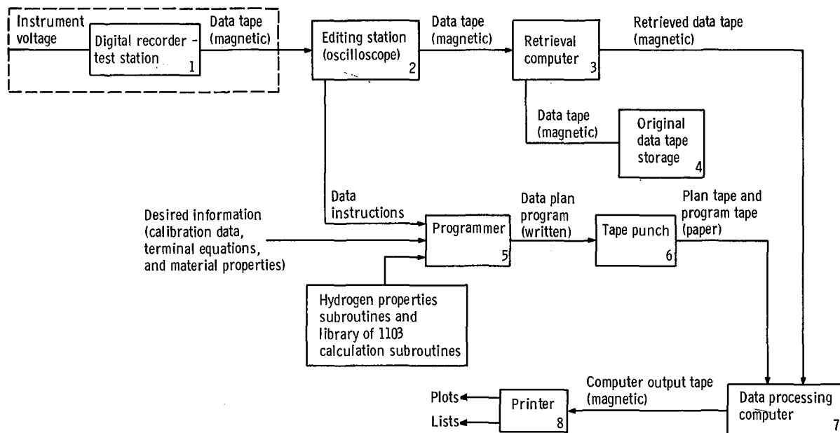
Figure 34. - Schematic diagram of pump tests data processing.
