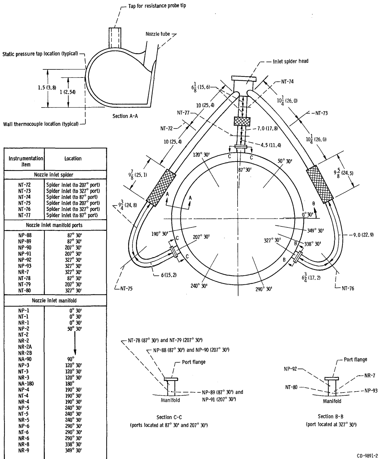
Figure 22. - Nozzle inlet manifold and spider instrumentation. (Dimensions in inches (cm); instrumentation items are identified in table I.)
