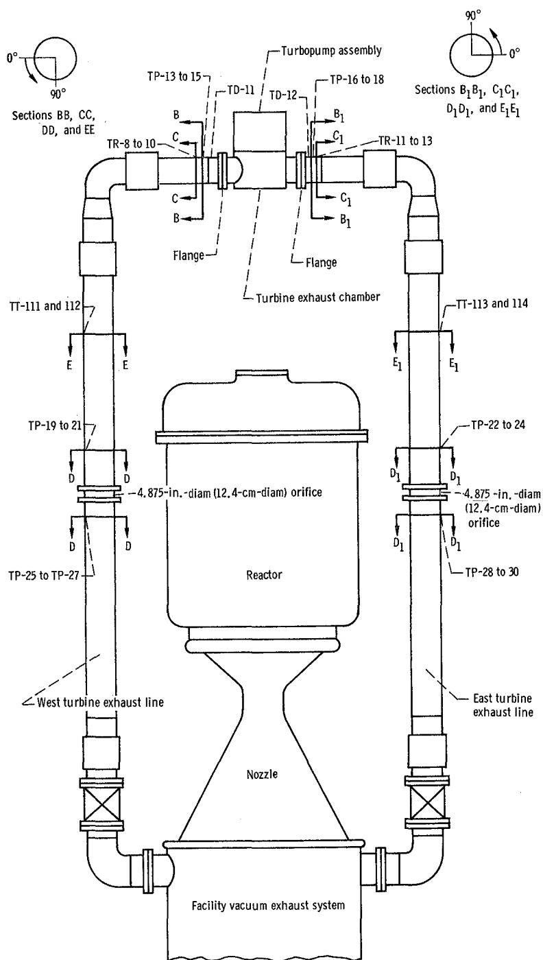
Figure 21. - Turbine exhaust instrumentation, pump and systems tests. (Instrumentation items are identified in table I.)
