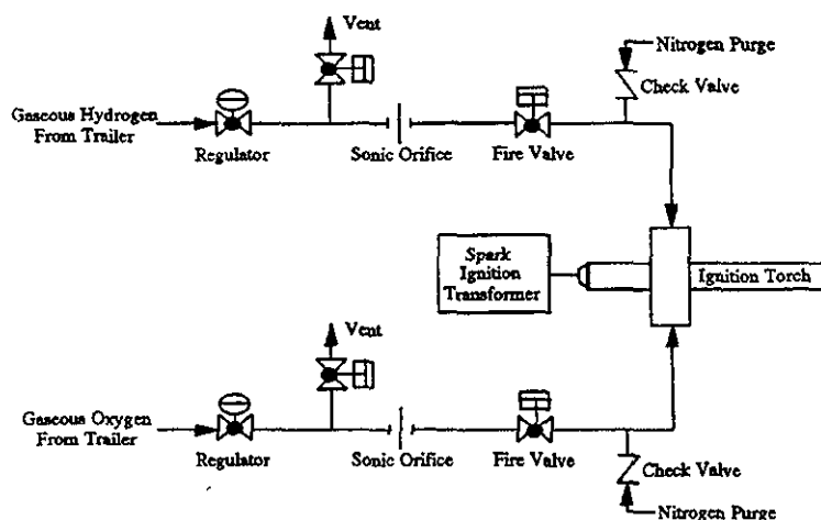
Figure 5: Schematic of the Ignition System
