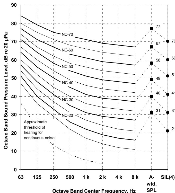
Figure 6.6-1—NC Curves
