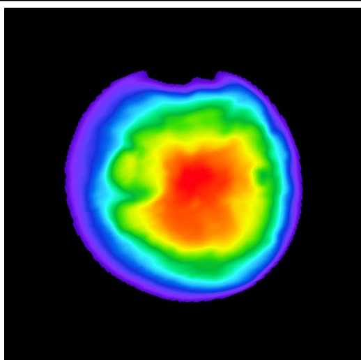
This picture of Mars is a colorized composite of several images captured by Europa Clipper's thermal imager during a flyby of Mars in March 2025. Warm colors represent relatively warm temperatures; red regions are about 32 degrees Fahrenheit (0 degrees Celsius), and purple regions are about minus 190 degrees Fahrenheit (minus 125 degrees Celsius).
