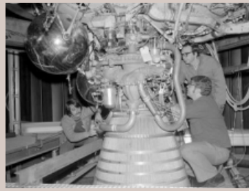
RL-10 in SPC No.1
