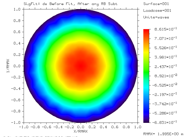
SFE from isothermal with defocus SFE = 977 nm PV; 288 nm RMS
