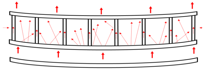
0.5 m thick closed-back ULE mirror Radial Gradient depends on view factor and side insulation.
