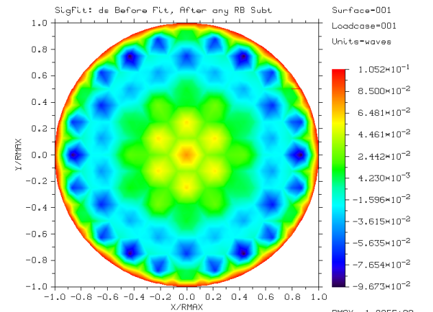
SFE from with defocus removed SFE = 128 nm PV; 24 nm RMS
