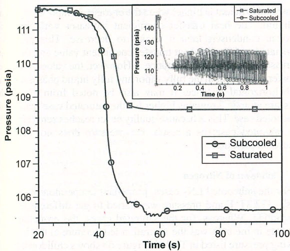
Fig. 9 Pressure-history comparison between subcooled and saturated LH 2 near the entrance of the pipe (node 2) for the driving pressure of 111.71 psia. Also shown in the inset is the initial pressure for the first 1 s.
