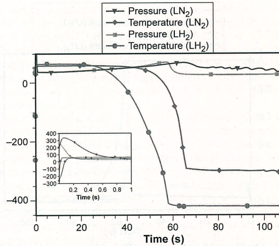
Fig. 10 Comparison of pressure and temperature between subcooled LH 2 and LN 2 at station 3 for the driving pressure of 86.7 psia.
