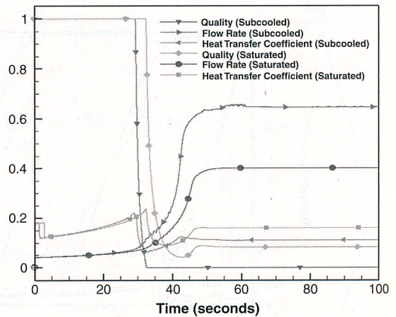
Fig. 8 Plots comparing a) quality and history between subcooled and saturated LH 2 near the entrance of the pipe (node 2) for the driving pressure of 111.71 psia and b) quality, heat transfer coefficient, and flow rate for subcooled and saturated cases for the same driving pressure at station 2.
