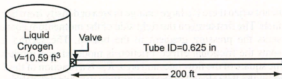
Fig. 1 Schematic of cryogenic line chilldown experimental setup.
