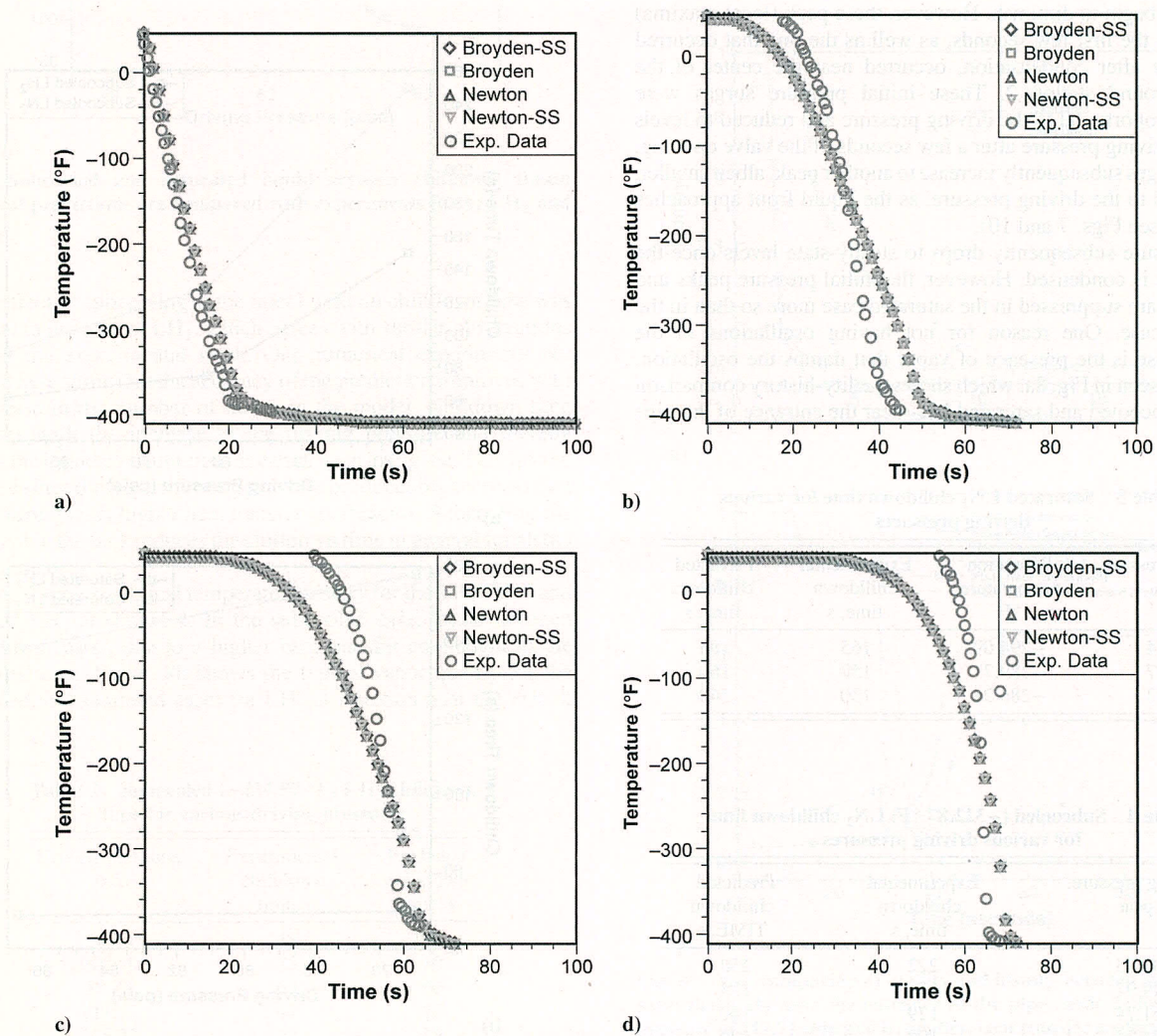
Fig. 13 Tube-wall temperature-history comparison of saturated LH 2 simulation with the four solvers for the driving pressure of 74.96 psia: a) station 1, b) station 2, c) station 3, and d) station 4.
