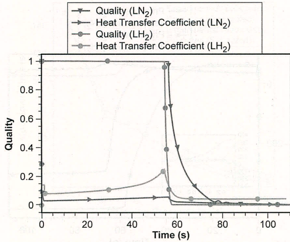
Fig. 12 Quality and heat transfer coefficient history of subcooled LH 2 and LN 2 for the driving pressure of 86.73 psia at station 3.
