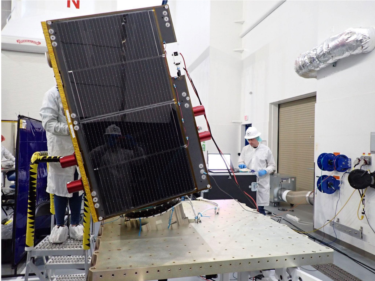
Figure 2.12: ESPA-Class satellite bus from Muon Space during integration at SpaceX facility for Transporter 8 rideshare mission. Credit: Muon Space via ExoLaunch and SpaceX.
