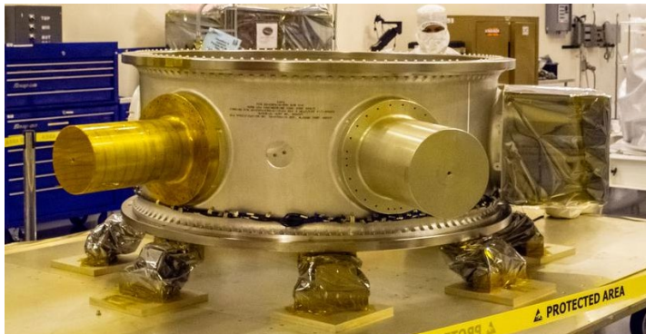
Figure 2.11: LandSat-9 ESPA Ring populated with payloads and mass ballasts. Credit: NASA/Randy Beaudoin.
