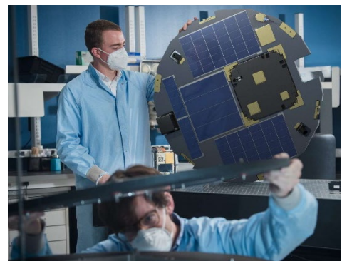
Figure 6.3: DiskSat structure. Courtesy of and reprinted by permission of The Aerospace Corporation.
