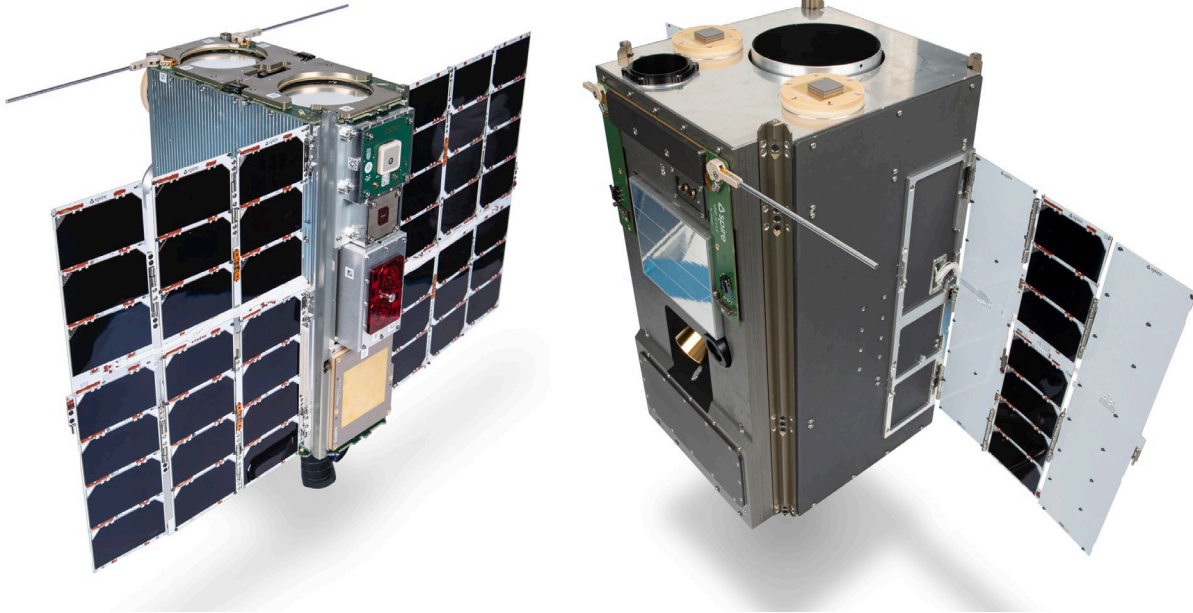
Figure 2.9: Examples of a 6U and 16U CubeSat. Credit: Spire Global.
