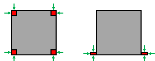
Figure 2.6: Rails vs. Tabs Restraint System Cross-Section.
