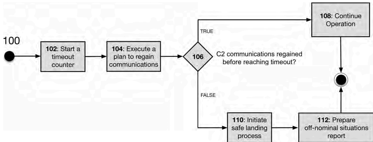
Figure 16: High-level Loss of C2 Communications Mitigations 6 .
