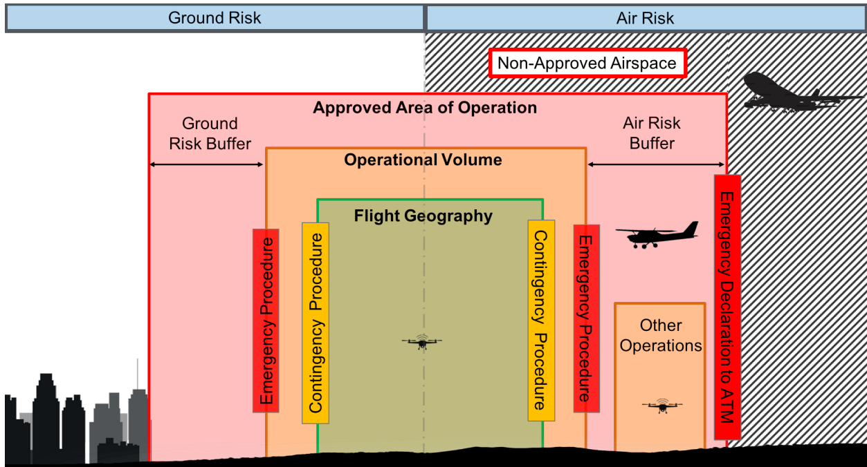
Figure 4: Airborne and ground risk posed to a UAS Operation.
