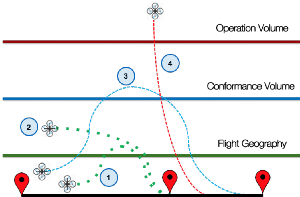
Figure 14: Scenarios of unmanned aircraft departing flight path and blundering through different operational boundaries.
