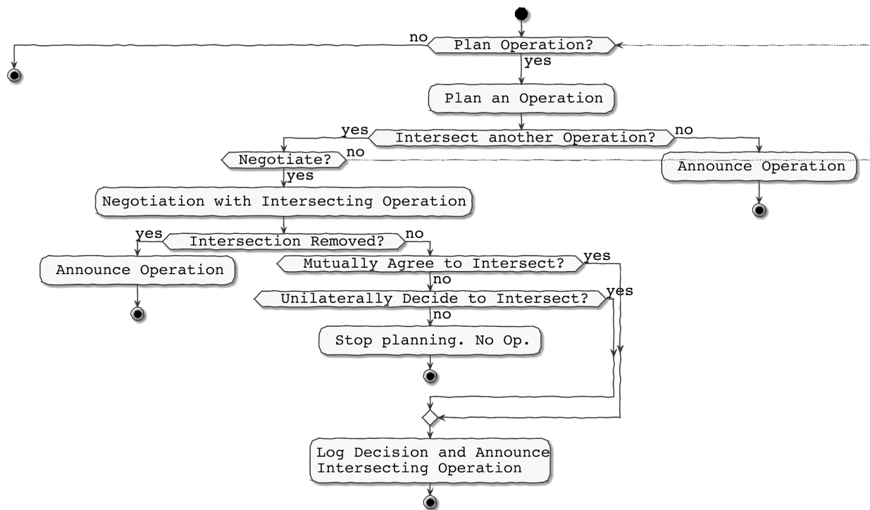
Figure 7: Strategic deconfliction process flow diagram.
