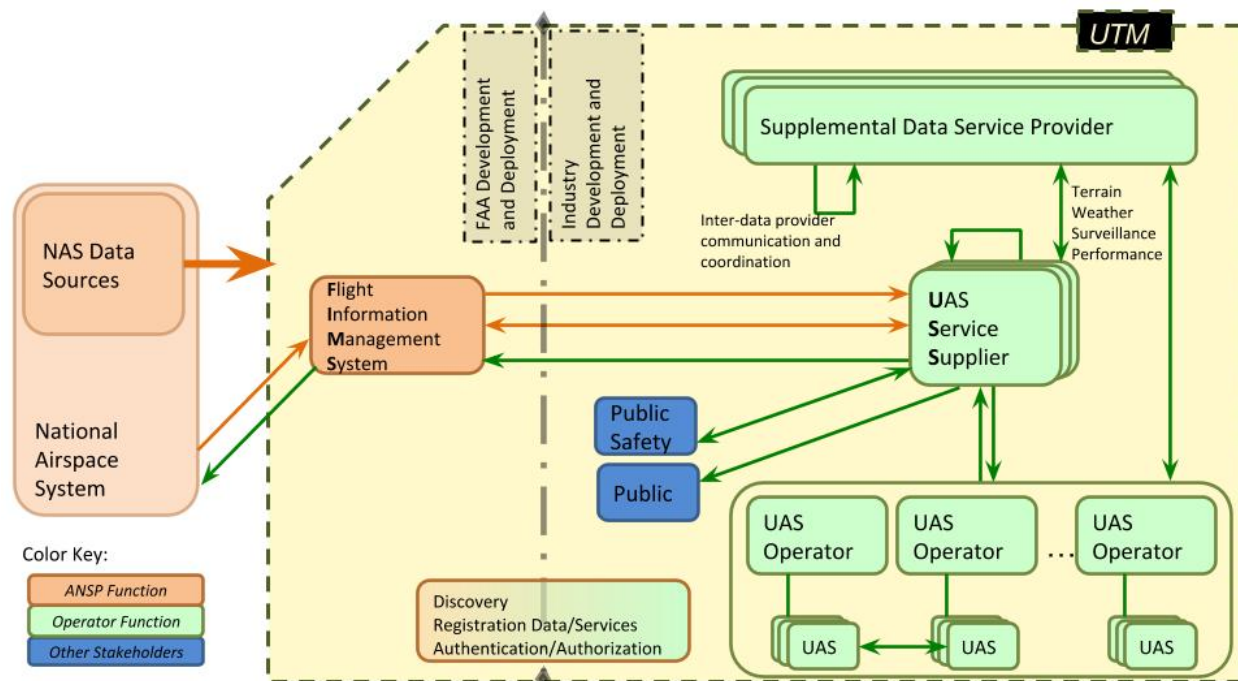
Figure 3: UAS Traffic Management System Architecture.
