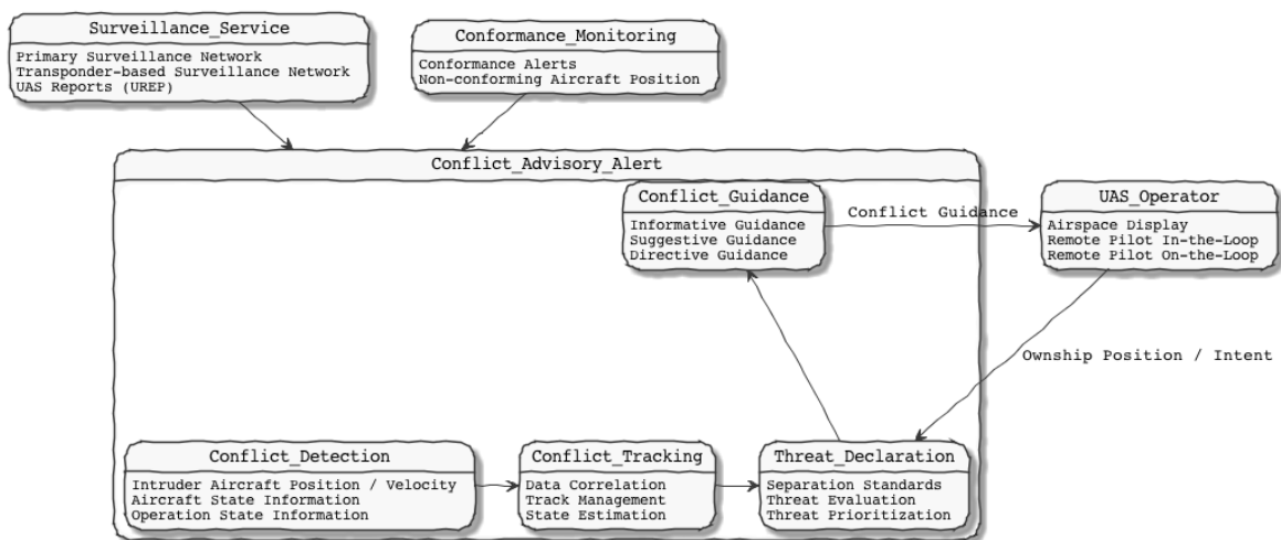
Figure 10: Functional diagram depicting the Conflict Advisory and Alerting Service.
