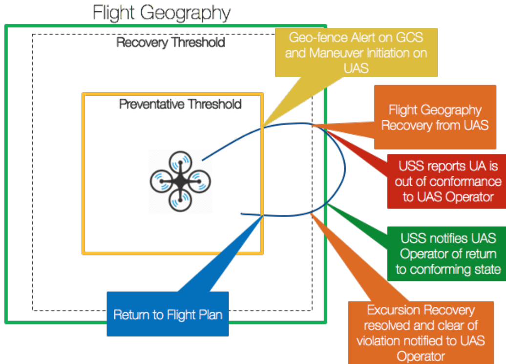
Figure 12: Relationship between Flight Containment Capability and Conformance Monitoring Services.
