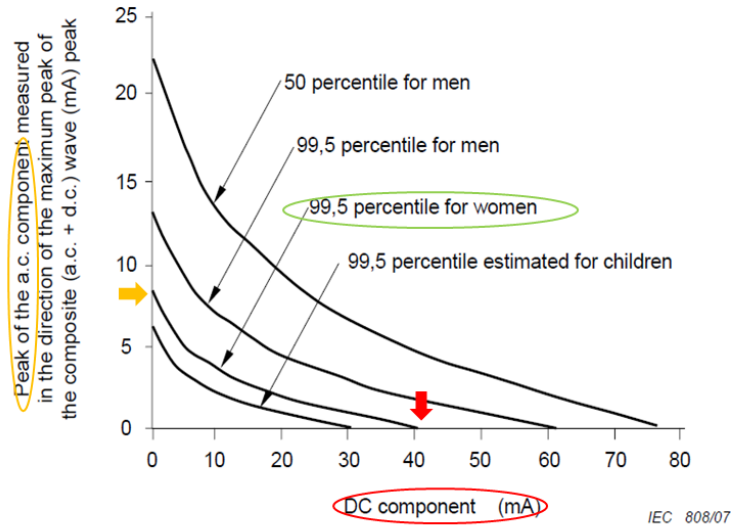
Figure 7 – Let-go thresholds for men, women and children
