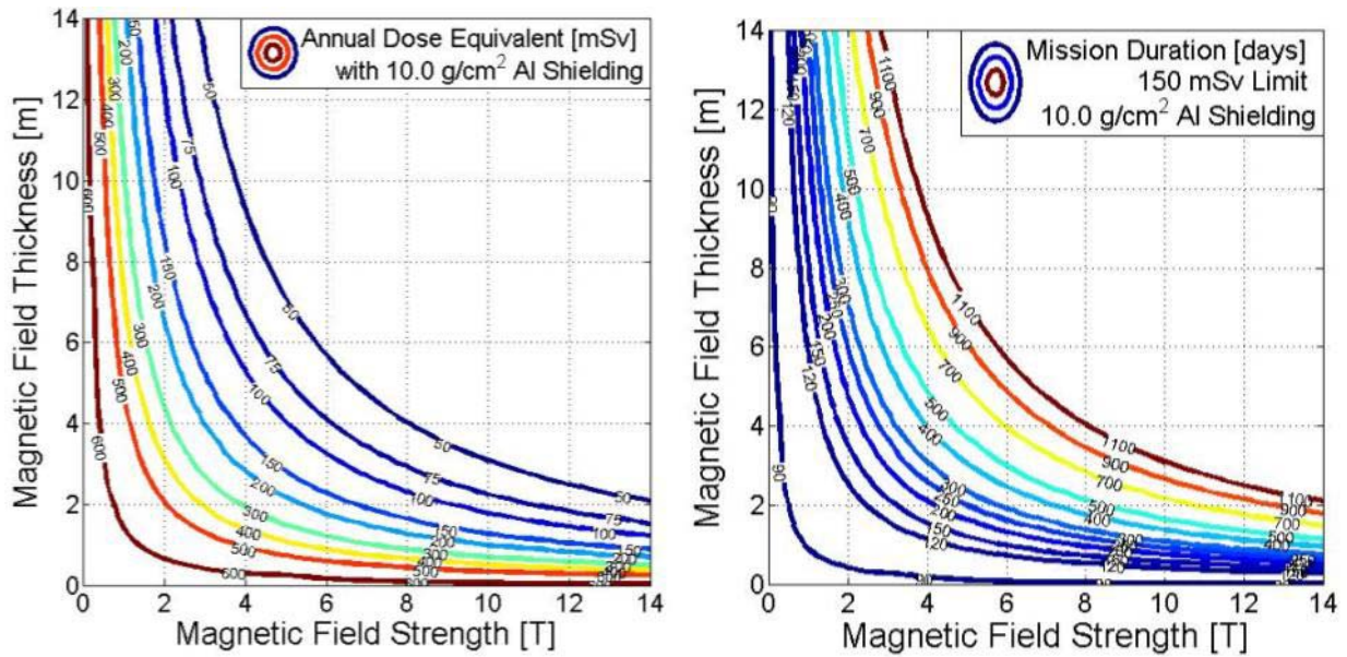
Figure A.3 Infinite Cylinder Model with 10.0 g/cm 2 Shielding ( r_i = 4\text{m} ) a) Annual Dose Equivalent, b) Maximum Mission Duration to 150 mSv Limit
