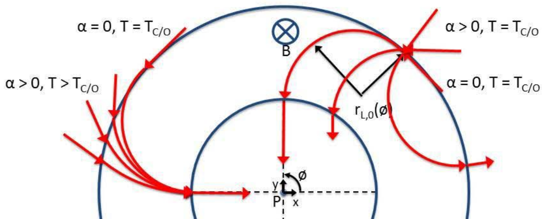
Figure 8.3. Flux Through Point P Inside Quasi-Spherical Model
