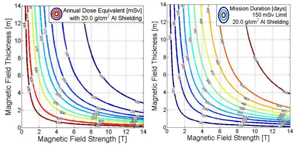
Figure A.6 Infinite Cylinder Model with 20.0 g/cm 2 Al Shielding ( r_i = 4\text{m} ) a) Annual Dose Equivalent, b) Maximum Mission Duration to 150 mSv Limit
