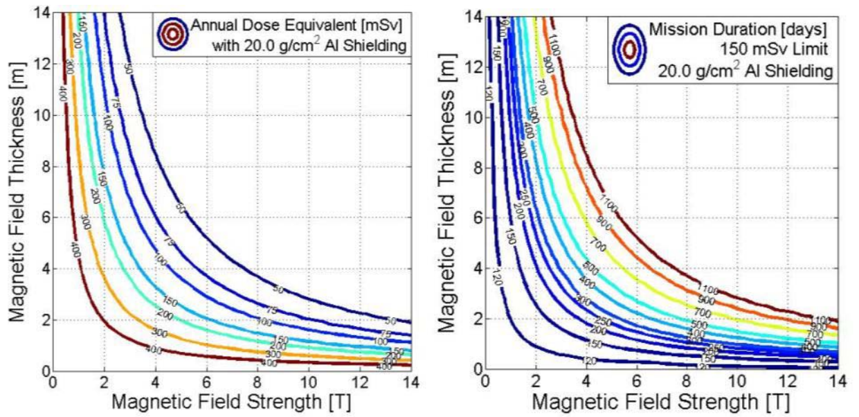
Figure A.4 Infinite Cylinder Model with 20.0 g/cm 2 Shielding ( r_i = 4\text{m} ) a) Annual Dose Equivalent, b) Maximum Mission Duration to 150 mSv Limit
