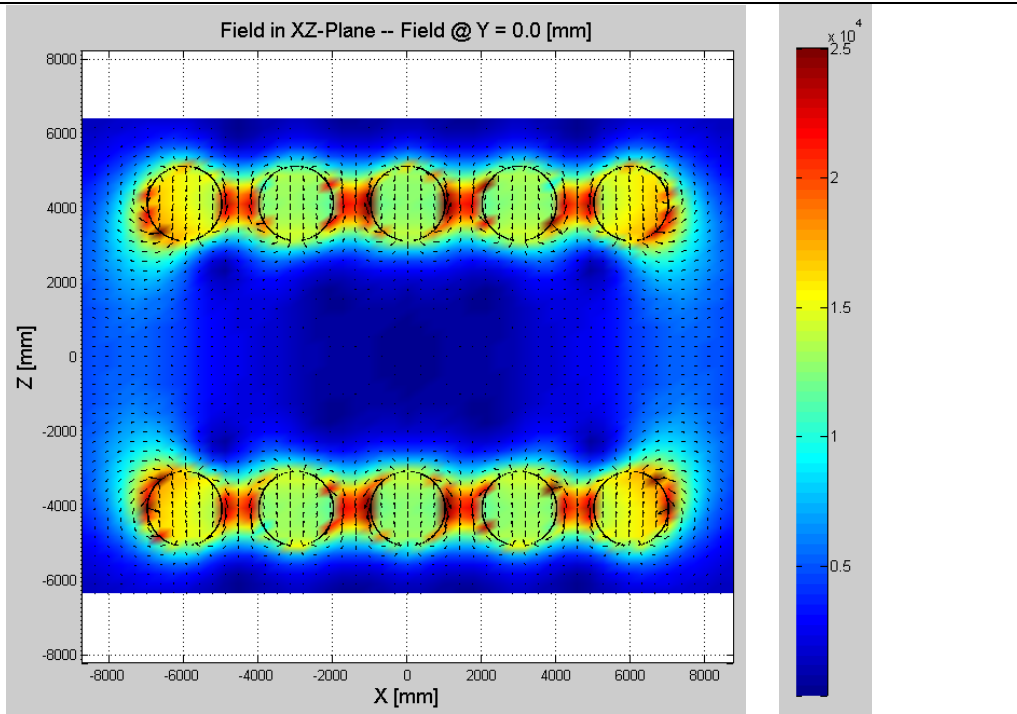
Figure 2.32: Flux density distribution of 5-toroid array with 1000-mm gap between adjacent coils.
