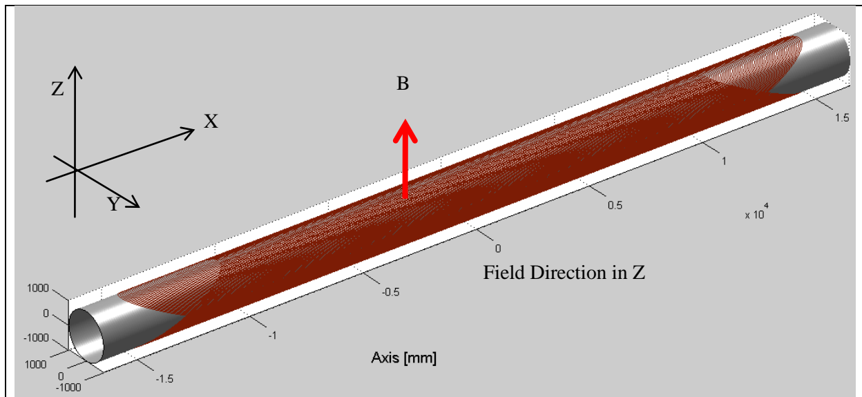
Figure 2.43. DH coil consisting of two concentric layers. The windings are oriented to generate a field perpendicular to the coil axis in the direction of the Z-axis. The axial field components are cancelled.
