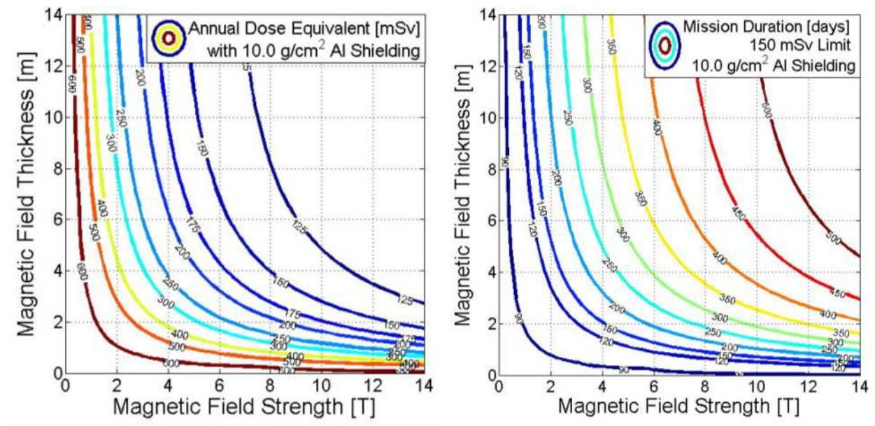
Figure A.5 Infinite Cylinder Model with 10.0 g/cm 2 Al Shielding ( r_i = 4\text{m} ) a) Annual Dose Equivalent, b) Maximum Mission Duration to 150 mSv Limit
