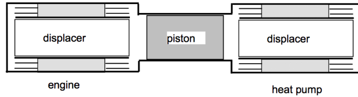
Figure 5.9—Duplex Sketch
