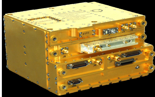
Figure 5.4—Image of Representative SDST communications hardware.
