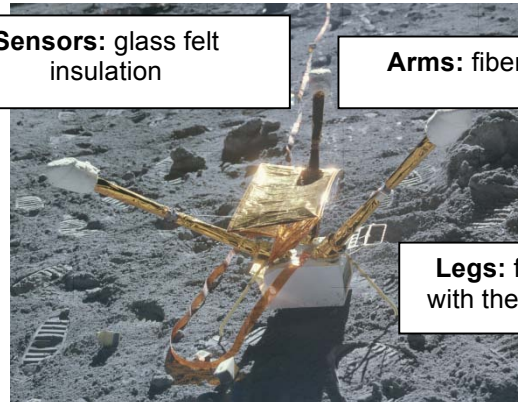
Figure B4 – Lunar Surface Magnetometer
