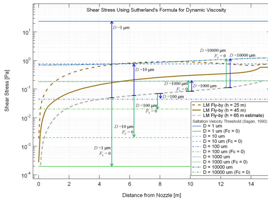
Figure 11: Shear stress generated by a rocket exhaust plume and shear stress levels required to mobilize various sizes of lunar soil particles.
