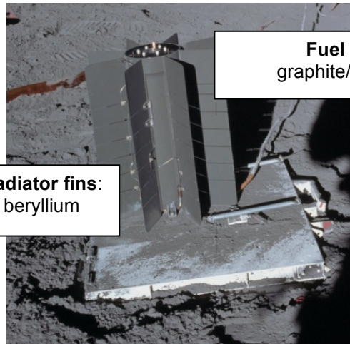
Figure B2 – RTG
