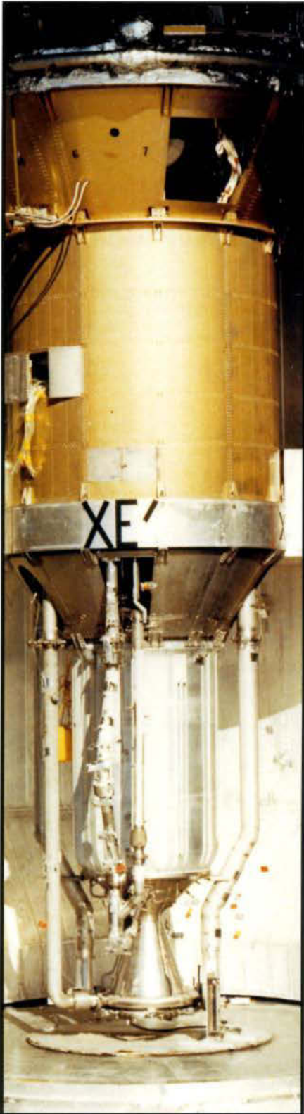
Figure 3: NERVA Engine
