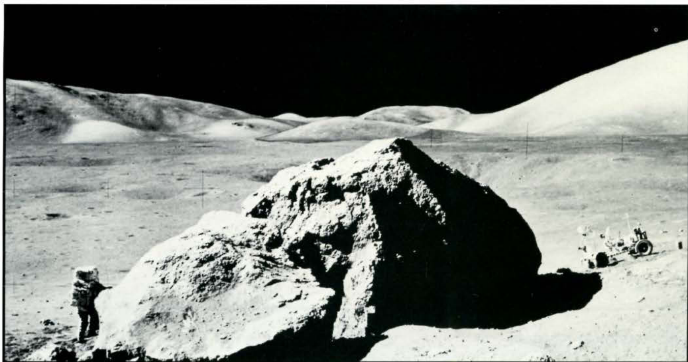
Lunar Boulder Near Taurus Littrow, Apollo XVII
