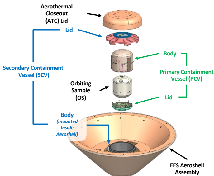
The conceptual design of the Earth Entry System (EES) for Mars Sample Return includes redundant layers of containment for the samples.
