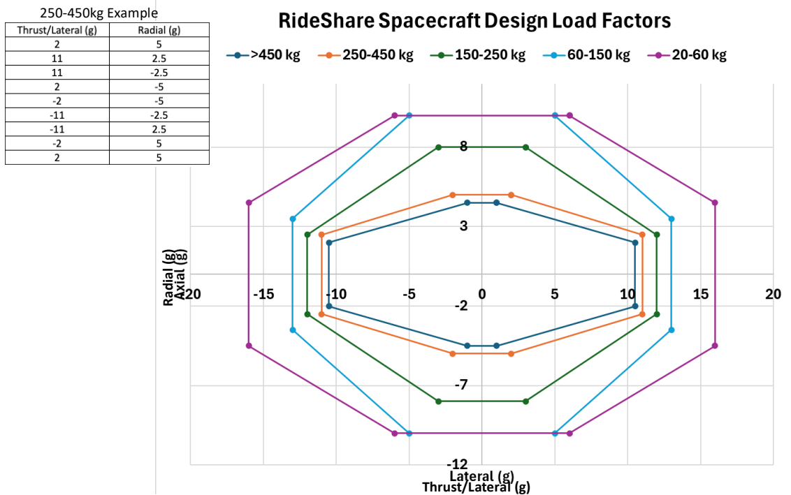
Figure 6.2 Side Mounted Design Load Factors
