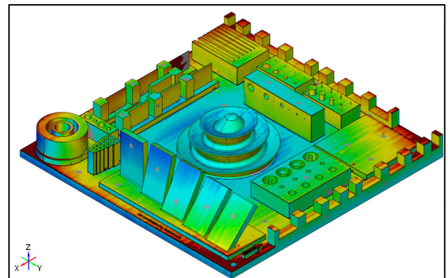
Structured Light Scanning of hardware
