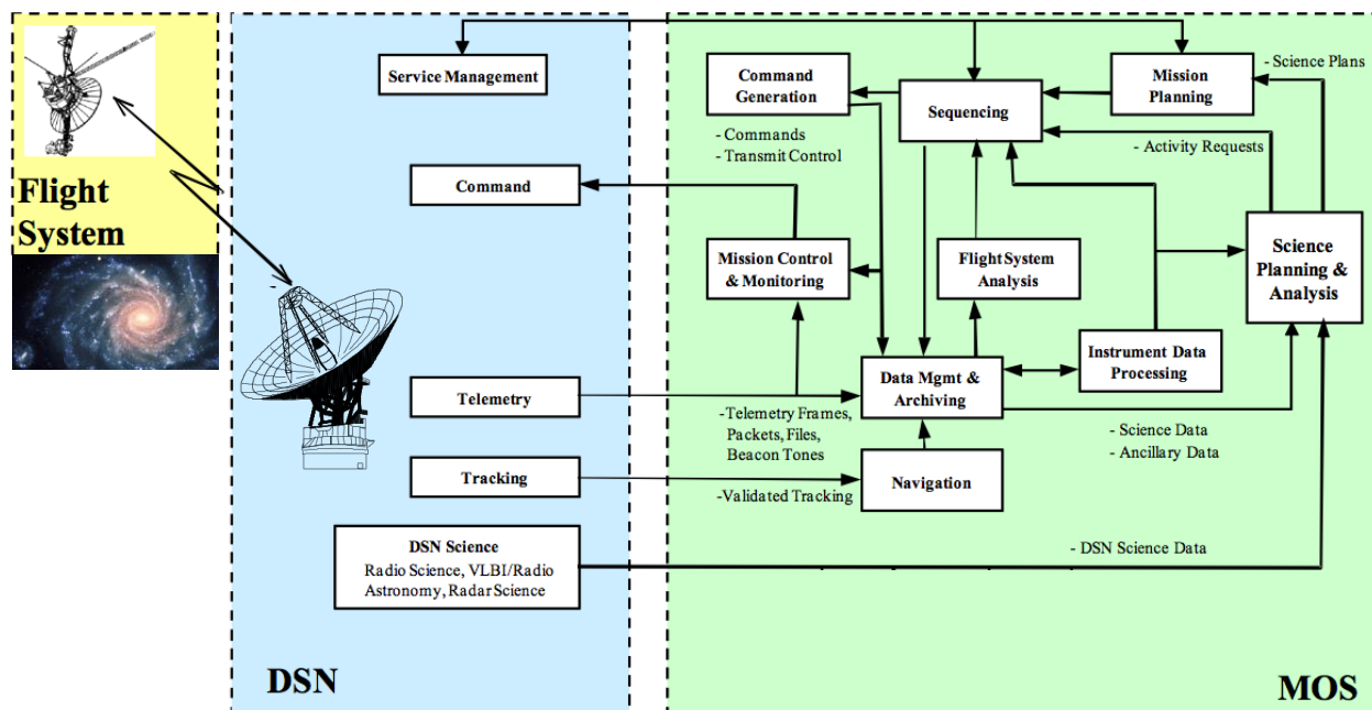
Figure 2-1. Mission Operations Context – Functional View
