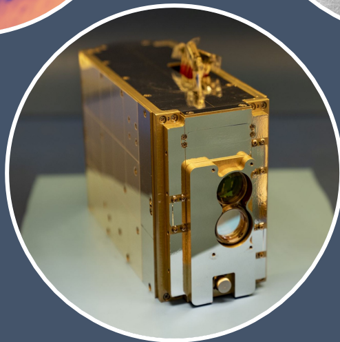
PTD-4 / TBIRD 200 Gbps Optical Link
