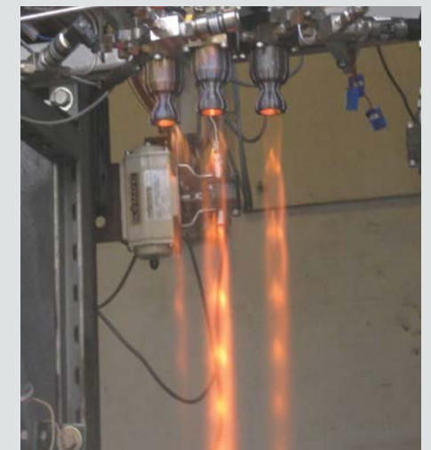
Testing of low-cost engines for nano-launcher upper stage.
