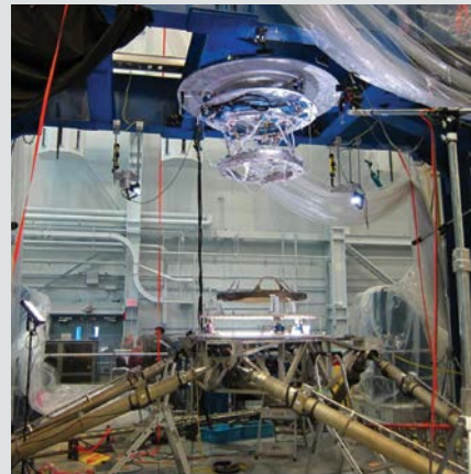
Engineering model of the LIDS being tested in the JSC 6 degrees-of-freedom test stand.
