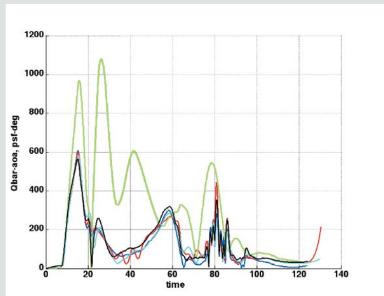
Comparisons between five simulations for an early Ares I-X concept.
