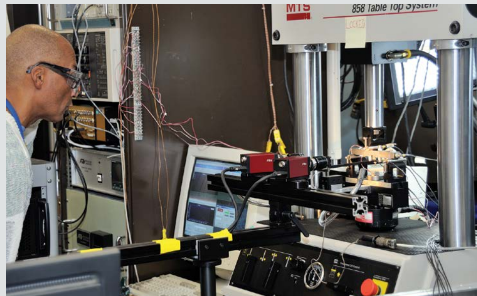
Stewart Walker of the LaRC Advanced Materials and Processing Branch is shown conducting a 3-point strength test on a ceramic C/C-SiC composition material. The specimen is highly instrumented to understand performance.
