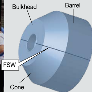
An aluminum alloy 2219 spin-formed MPCV CM-like bulkhead containing a single friction stir weld (FSW) region.
