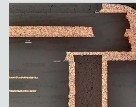
Partial coupon microsection illustrates measurement of internal annular ring and solid copper microvia structures at upper right edge.
