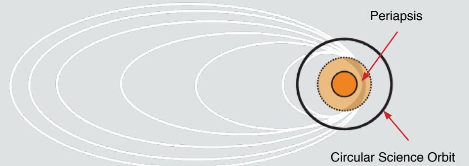
Aerobraking is used to reduce the propellant required to deliver a spacecraft into its desired final orbit around a target planet or moon that has an atmosphere.
