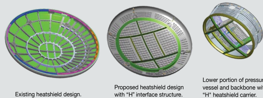
Existing heatshield design.
