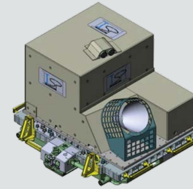
NOFBX flight experiment solid model rendering.
