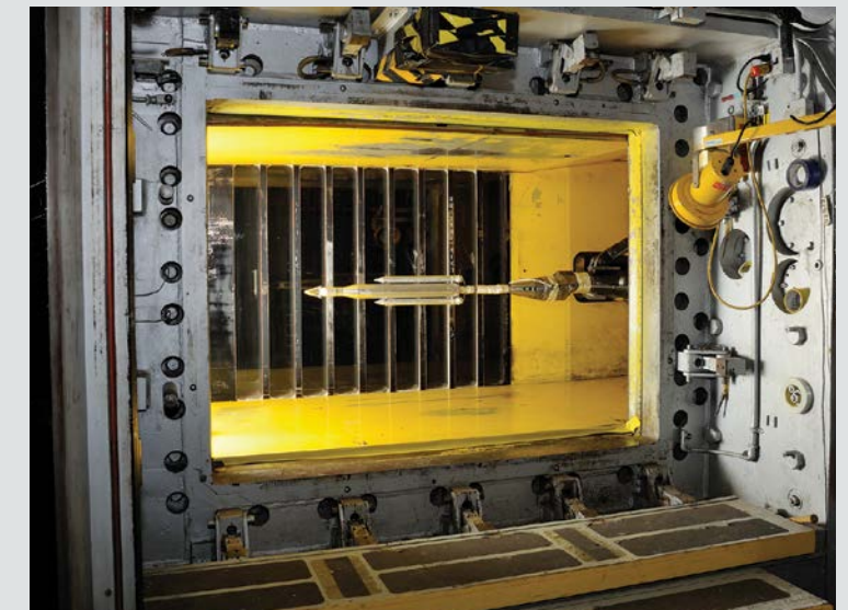
Test section of LaRC Unitary Wind Tunnel with the HL-20 lifting body spacecraft on an SLS model.
