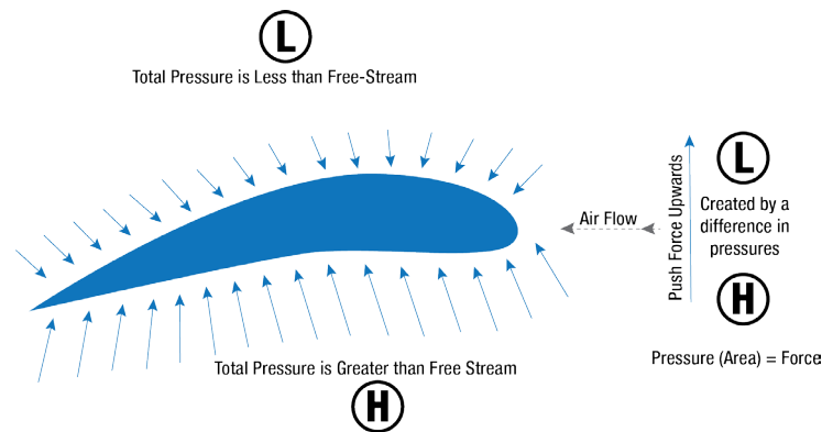
Fig. 4 Lift
