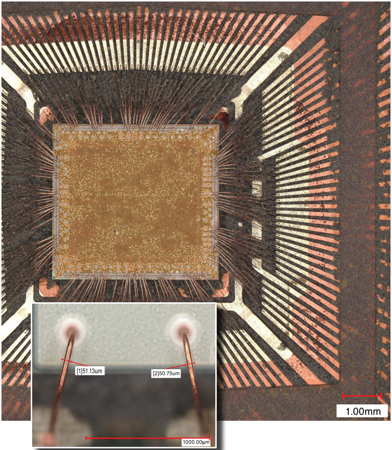
Example of copper wire bonds.
