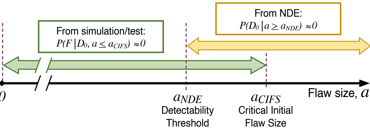
Figure 1. A probabilistic interpretation of damage tolerance
