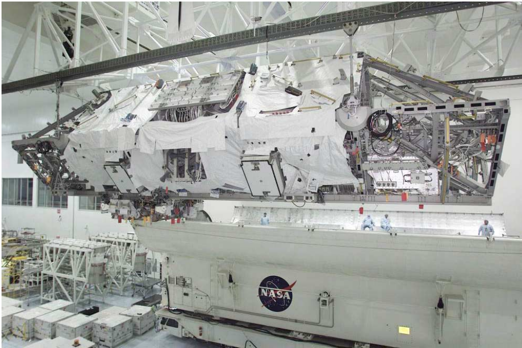
The S0 truss is loaded into its transport canister at Kennedy Space Center.
